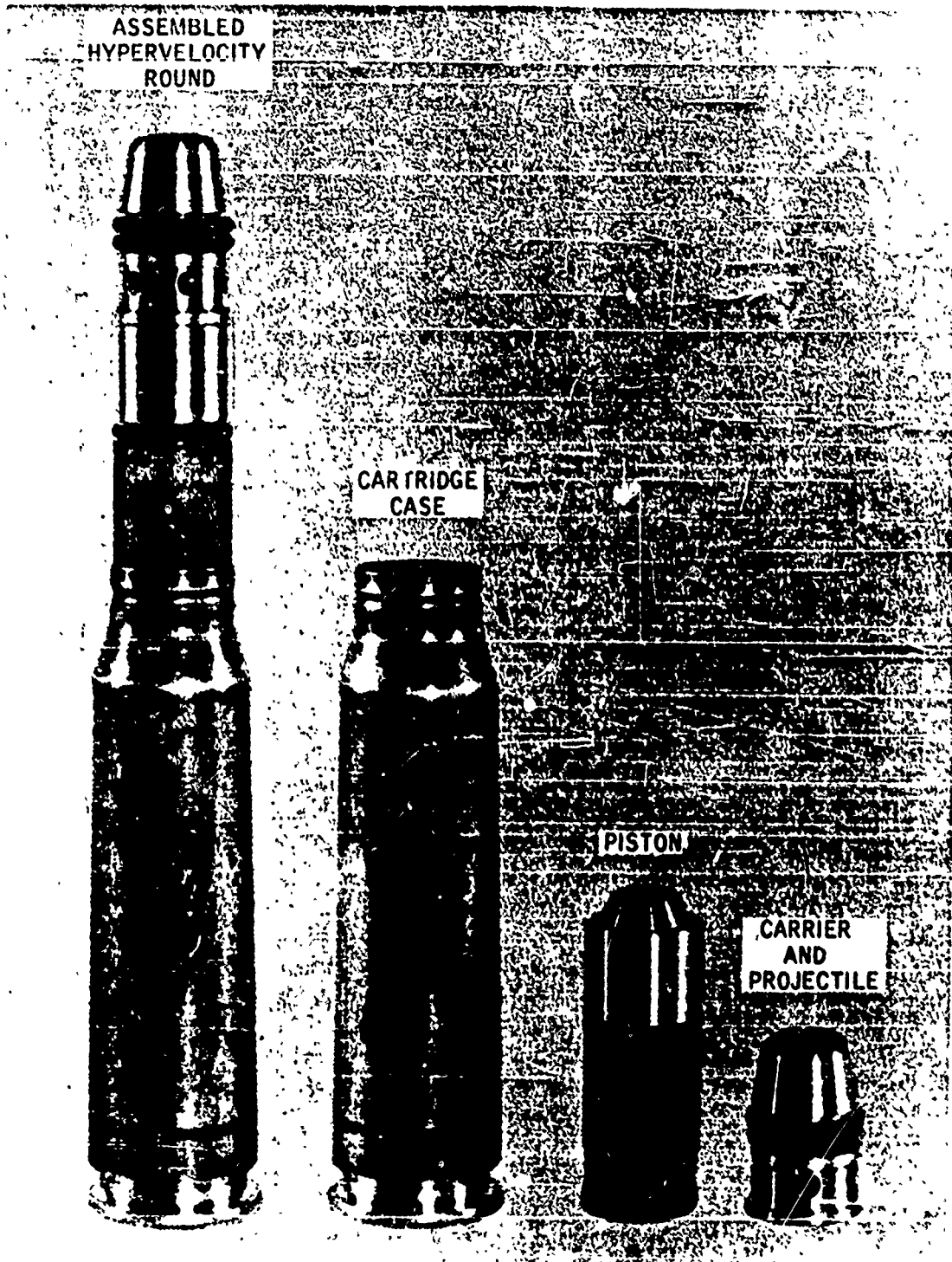
Figure 4-11. Hypervelocity Round and Components (Present Configuration)
