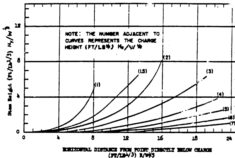
FIGURE 2-3 MACH STEM HEIGHT VS HORIZONTAL DISTANCE FROM CHARGE FOR VARIOUS CHARGE HEIGHTS FOR TEST
