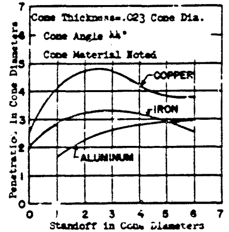
FIGURE 4-18 PENETRATION VS STANDOFF AGAINST MILD STEEL TARGETS
