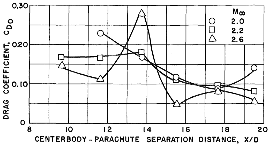
Fig. 25 Variation of Drag Coefficient with Centerbody-Parachute Separation Distance
