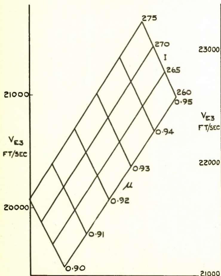
(c) PAYLOAD WEIGHT 110 LB. FIRST STAGE T = 21,600 LB. WT. I = 213, W_P = 11600 LB. W_E = 1380 LB.
