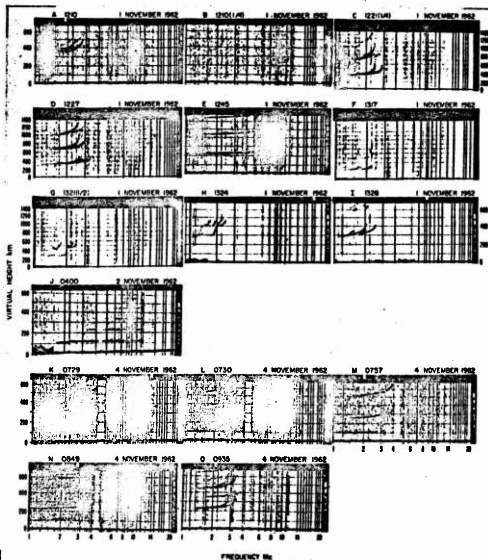
Figure 67 King Fish, Tight Rops, Midway, selected ionograms.
