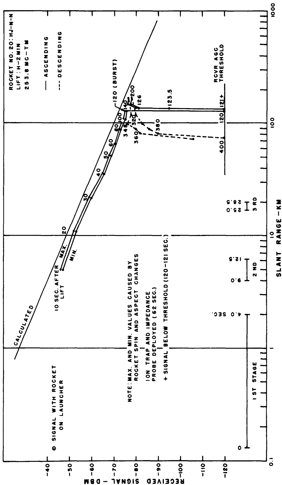
Figure C.221 Received signal strength versus slant range for VHF telemetry, Rocket 20, King Fish.
