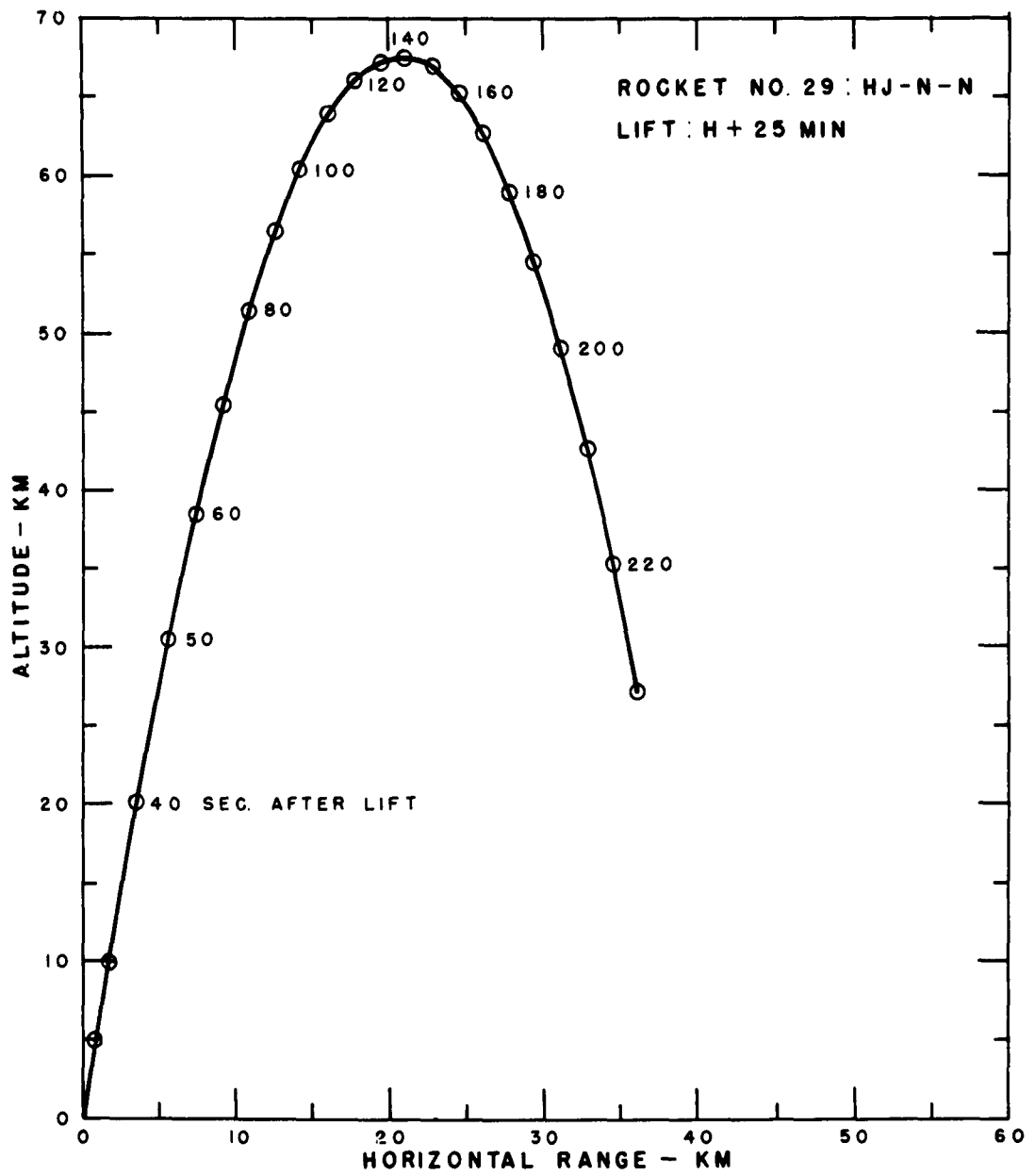
Figure B.27 Trajectory for Rocket 29, King Fish.
