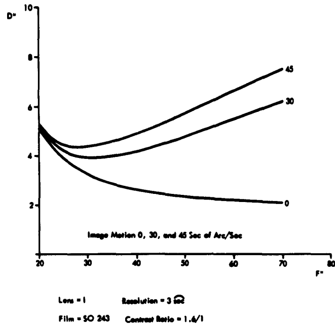
Figure 3-20. Aperture (D) vs Focal Length (F) for Resolution of 3 Sec, Lens I
