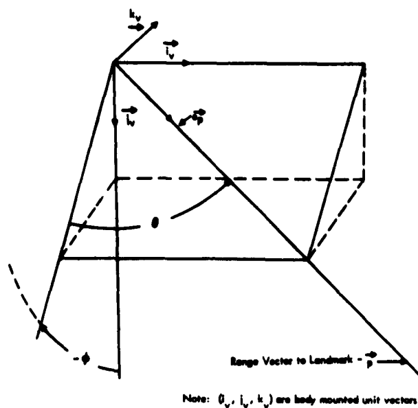
Figure 3-67. Pitch and Roll Angles of the Line of Sight
