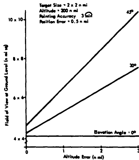
Figure 3-3 Field of View Necessary to Ensure Target is Included
