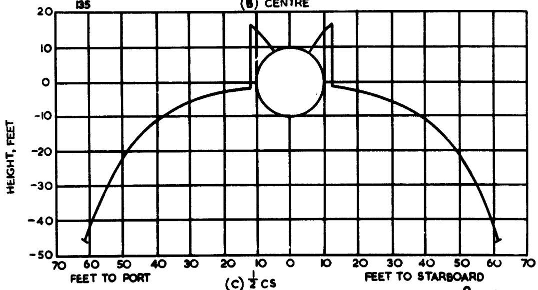
FIG. 9 FIRING LOCI FOR SUBMARINE HEADING SOUTH ( 70^\circ DIP) (REVERSE BOW AND STERN FOR NORTH HEADING)
