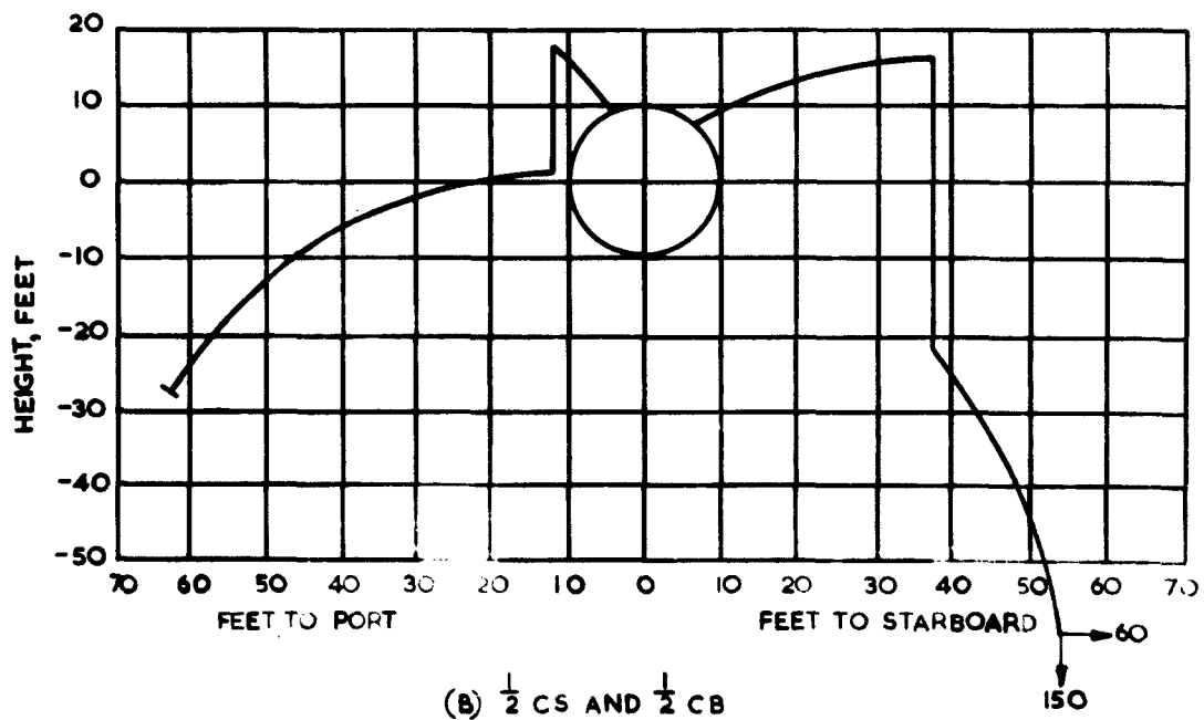
FIG. 10 FIRING LOCI FOR SUBMARINE HEADING EAST ( 70^\circ DIP) (REVERSE PORT AND STARBOARD FOR WEST HEADING)
