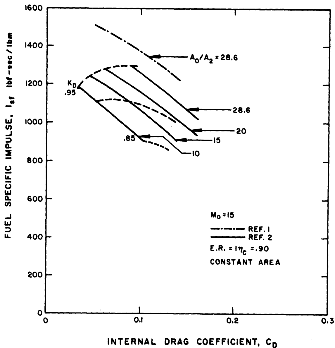
FIGURE 3.10 EFFECT OF INLET INTERNAL DRAG COEFFICIENT ON FUEL SPECIFIC IMPULSE
