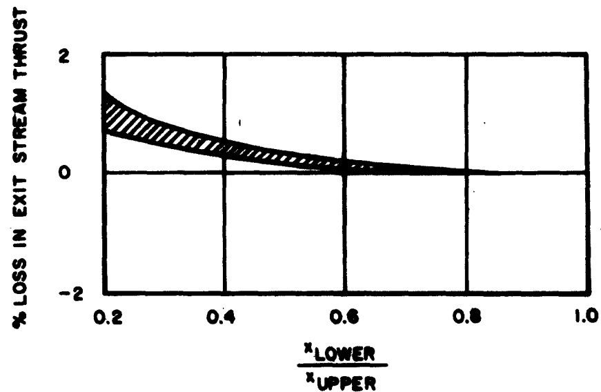
FIGURE 5.18 LOSS IN EXIT STREAM THRUST DUE TO LOWER WALL TRUNCATION
