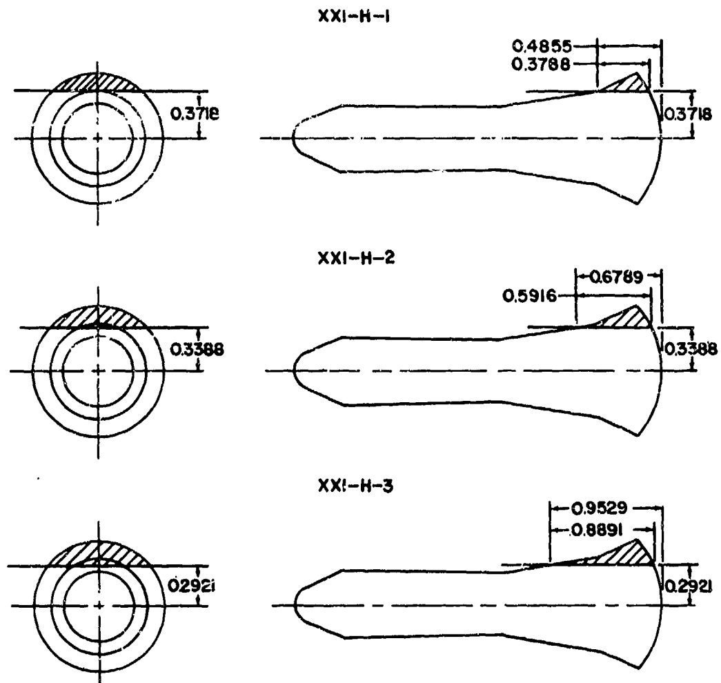
NOTE: ALL MATERIAL IN CROSS-HATCHED AREA HAS BEEN REMOVED FIG. 2 MARK 3 CONFIGURATIONS WITH FLARE MODIFICATIONS, XXI-H-1, 2, AND 3
