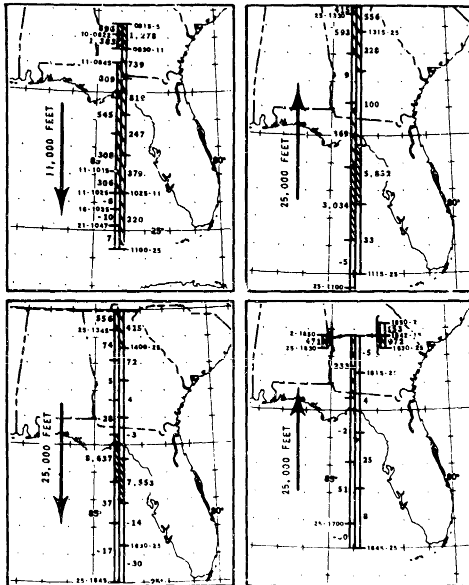
Fig. 3.37 LARK WILLIAM 11, 7 November 1951
