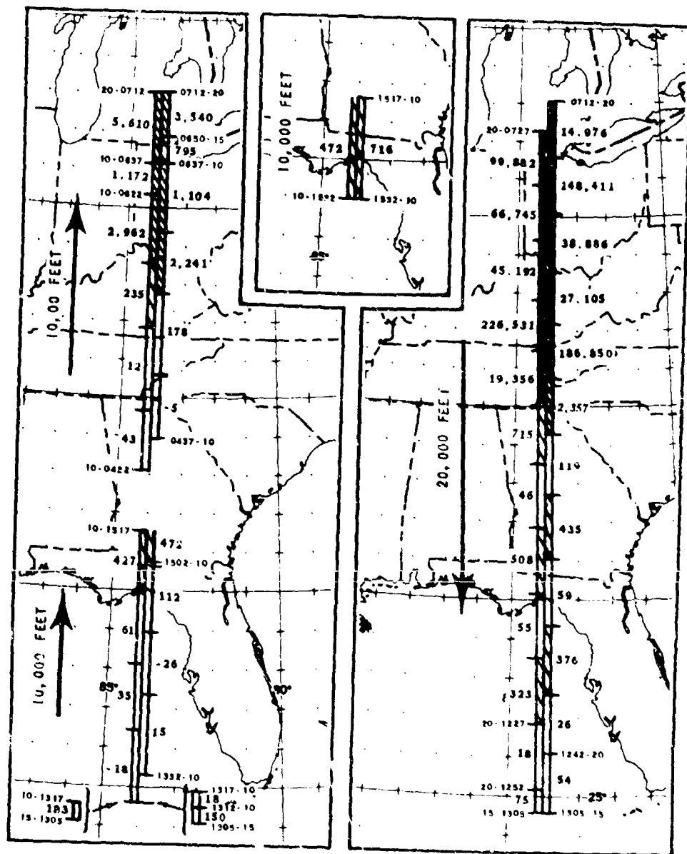
FIG. 3.18 LARK WILLIAM 4, 1 November 1951
