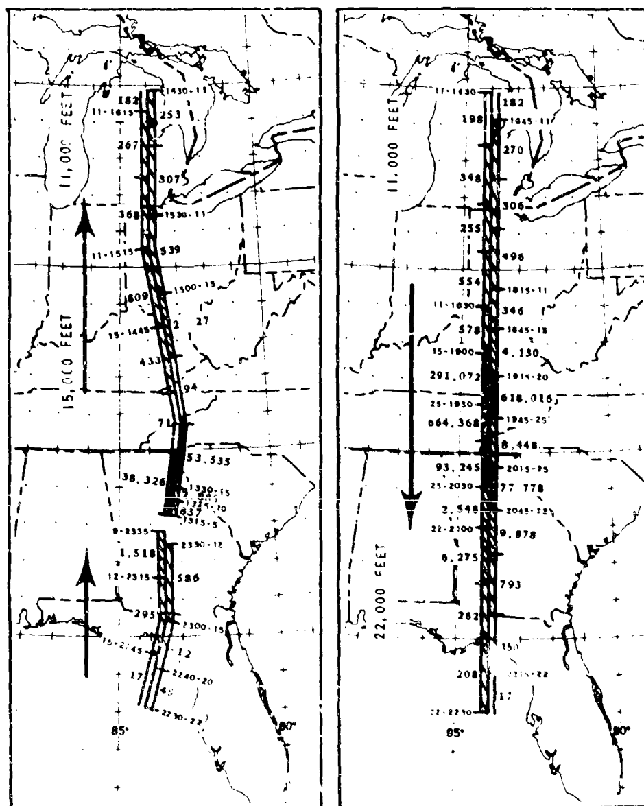
Fig. 3.25 LARK WILLIAM 6, 2 November 1951
