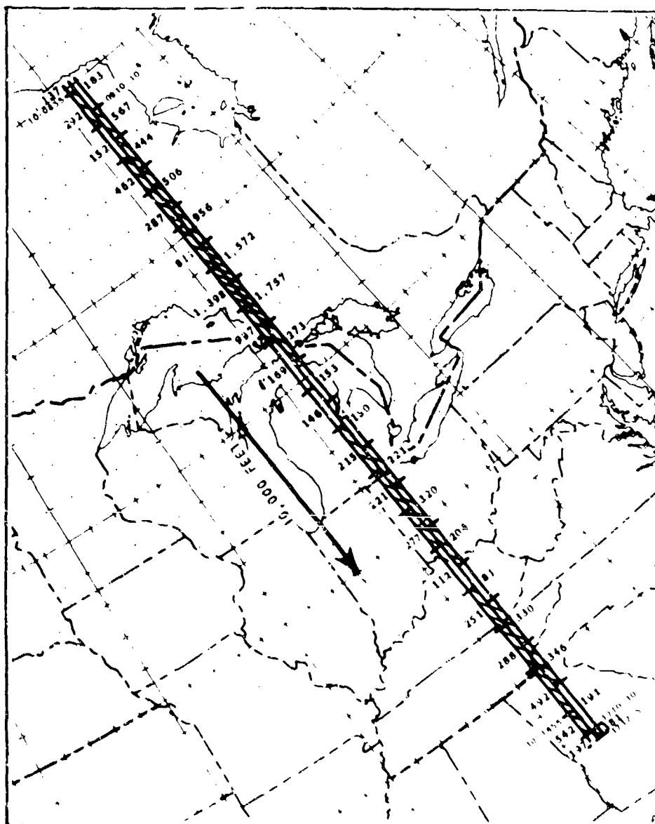
Fig. 3.58 LARK WILLIAM 21, 22 November 1951 - Southbound
