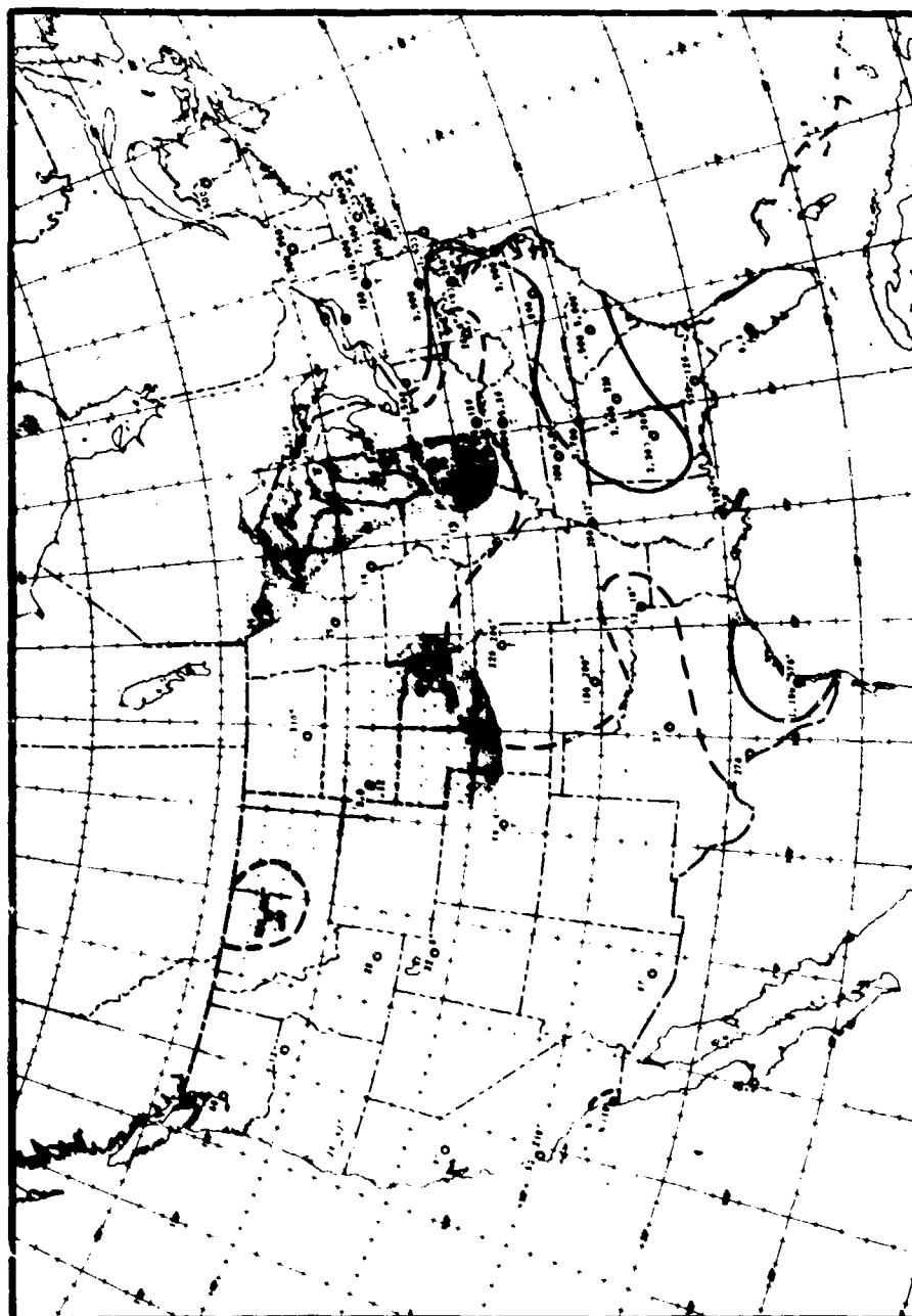
Fig. A.17 Surface Distribution of Radiocative Debris and Concurrent Precipitation, 4 November 1951
