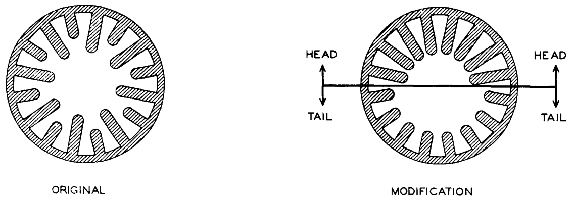
Fig. 1 Original grain design and tapered modification.
