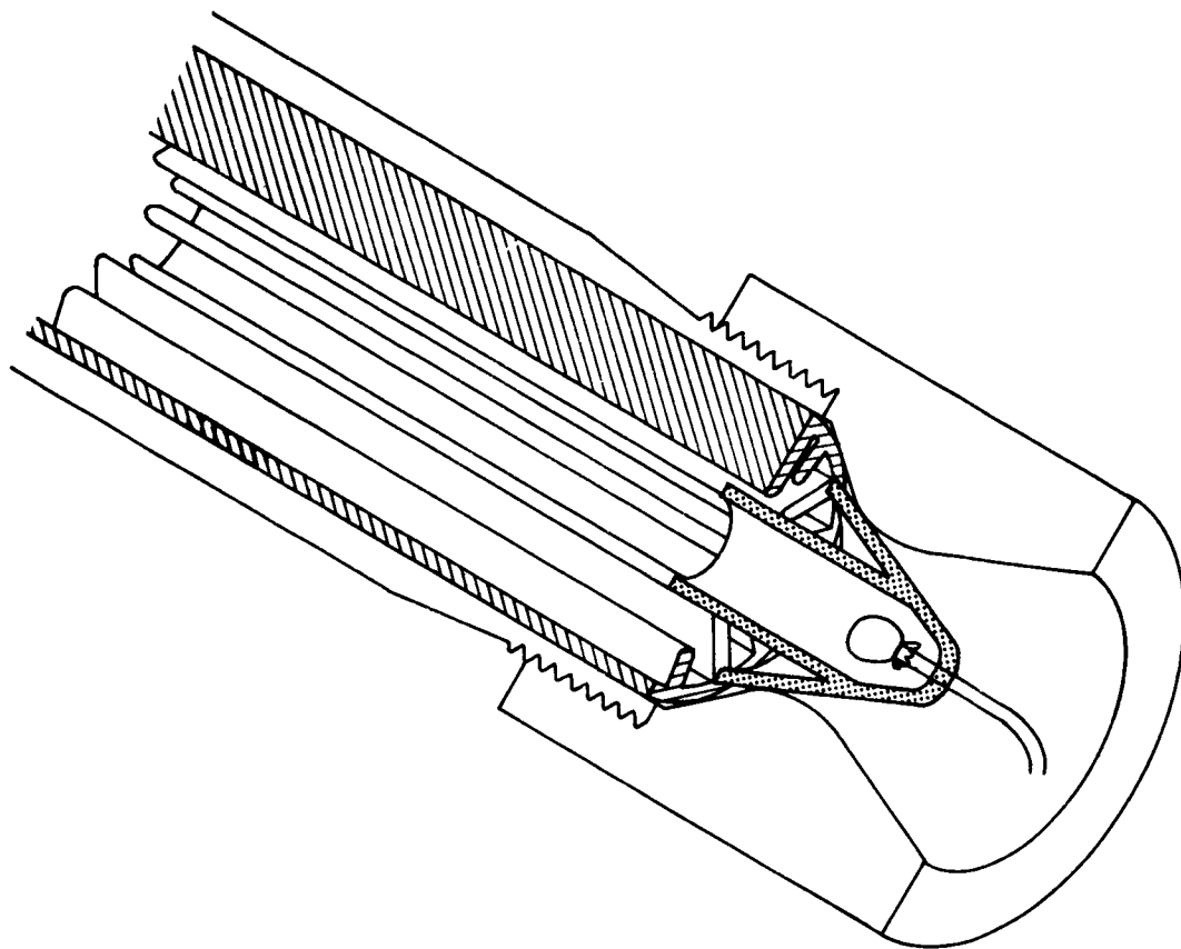
Fig. 2 Nozzle-closure igniter system.
