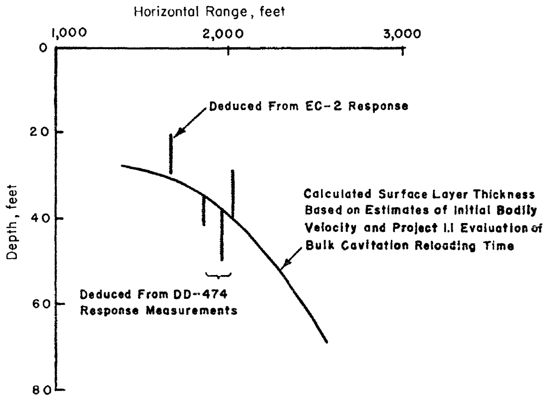
Figure 6.20 Surface layer thickness versus horizontal range, Shot Umbrella.
