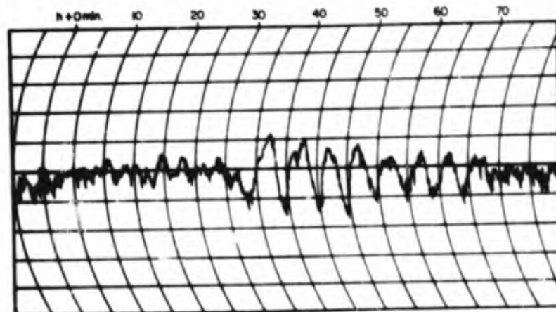
Figure 11 Reproduction of actual record obtained at Eniwetok for Shot Tewa, Operation Redwing. Shot time indicated as h + 0 minutes.
