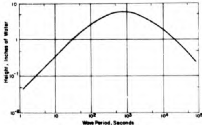
Figure 2 Amplitude response curve for the hydraulic filter. Curve shows output pressure in inches of water as a function of wave period for a 10-inch sine-wave input.
