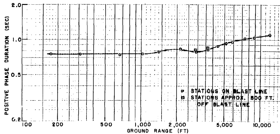
Fig. 2.43 Positive Phase Duration, t_h , Ground Level, TUMBLER 3
