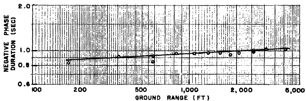
Fig. 2.24 Negative Phase Duration, t_8 , Ground Level, TUMBLER 1
