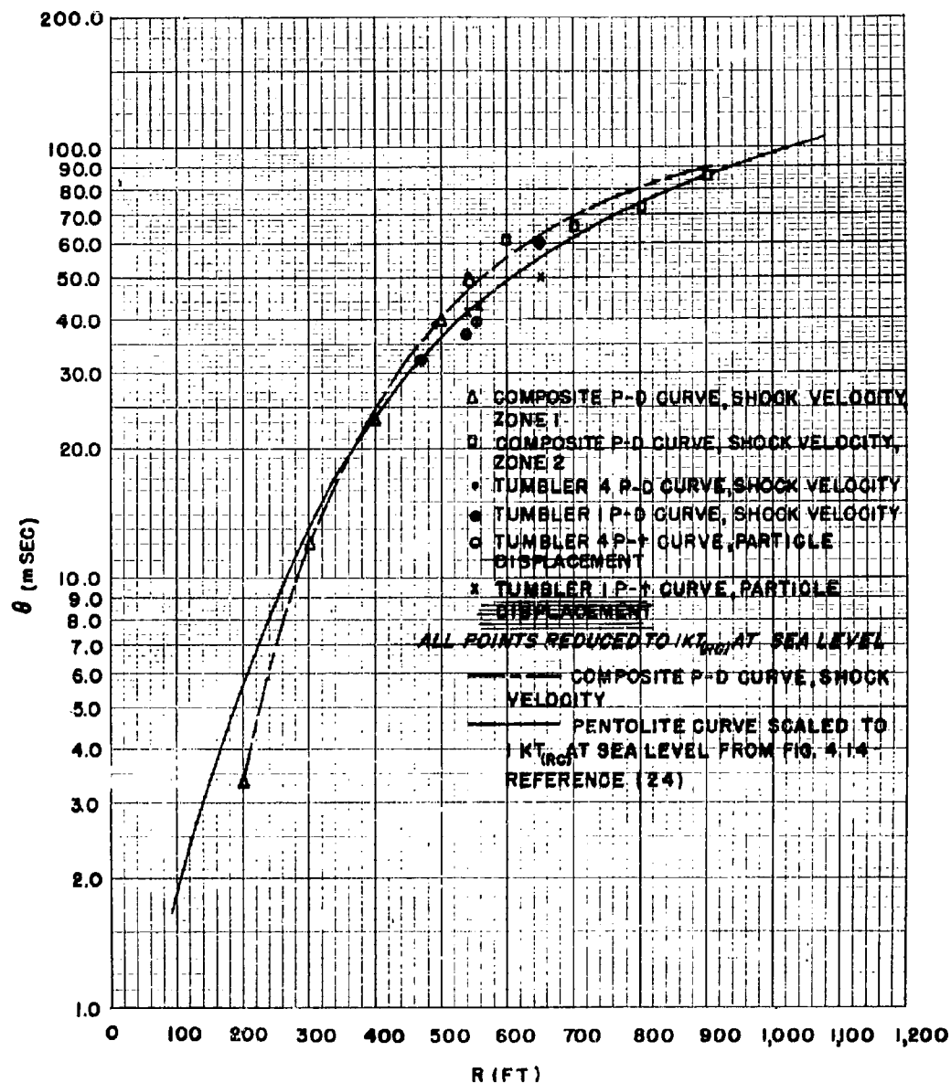
Fig. 4.14 \theta vs Distance Reduced to 1 KT (RC) at Sea Level (Free Air)
