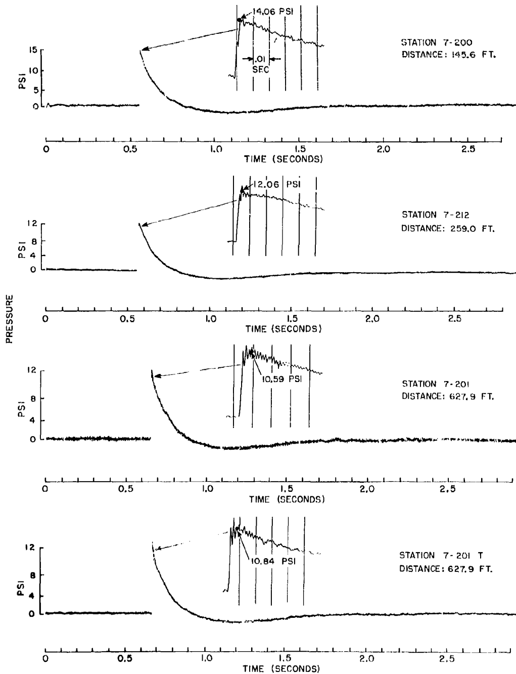
Fig. 2.26 Records, TUMBLER 2, Stations 7-200 through 7-201T
