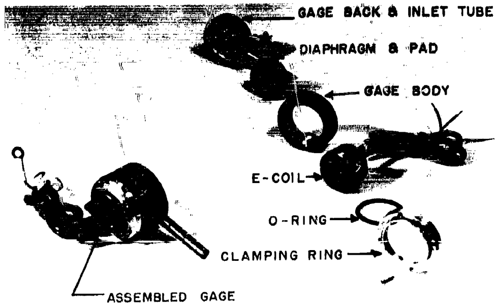
Fig. 2.3 Bendix Gage and Its Construction
