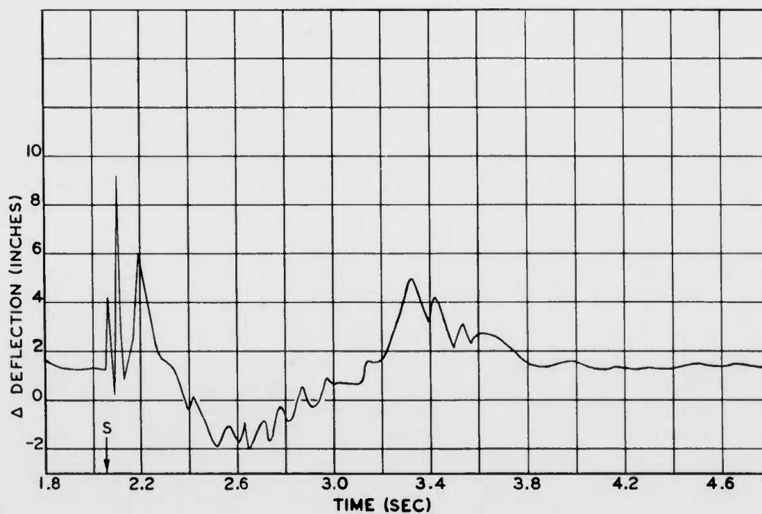
Figure 5.14 Wing Deflection, Station 213 Left, Drone 3
