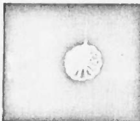
d. Configuration H-8, 9.6-percent Porosity, M_\infty = 2.6
