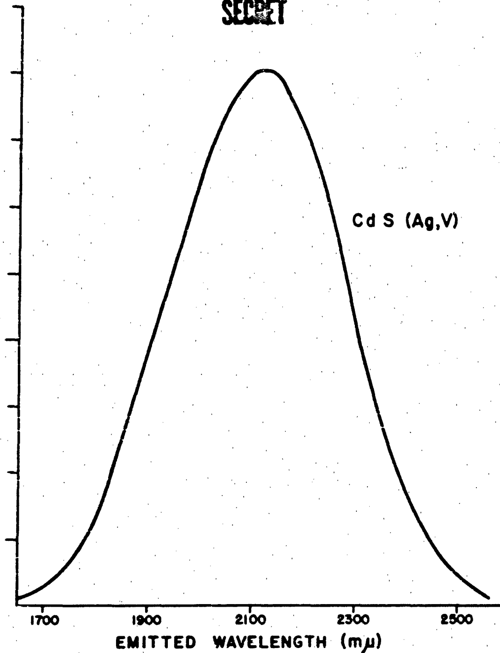
Figure 26 - Fluorescence Spectra of CdS (Ag,V)
