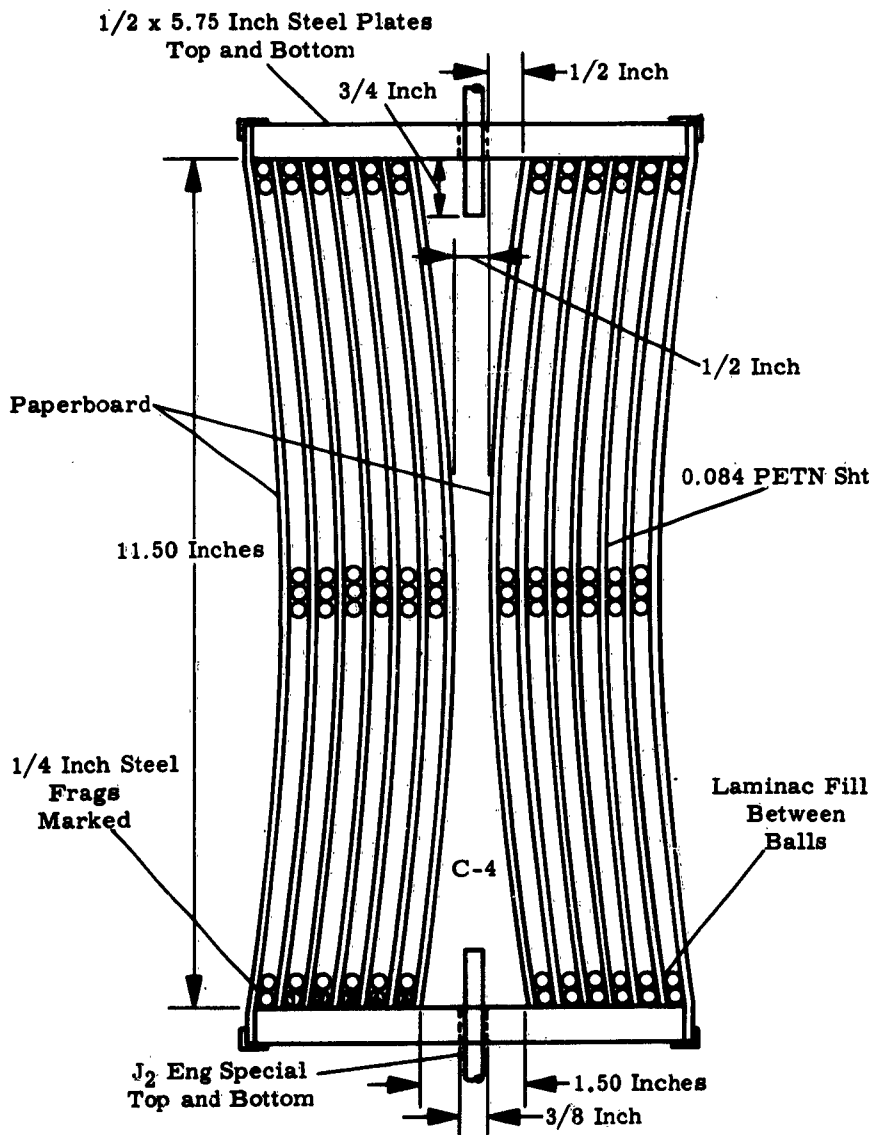
Figure 64. Test Model Design, Round RE-2
