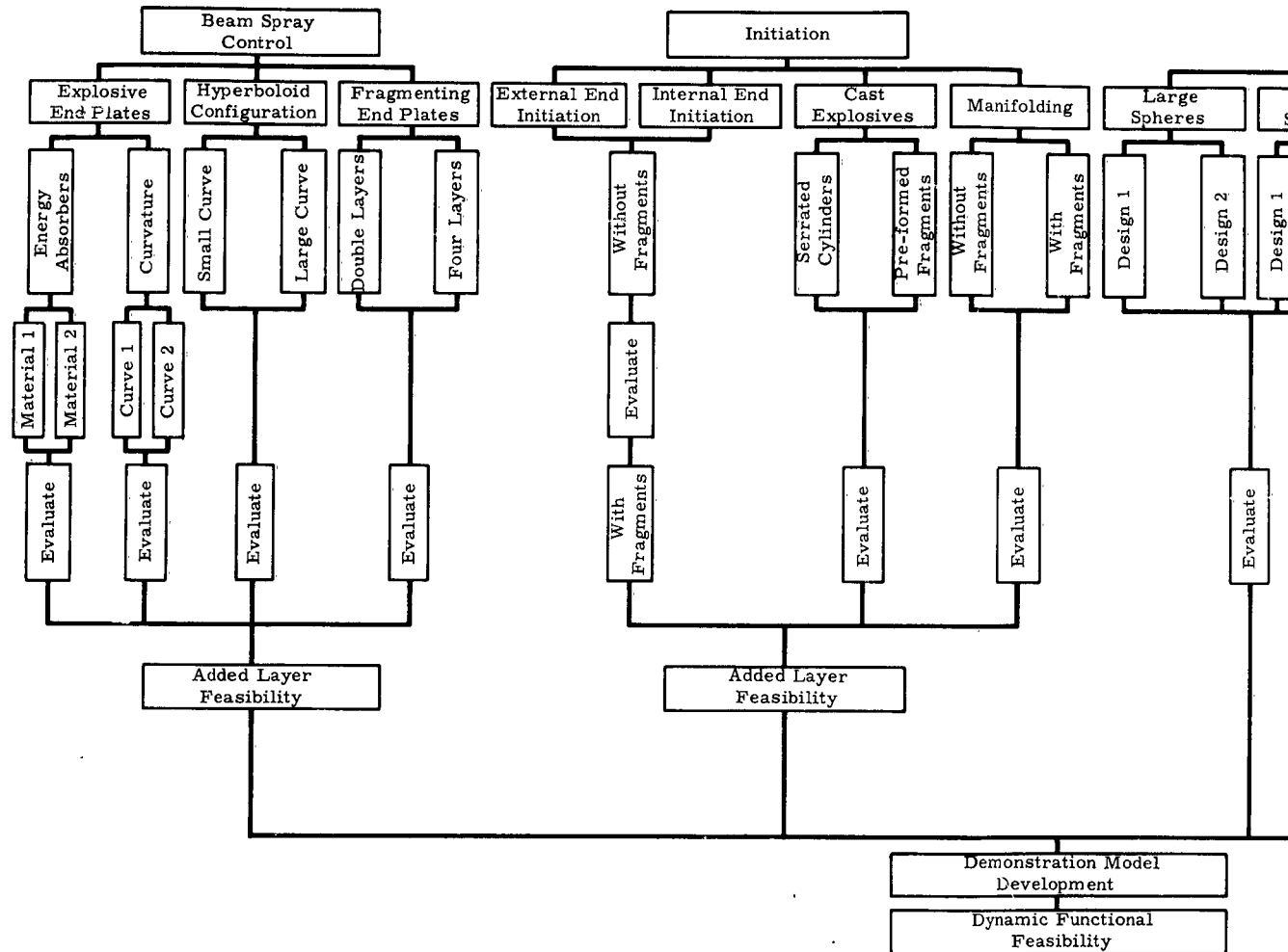
Figure 2. Experimental Program Flow
