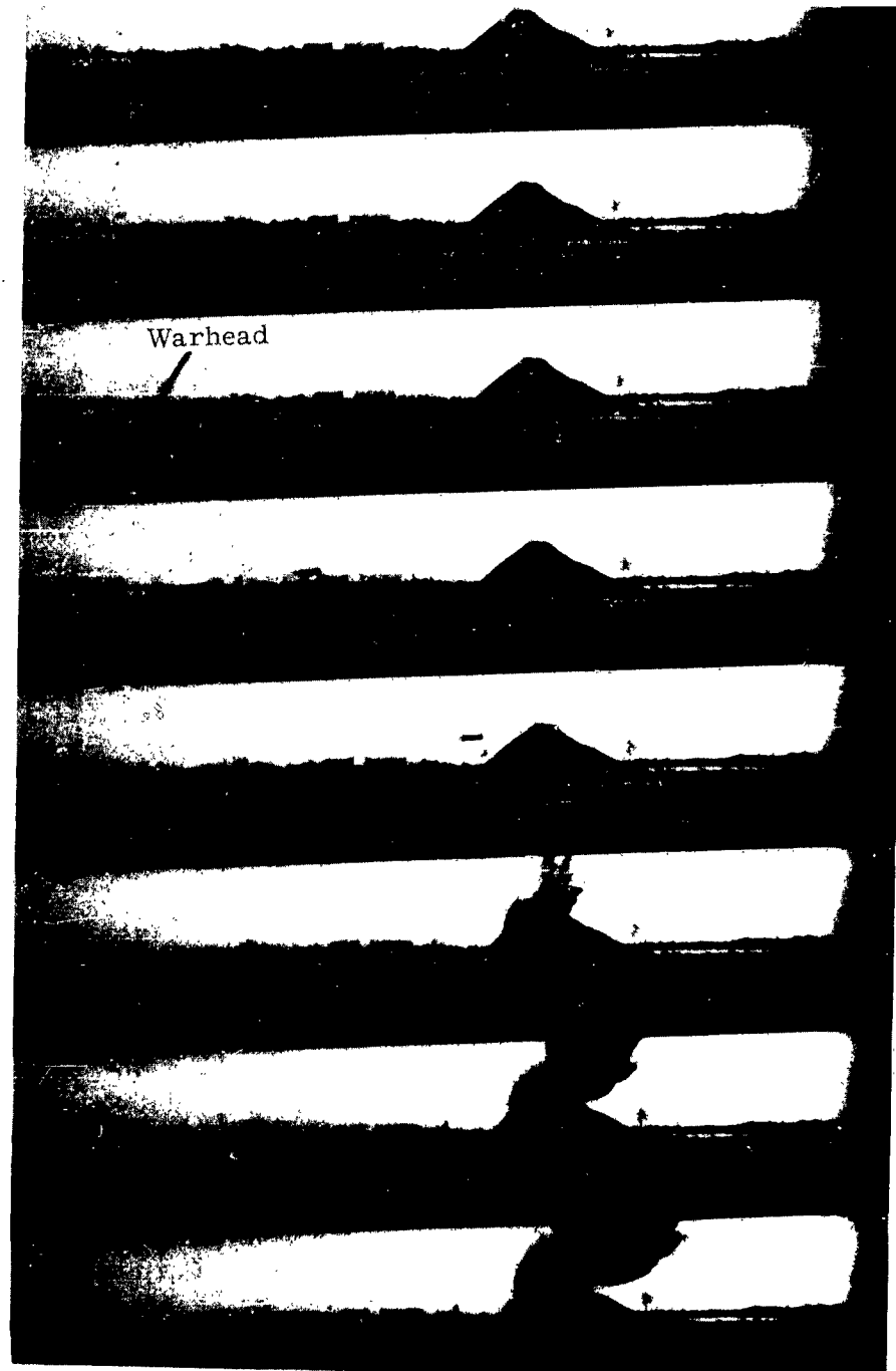
Figure 18. CZR Camera Record of Inert Model Sled Test
