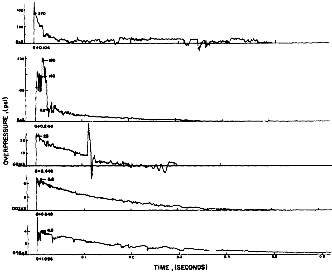
Figure 3.9 Dynamic pressure versus time records.
