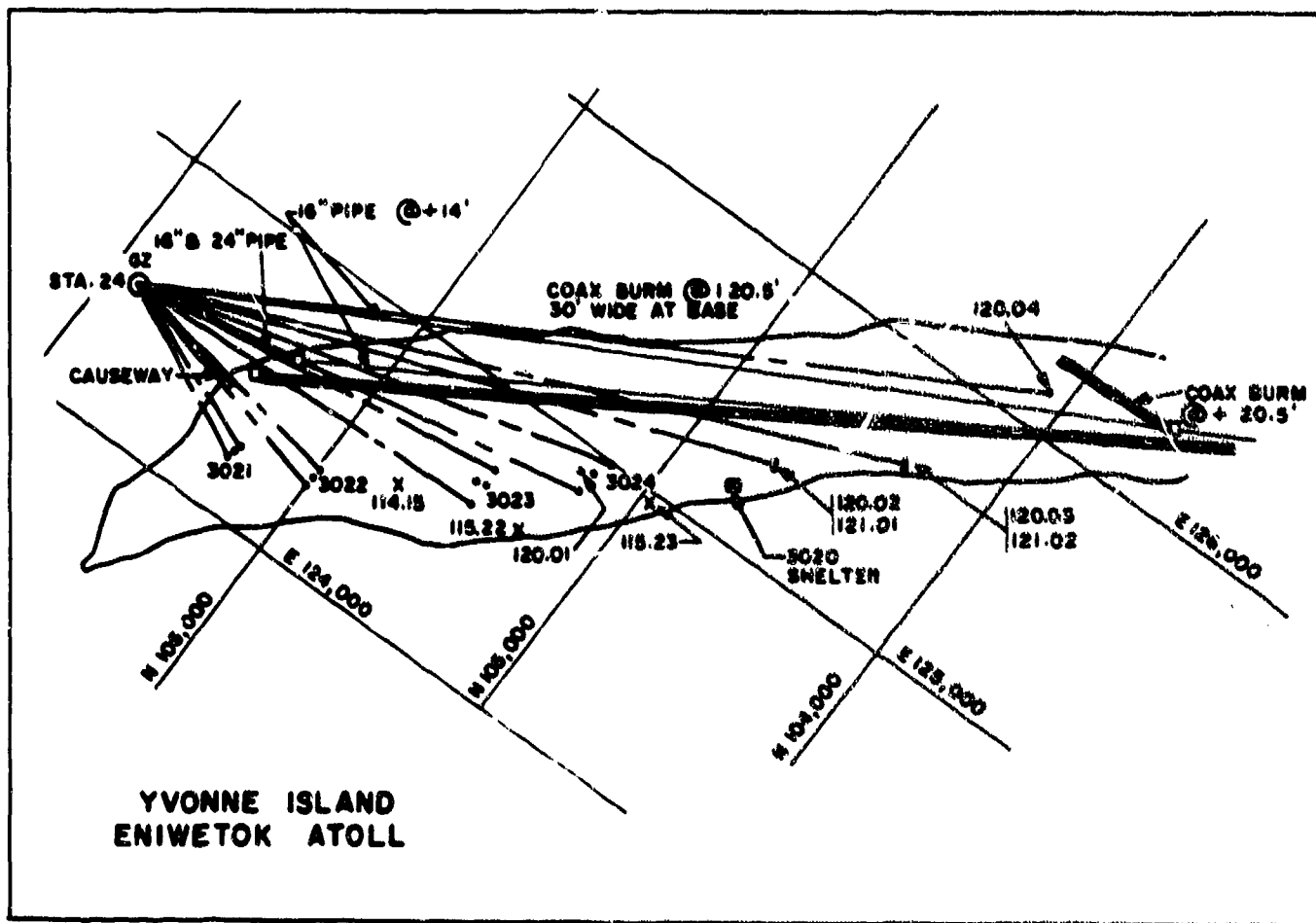
Figure 2.1 Gage layout.
