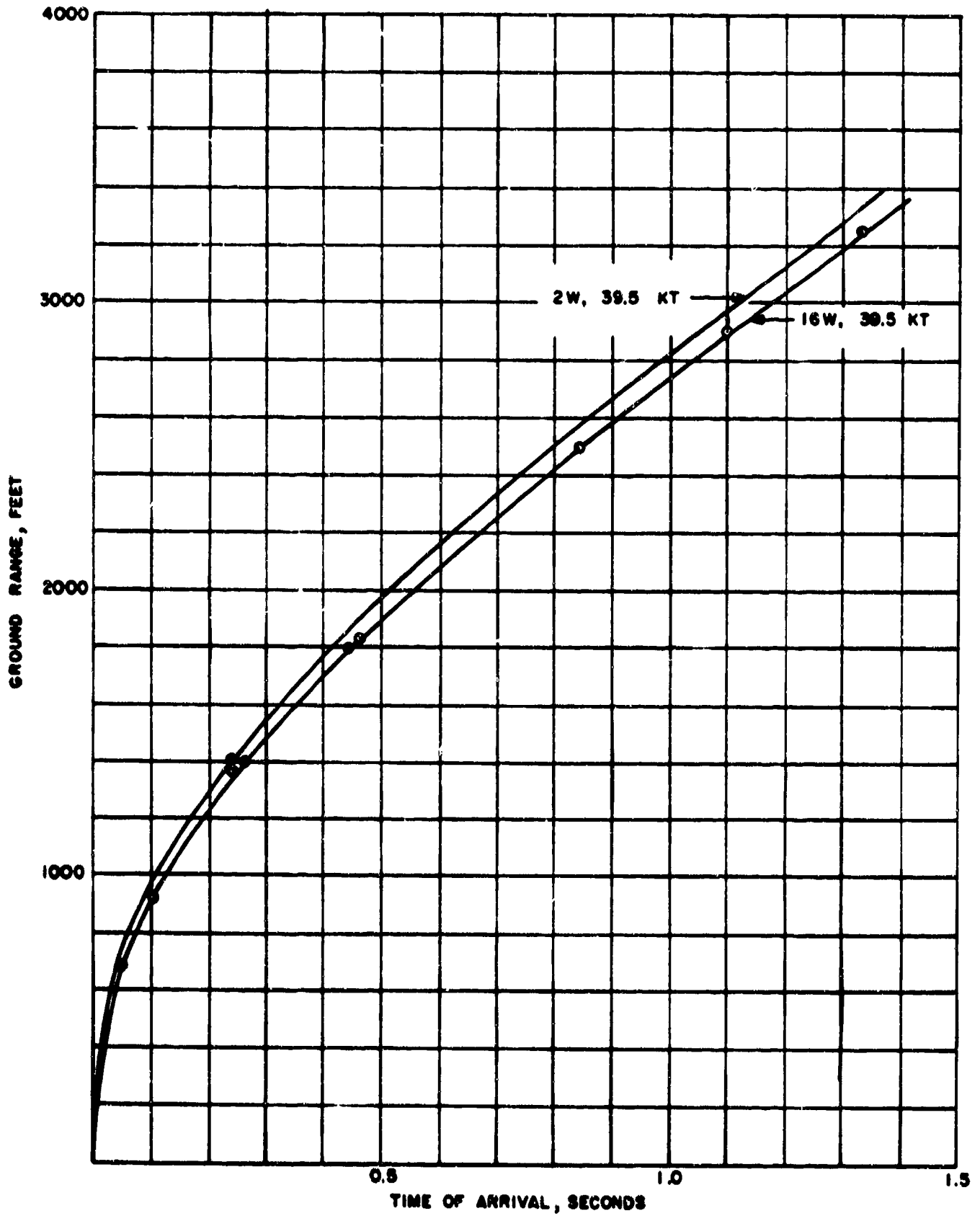
Figure 3.1 Arrival time versus ground range.
