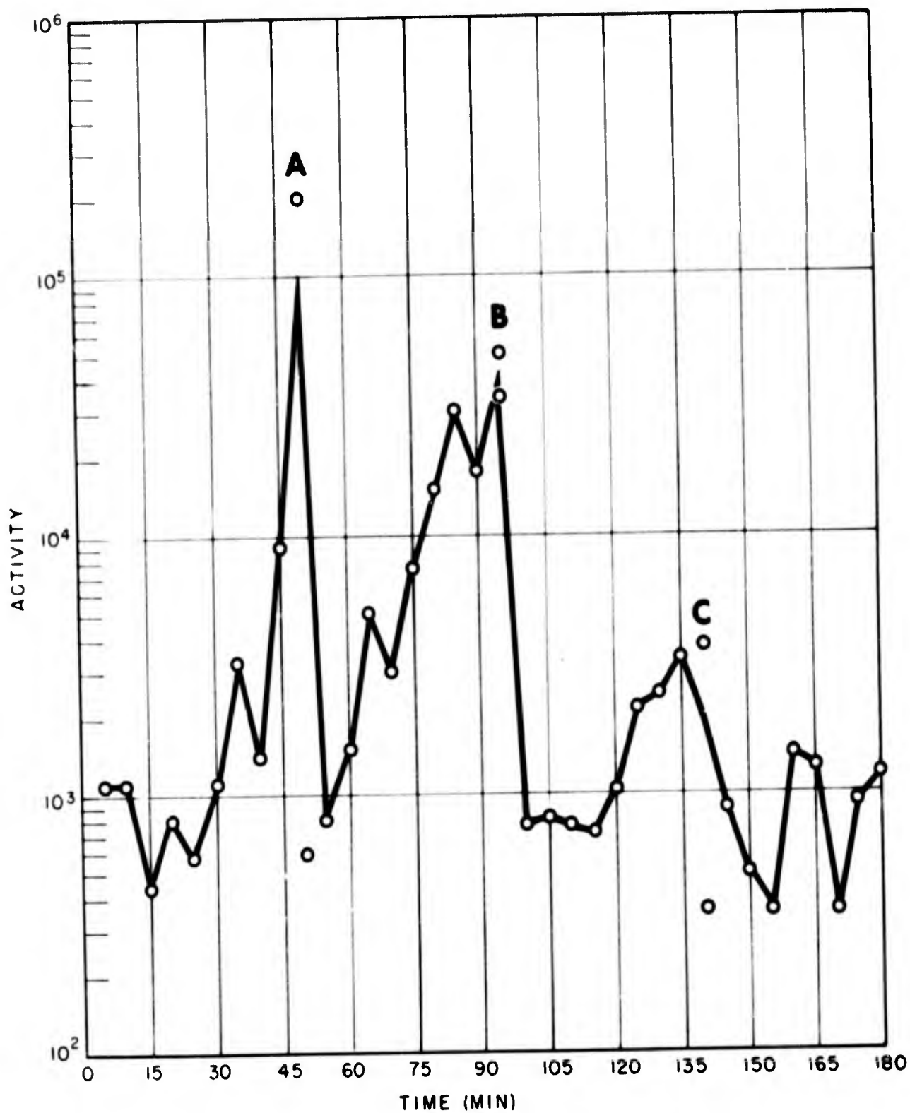
Fig. C.11 Shot 1, Time of Arrival and Period of Fallout, Station 250.22
