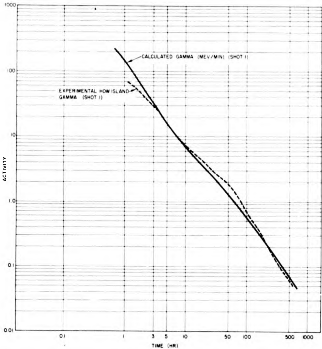
Fig. 5.2 Calculated Gamma Decay Curve and Experimental Gamma Ionization Decay Curve for Shot 1
