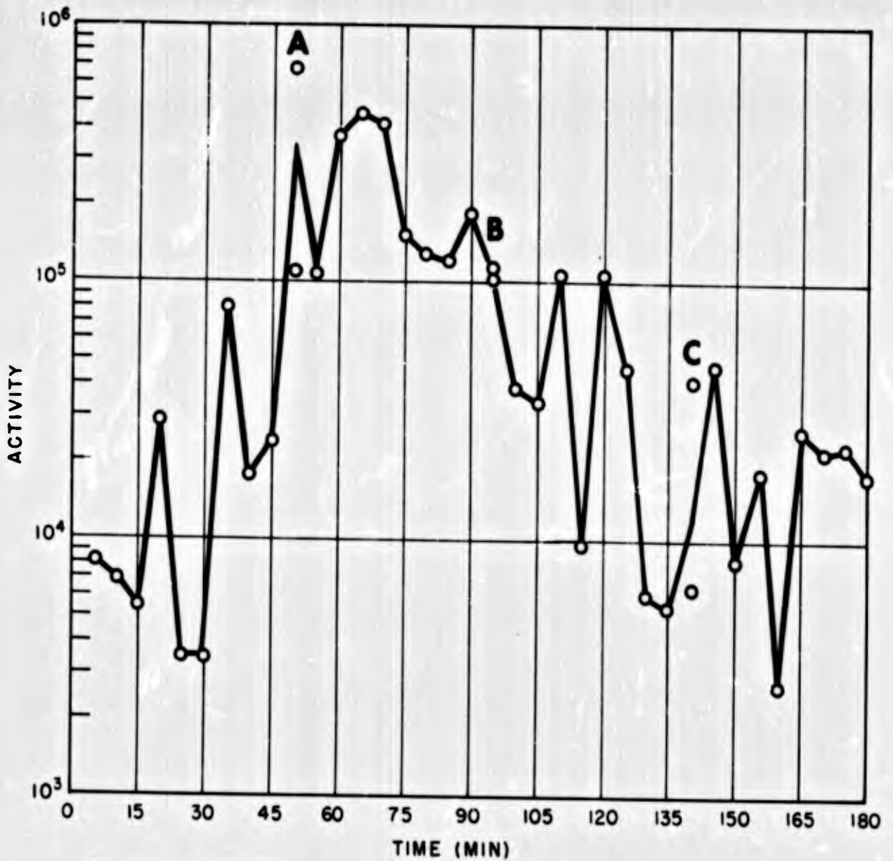
Fig. C.14 Shot 1, Time of Arrival and Period of Fallout, Station 251.05
