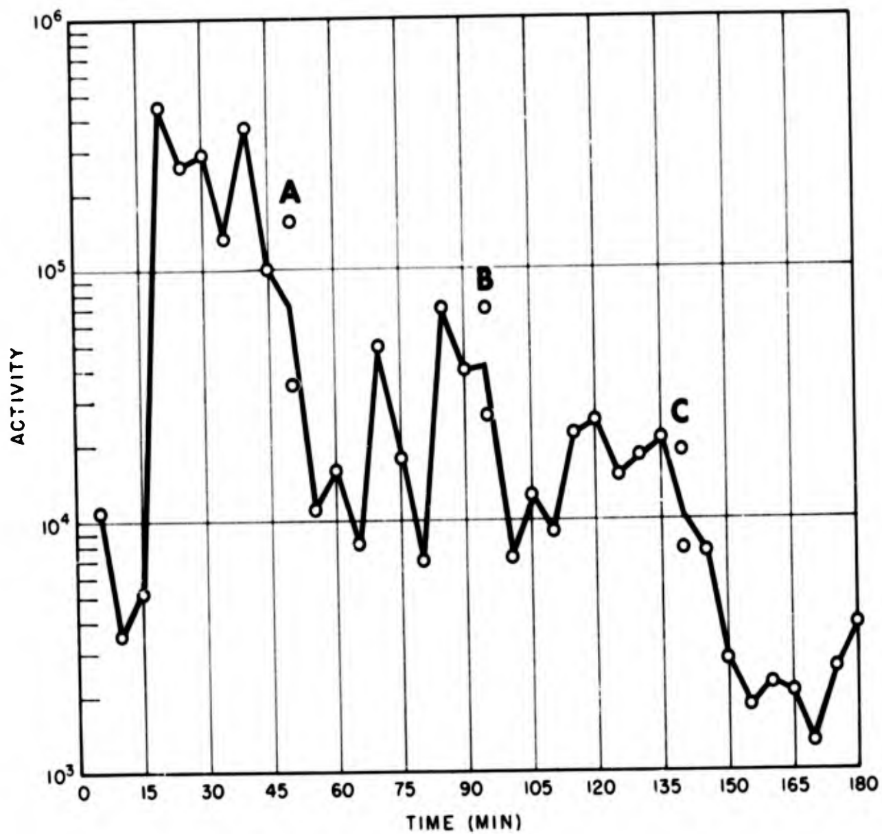
Fig. C.9 Shot 1, Time of Arrival and Period of Fallout, Station 250.05 (A,B, and C as in text p. 69)
