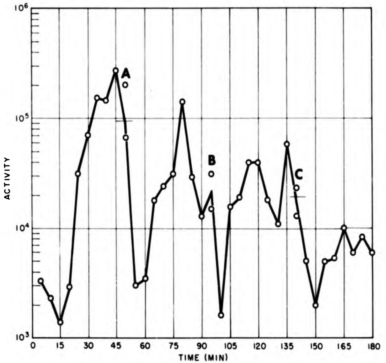
Fig. C.10 Shot 1, Time of Arrival and Period of Fallout, Station 250.06
