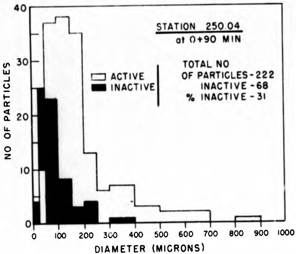
Fig. 5.9 Shot 1, Ratio of Active to Inactive Particles
