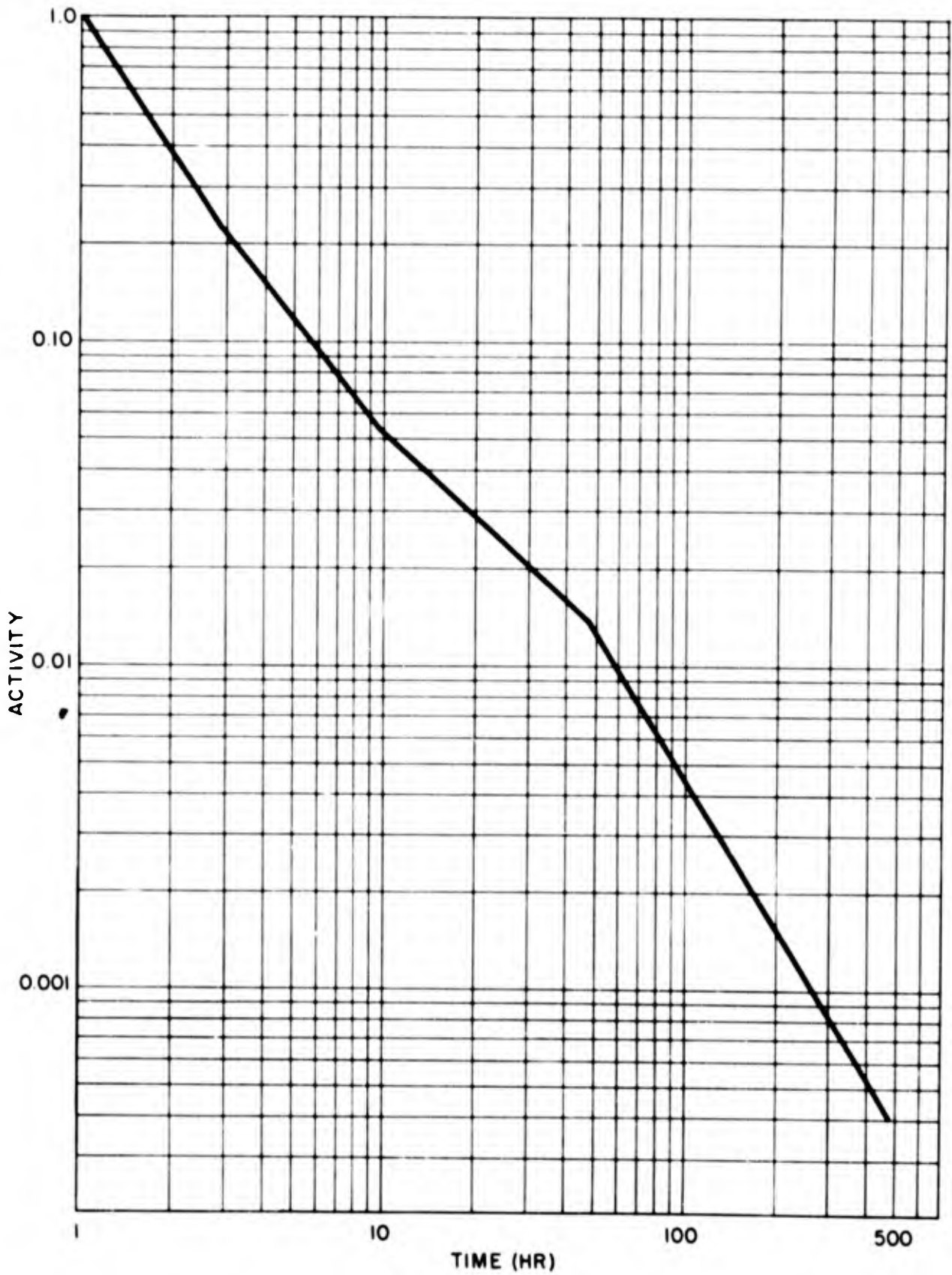
Fig. 5.3 Composite Gamma Ionization Decay Curve
