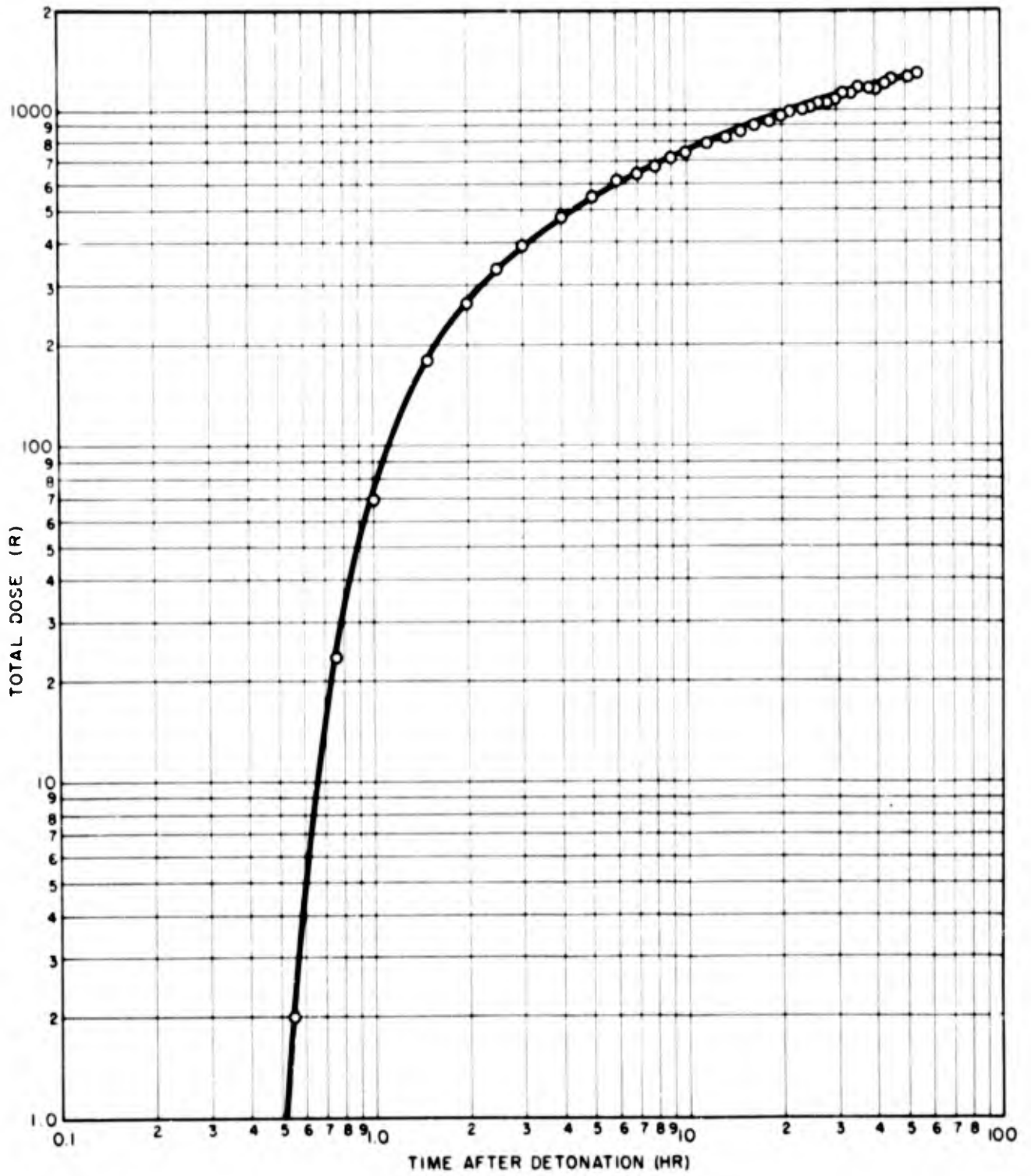
Fig. 5.11 Shot 1, Integrated Gamma Dose, Station 251.03
