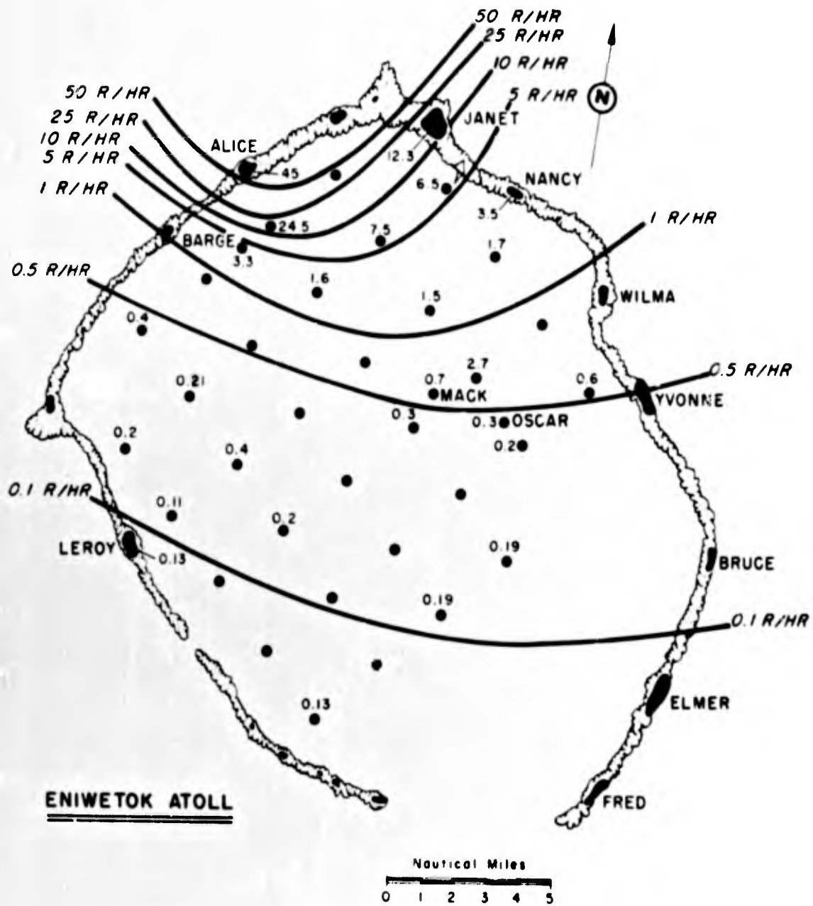
Fig. 6.4 Shot 6, Close-in Gamma Fallout Pattern (r/hr at 1 hr)
