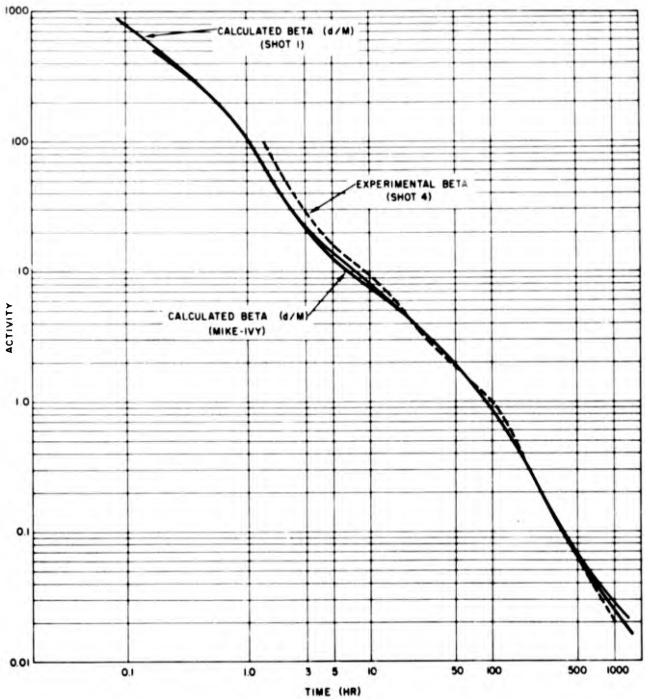
Fig. 5.1 Experimental and Calculated Beta Decay Curves
