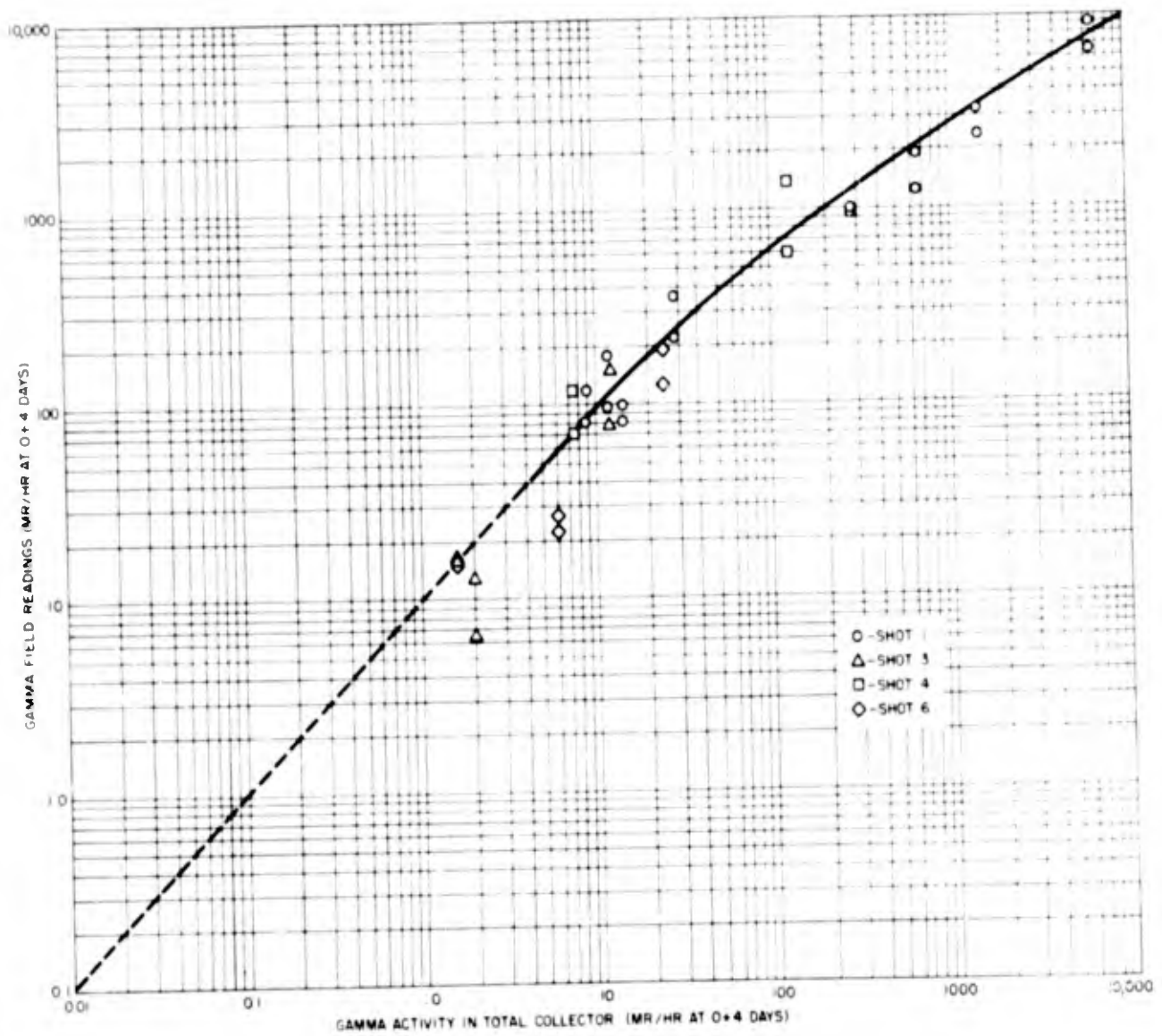
Fig. 4.1 Ratio of Gamma Infinite Field Measurements to Equivalent Gamma Measurements From the Total Collector (mr/hr at 0 + 4 days)
