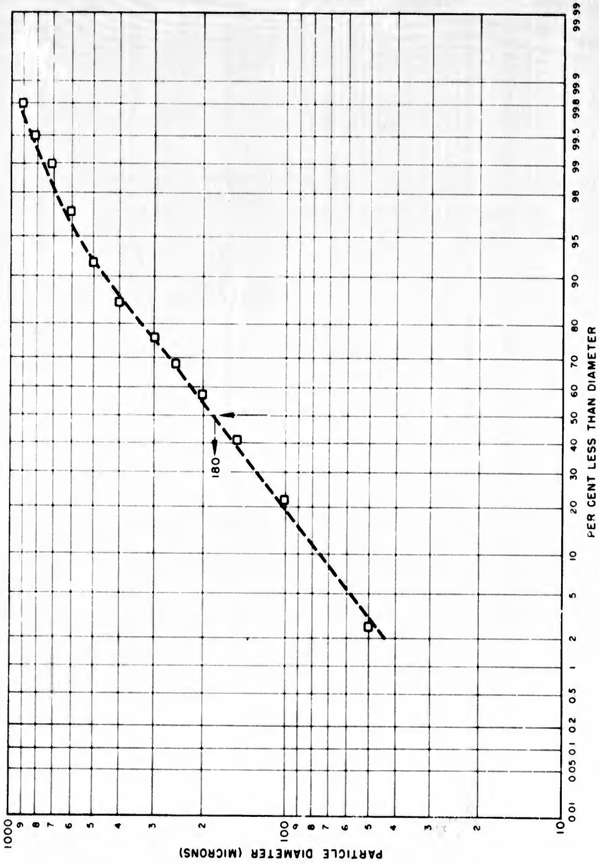
Fig. 5.8 Shot 6, Cumulative Particle Size Distribution, Station Alice
