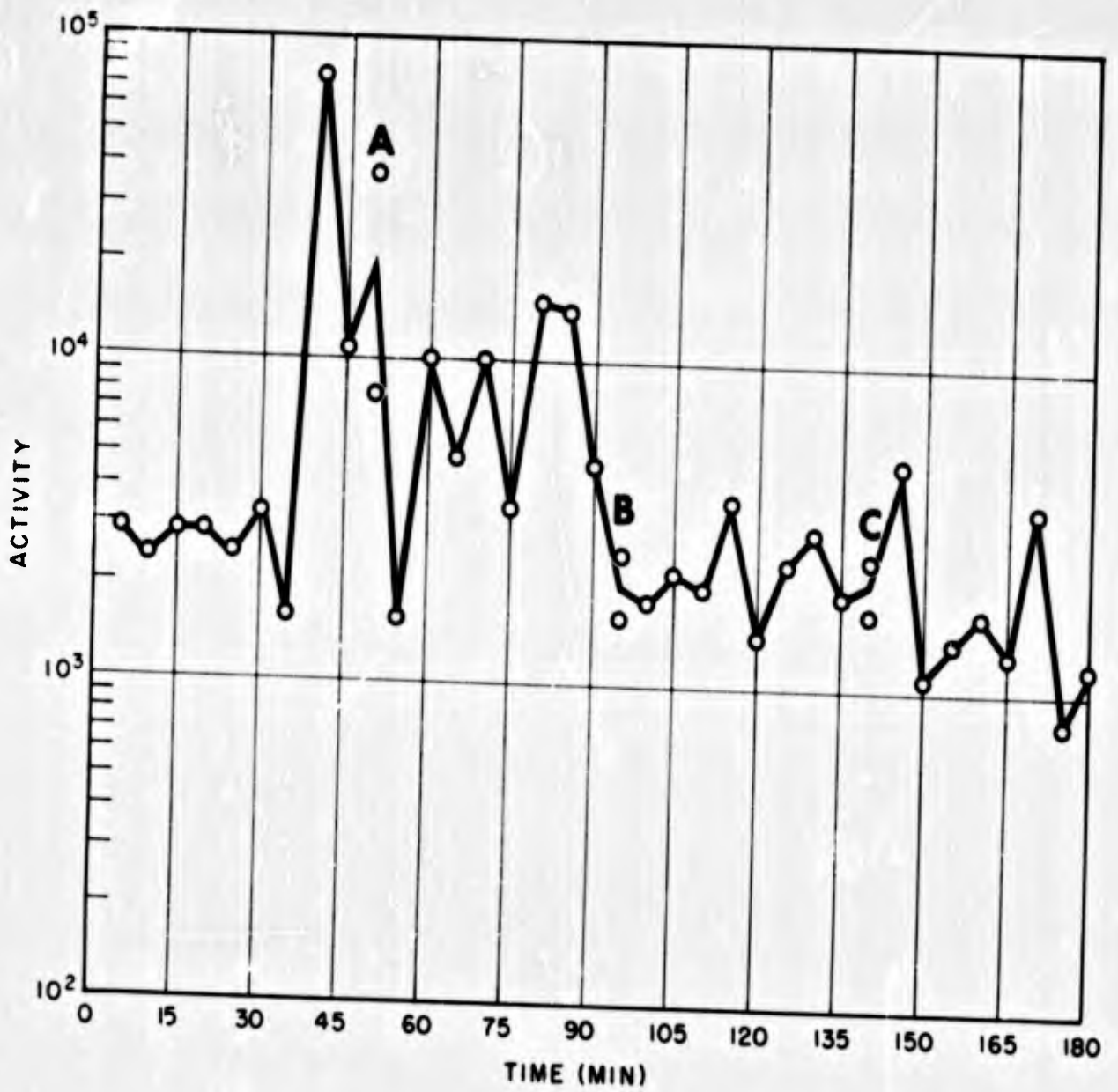
Fig. C.16 Shot 1, Time of Arrival and Period of Fallout, Station 251.10
