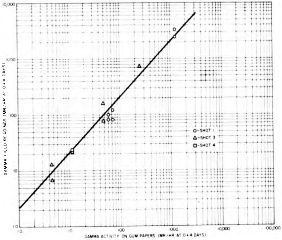
Fig. 4.2 Ratio of Gamma Infinite Field Measurements to Equivalent Gamma Measurements from the Gummed Paper Collector (mr/hr at 0 + 4 days)
