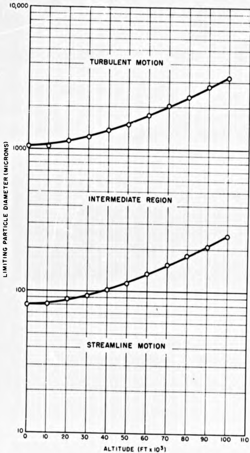
Fig. E.1 Areas of Applicability in Calculating Terminal Velocities
