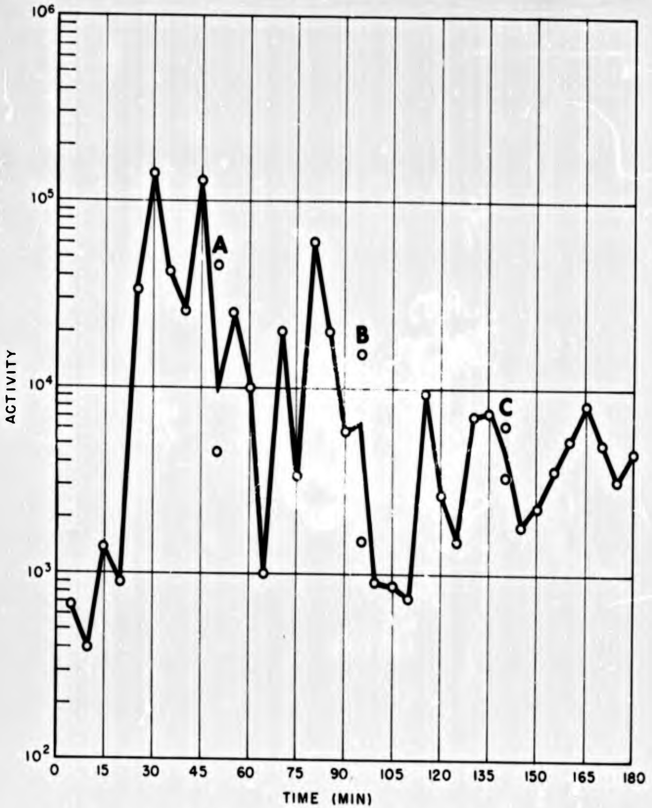
Fig. C.15 Shot 1, Time of Arrival and Period of Fallout, Station 251.06
