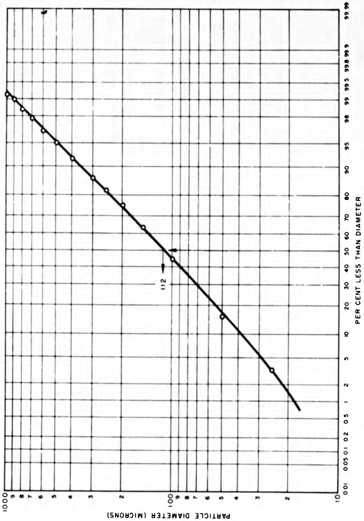
Fig. 5.5 Shot 1, Cumulative Particle Size Distribution
