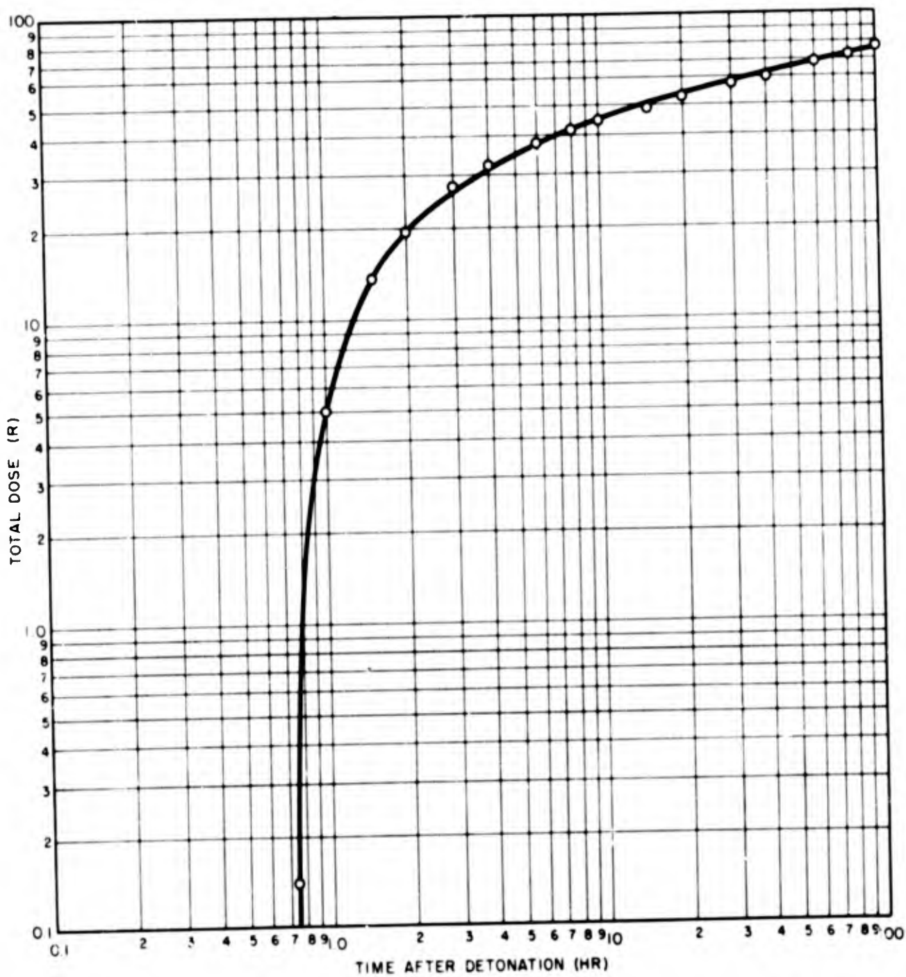
Fig. 5.12 Shot 3, Integrated Gamma Dose, Station 251.03
