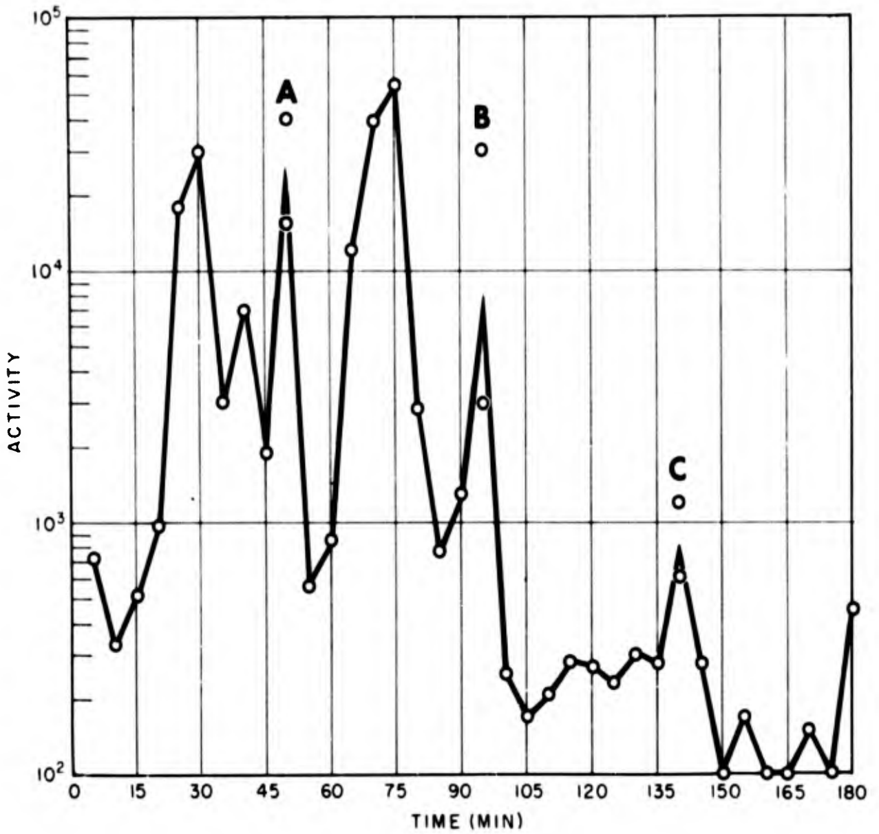
Fig. C.12 Shot 1, Time of Arrival and Period of Fallout. Station 250.24
