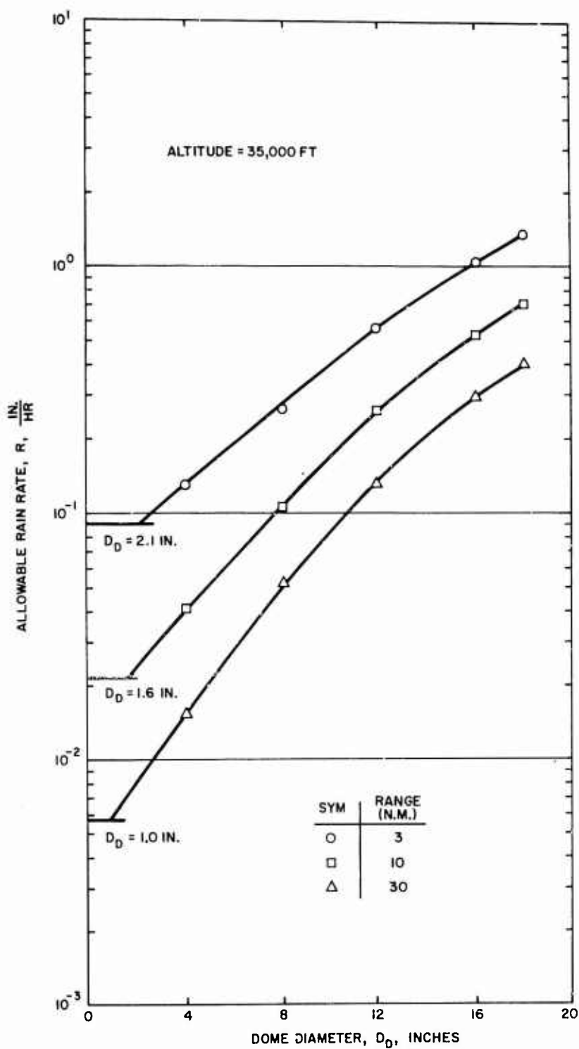
Figure 25. Allowable Rain Rate Versus Dome Diameter for a Flight at 35000 Feet.
