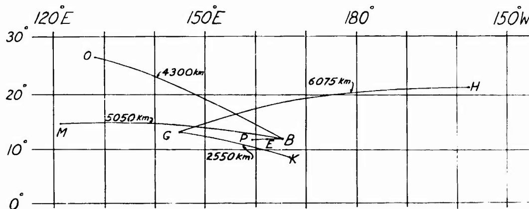
Fig. 2.1—Great-circle transmission paths and distances showing relationship of the paths to GZ, Eniwetok (B, Bikini; P, Airplane; G, Guam; K, Kwajalein; H, Honolulu; O, Okinawa; M, Manila; and E, Eniwetok).
