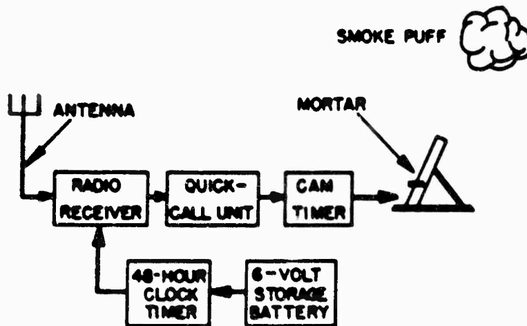
Fig. 2.4—Radio firing system (EG&G photograph).
