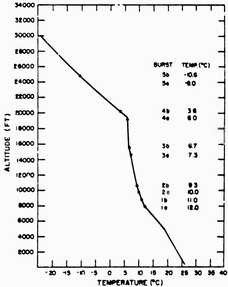
Fig. A.3—Ambient temperature vs. altitude.
