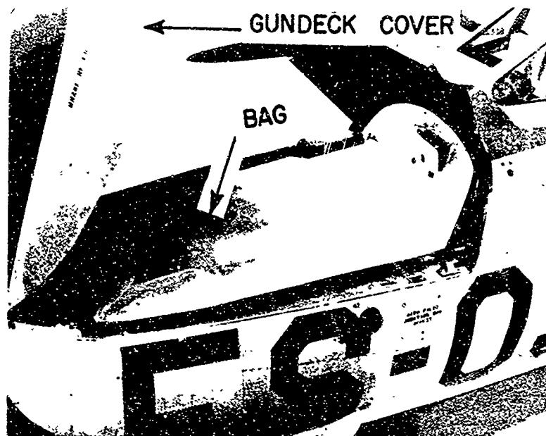
Fig. 3.7—Gun-deck cover opened, showing polyethylene bag installed in gun-deck liner.
