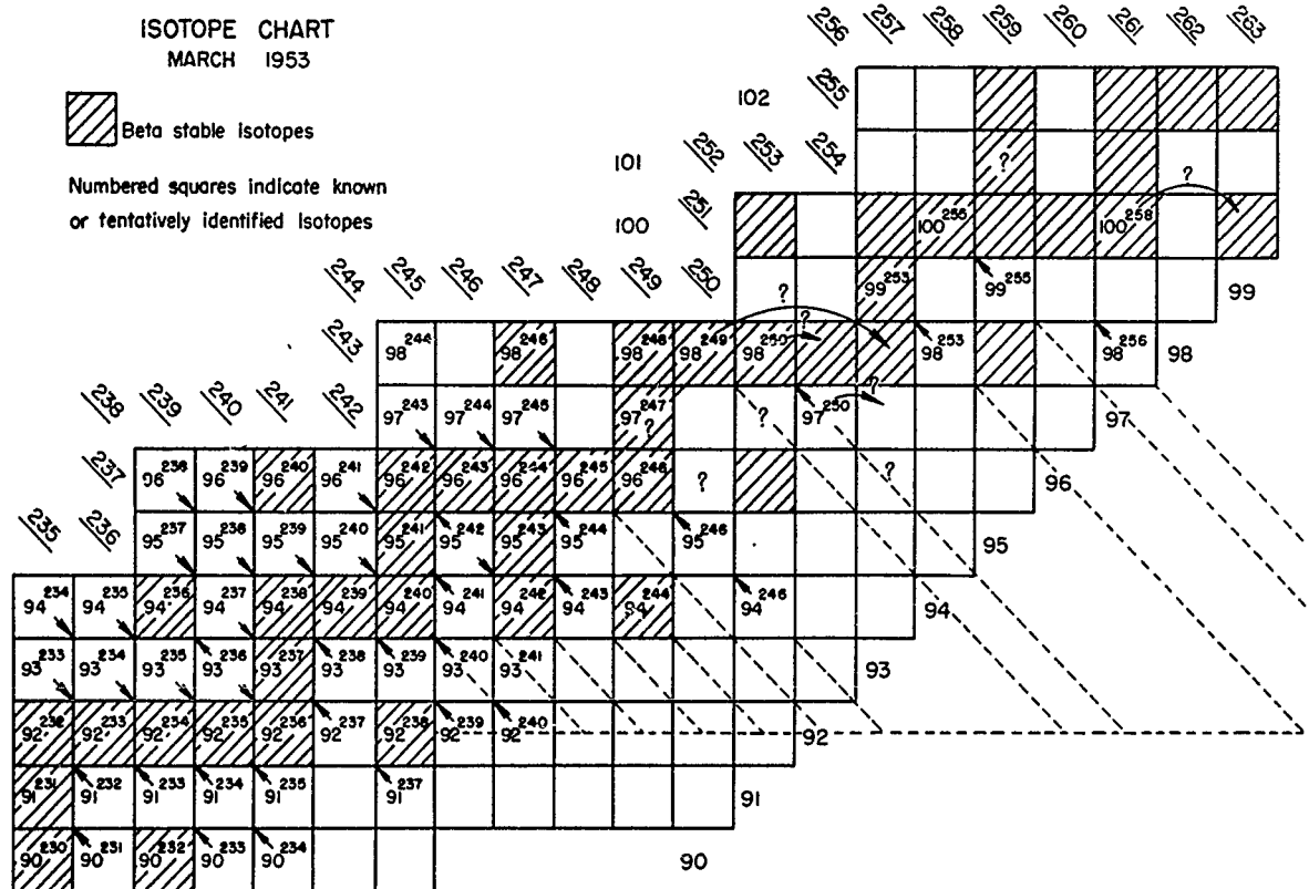
Fig. 11.1—UCRL isotope chart of heavy nuclides.
