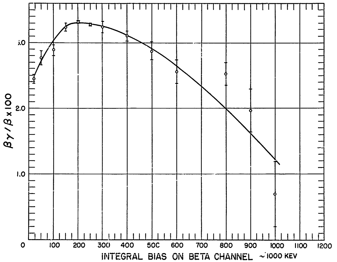
Fig. 5.1—Beta-gamma coincidences per beta in equilibrium Pu 246 -Am 246 sample.
