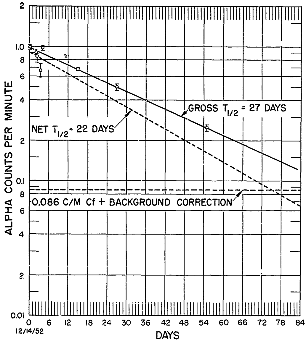
Fig. 8.28—UCRL elutions; decay of 6.8-Mev alpha activity in 99 fraction.
