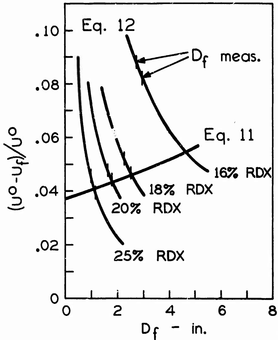
FIG. 7 CALCULATED RELATION BETWEEN D_f AND (U^0 - U_f)/U^0 FOR PBAA COMPOSITE PROPELLANTS CONTAINING RDX.
