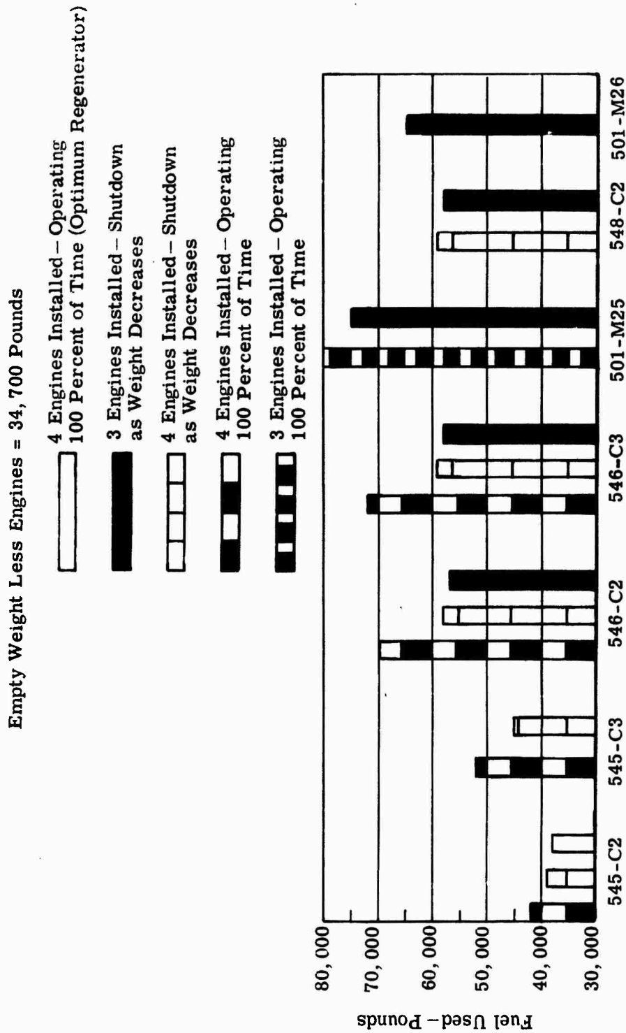
Figure 39. (C) Ferry Mission—Fuel Required (U)
