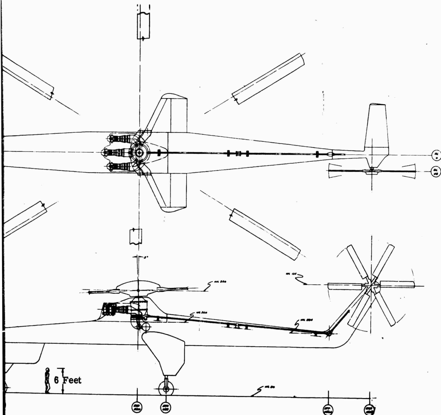
Integrated Engine-Power Turbine Transmission Drive System (SK-10082)
