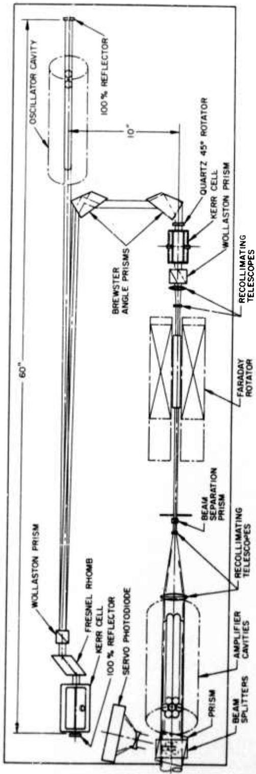
Figure 16. High energy controlled pulse oscillator-amplifier optical layout.
