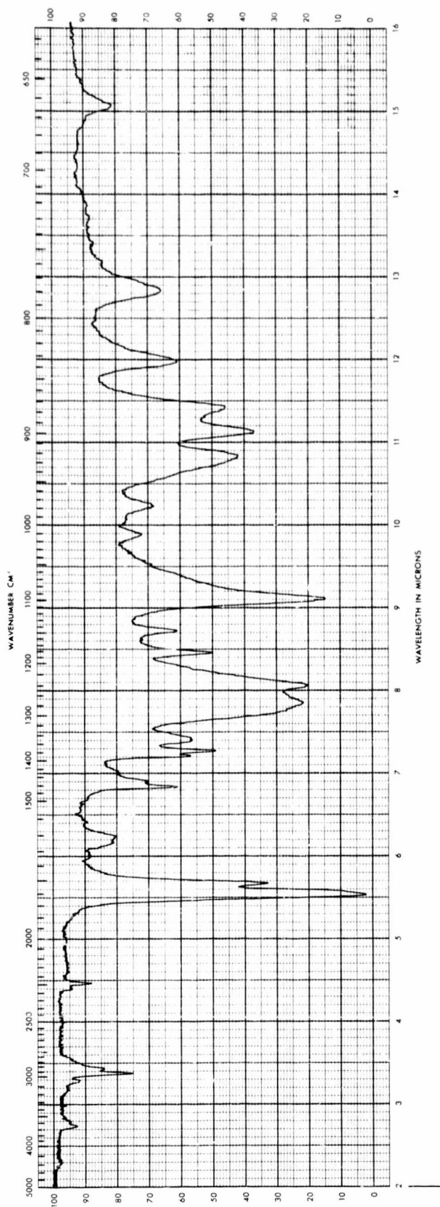
Fig. 13. Infrared Spectrum of 1-Carboisopropoxyperfluoroguanidine (C 31 PFG)
