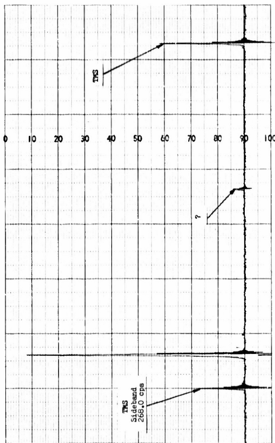
Fig. 7. Infrared Spectrum of 1-Carbomethoxyperfluoroguanidine (C 1 PFG)
