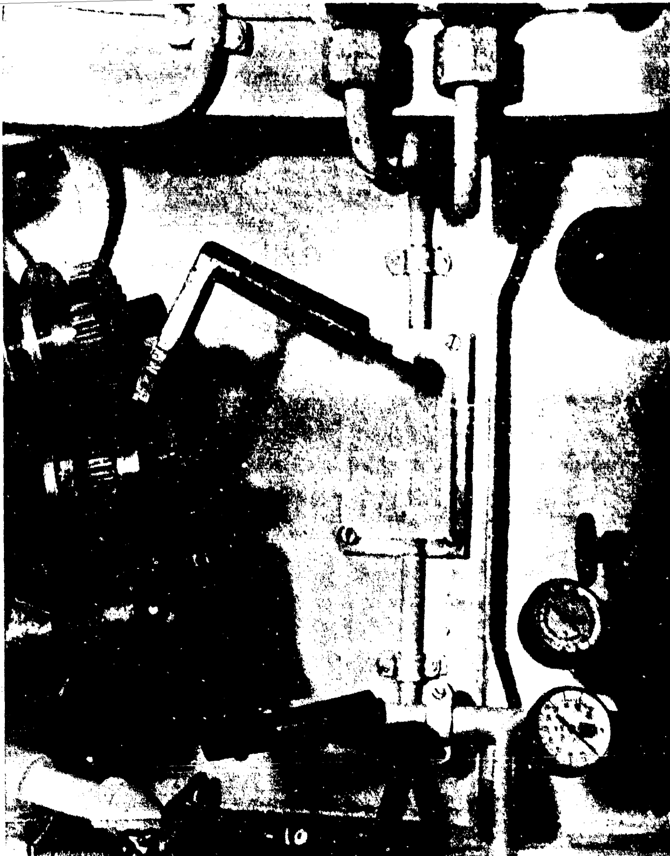
AA-CR-59-2011-10. Control room submerged signal sector showing operating shaft pushed in and bent operating handle gears not meshed.
