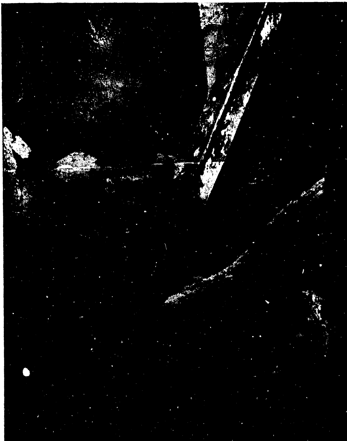
AA-CR-68-1752-8. Closeup of dislocation of No. 6 torpedo tube impulse air flash showing rupture in pipe at flange.
