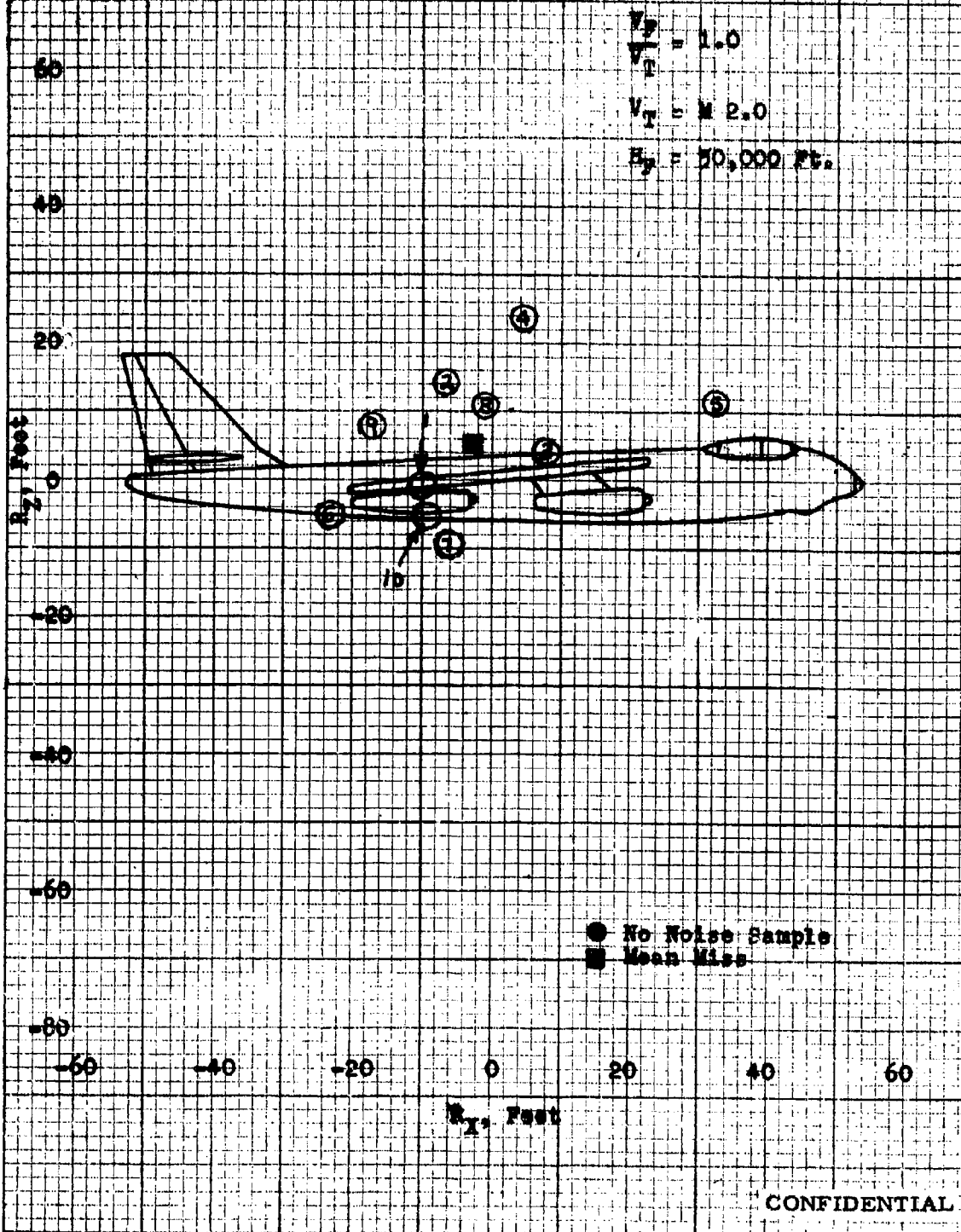
Fig. 17- Sparrow III Miss Distance - Co-altitude Attacks X-Z Miss Distance at the Target T_a = 60^\circ , Launch ( T_f + 2 ) sec after R_{max} Fighter Course - D-1
