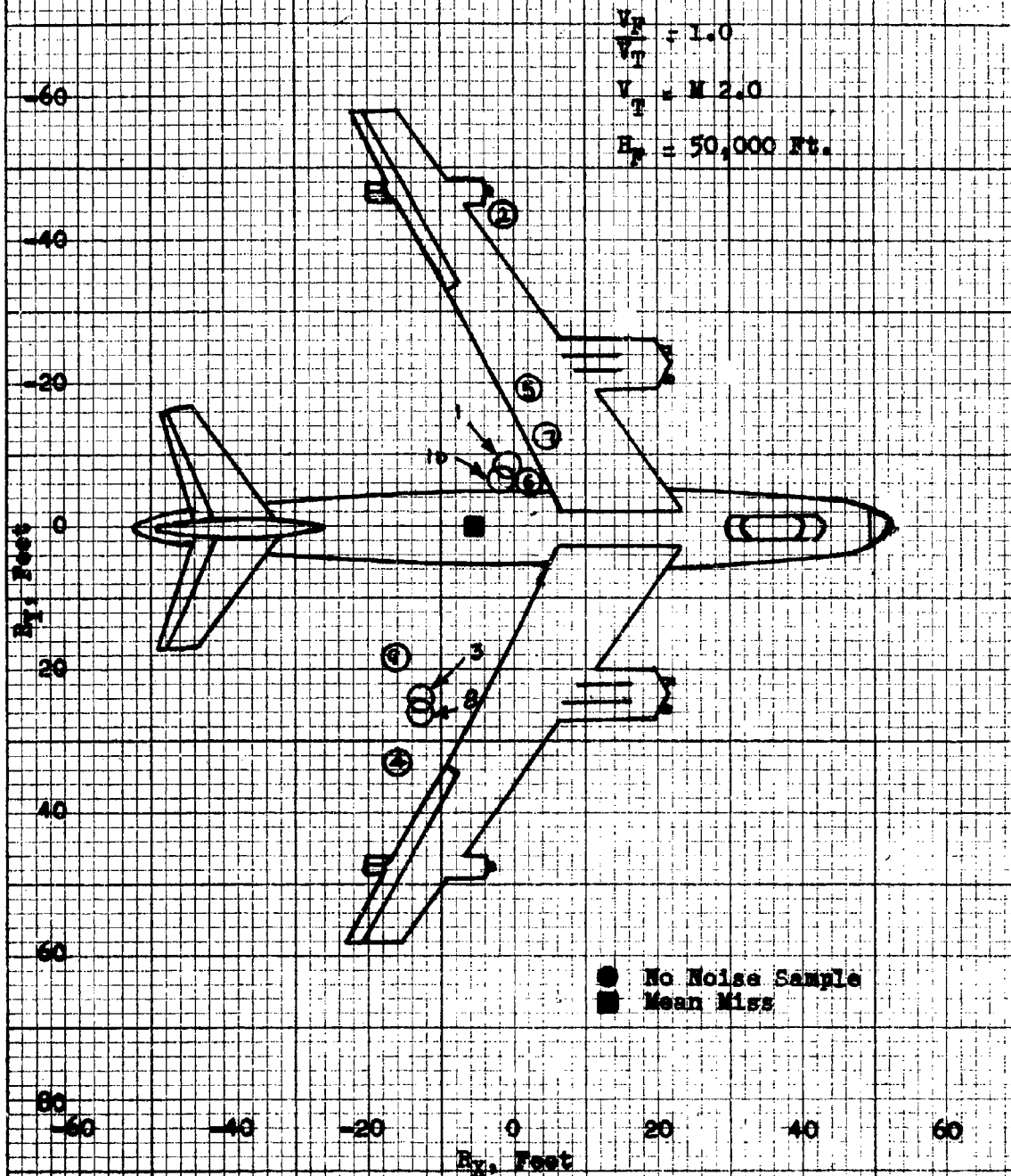
Fig. 7a - Sparrow III Miss Distance - Co-altitude Attacks X-Y Miss Distance at the Target T_0 = 15^\circ ; R_{\text{max}} Launch, Fighter Course - D-I
