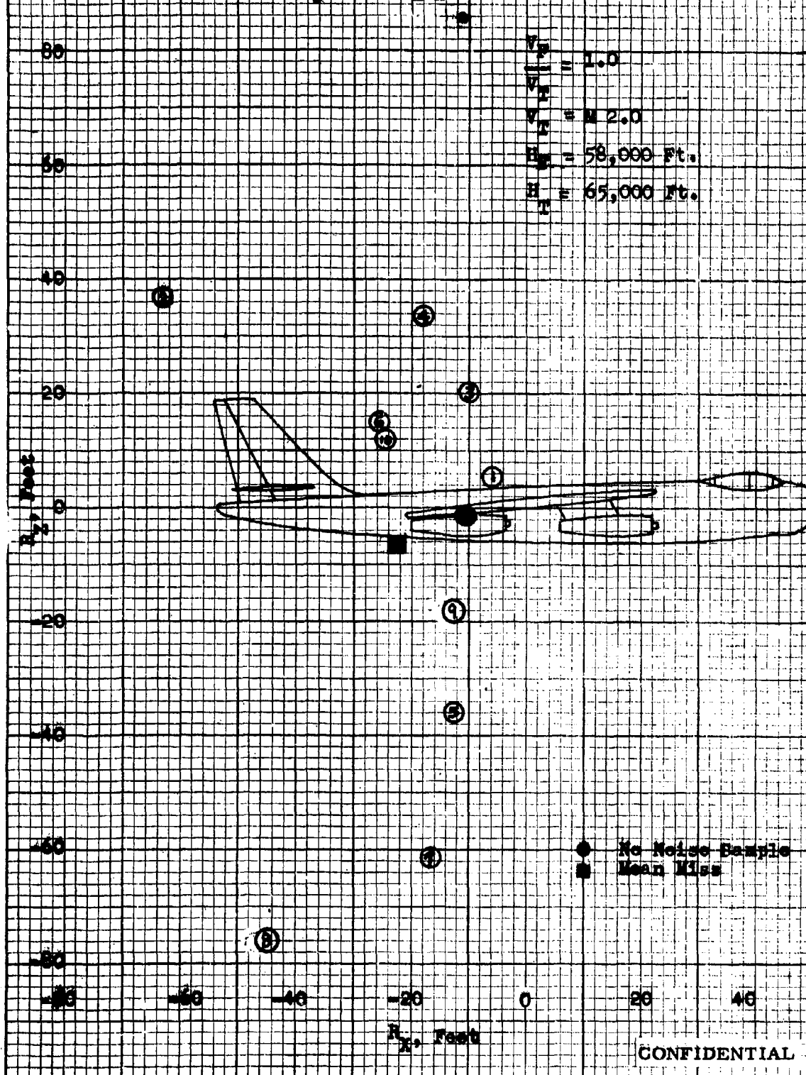
FIG. 23D - Sparrow III Miss Distance - Pull-up Attacks X-Z Miss Distance at the Target T = 45^\circ , R_{\text{max}} Launch, Fighter Course - E-4
