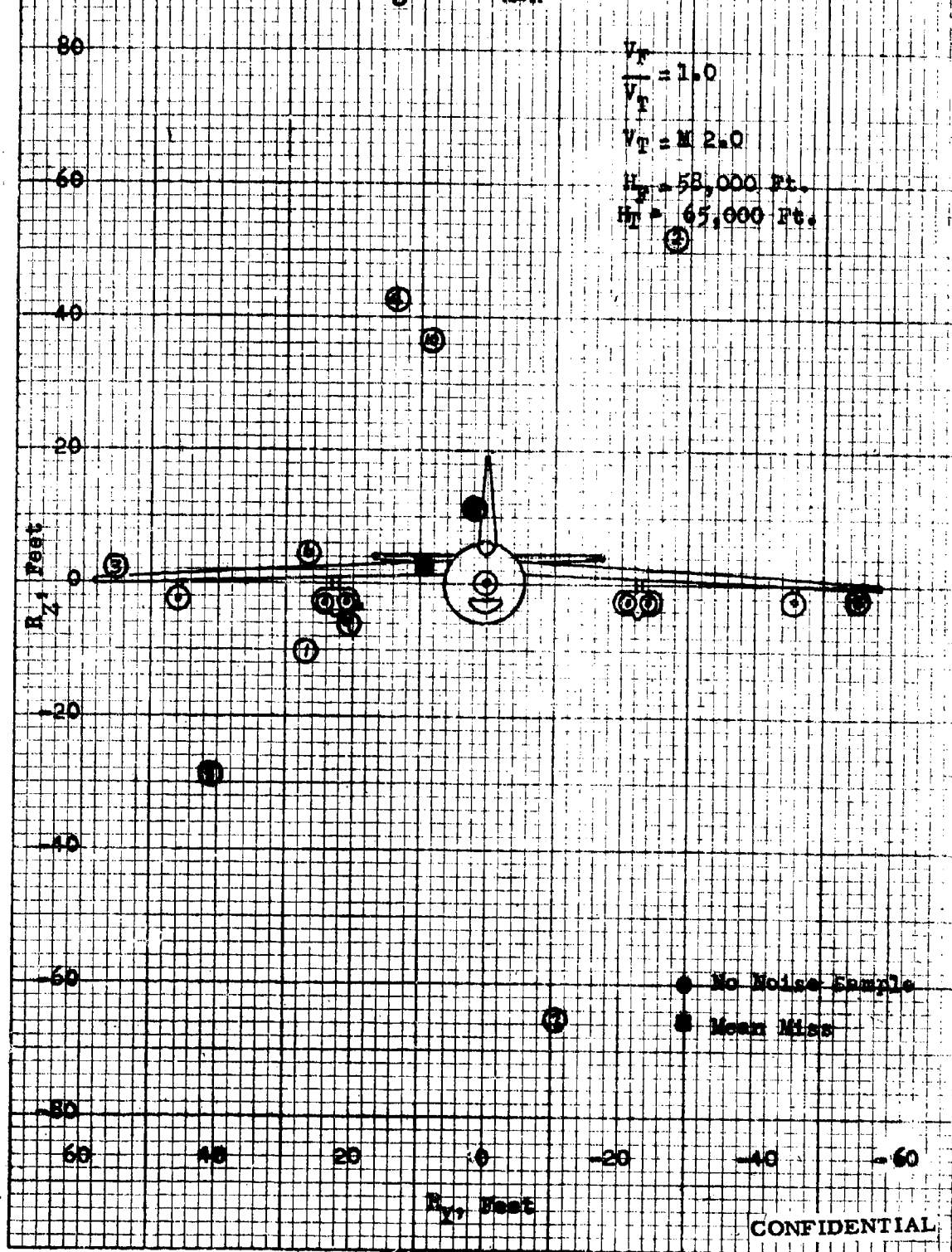
Fig. 18c - Sparrow III Miss Distance - Pull-up Attacks Y-Z Miss Distance at the Target \gamma_0 = 0^\circ , R_{\text{Max}} launch, Fighter Course - D-1
