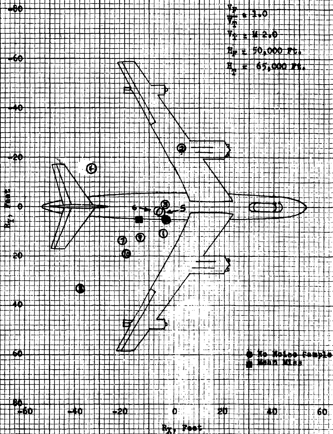
Fig. 26a - Sparrow III Miss Distance - Pull-up Attacks X-Y Miss Distance at the Target \gamma_0 = 45^\circ , R_{\text{max}} launch, Fighter Course - E-1
