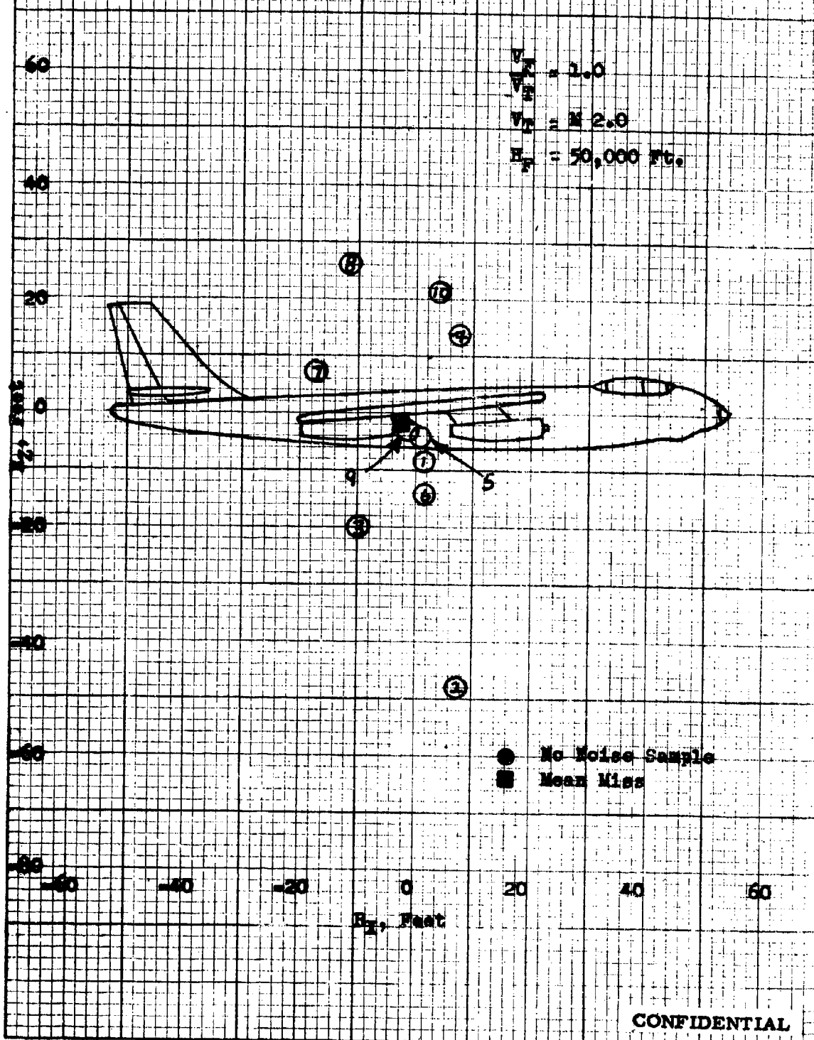
Fig. 14b Sparrow III Miss Distance - Co-altitude Attacks X-Z Miss Distance at the Target \gamma = 15^\circ , \lambda (Bear - Right) Launch Fighter Course - 0-3
