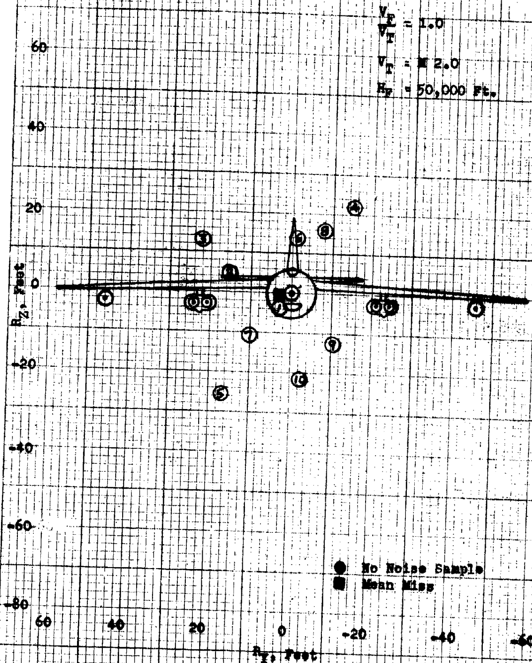
Fig. 8e- Sparrow III Miss Distance in Co-altitude Attacks Y-Z Miss Distance at the Target \gamma = 15^\circ , \pm(R_{\max} + R_{\min}) Launch Fighter Course - D-1
