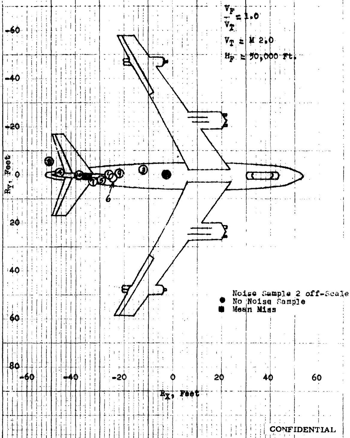
Fig. 16a - Sparrow III Miss Distance-Co-Altitude Attacks X-Y Miss Distance at the Target \gamma_0 = 60^\circ , R_{max} Launch, Fighter Course - D-1
