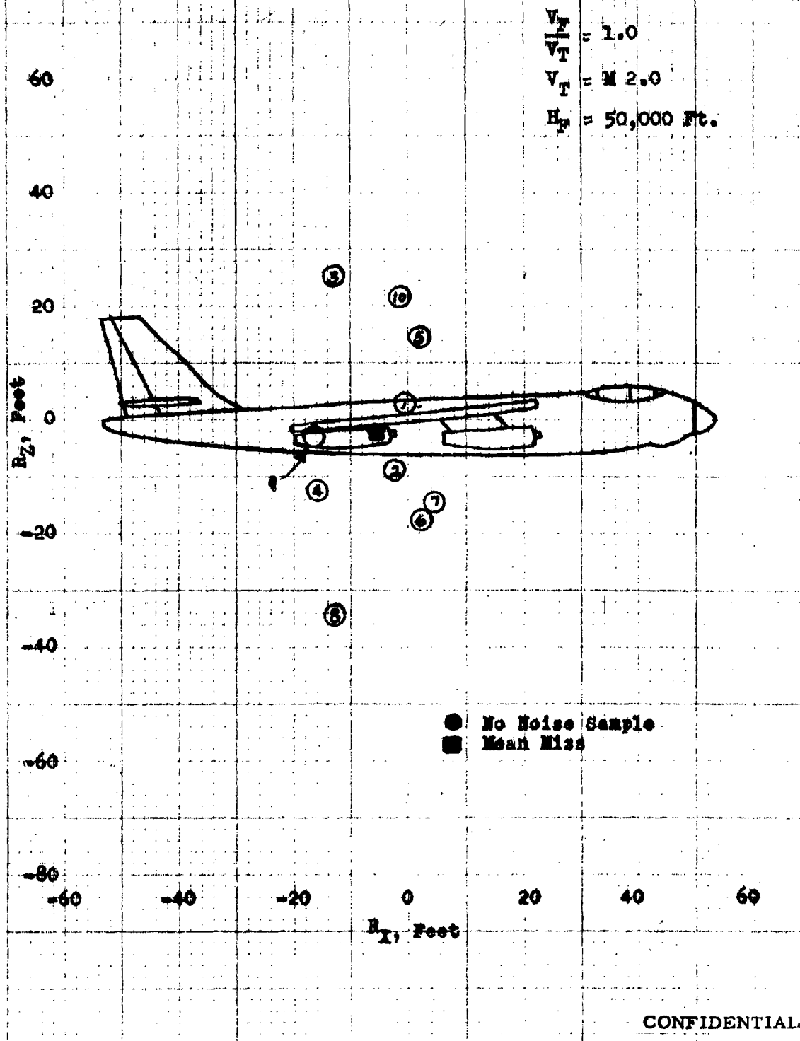
CONFIDENTIAL Fig. 7b- Sparrow III Miss Distance - Co-altitude Attacks R-Z Miss Distance at the Target \gamma_0 = 15^\circ , R_{\max} Launch, Fighter Course - D-1
