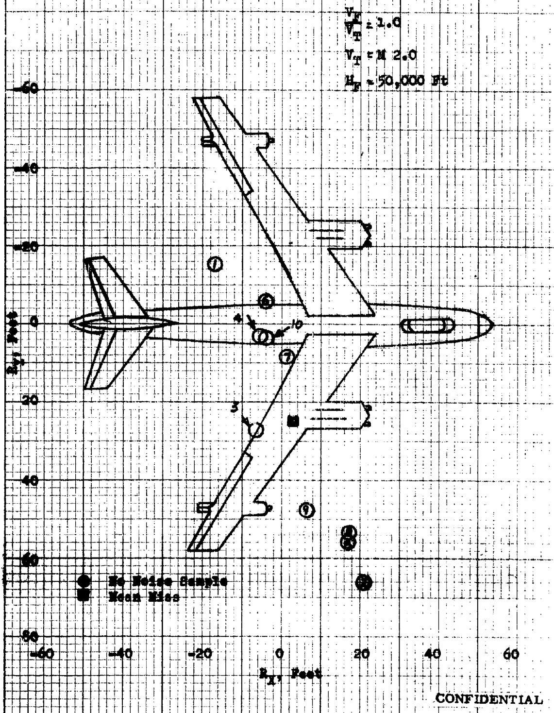
Fig. 13a- Sparrow III Miss Distance - Co-altitude Attacks CONFIDENTIAL \gamma_0 = 15^\circ , R_{\text{max}} Launch, Fighter Course - 8-3
