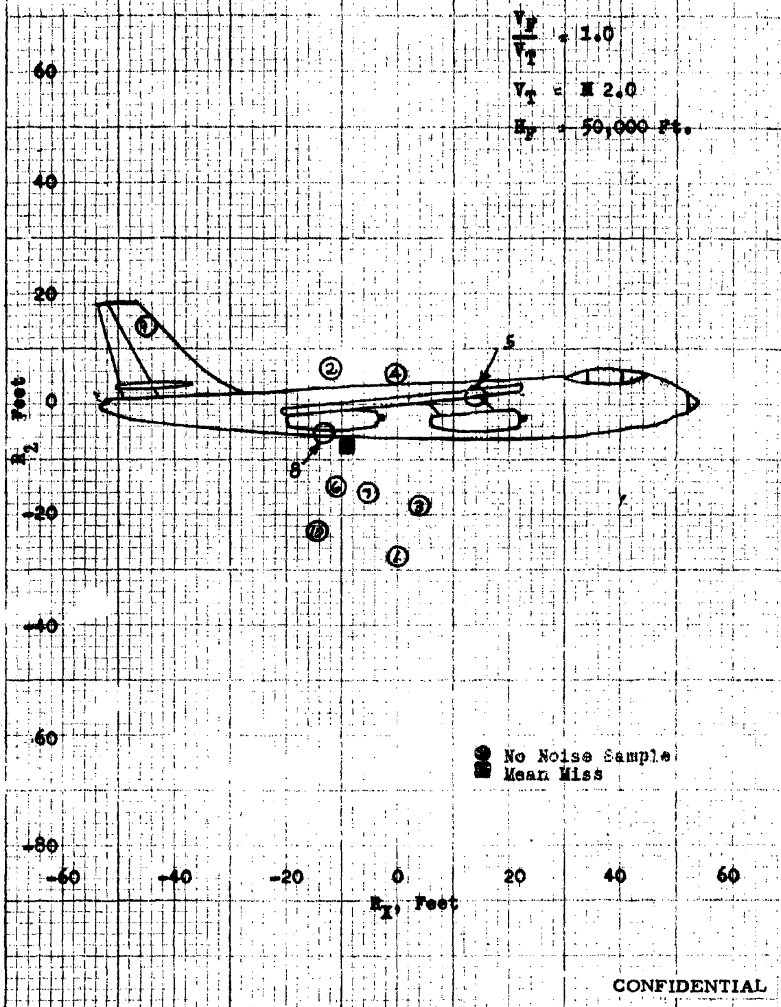
CONFIDENTIAL Fig. 4b- Sparrow III Miss Distance - Co-altitude Attacks X-Z Miss Distance at the target T_0 = 15^\circ , R_{Max} Launch, Fighter Course - B-3
