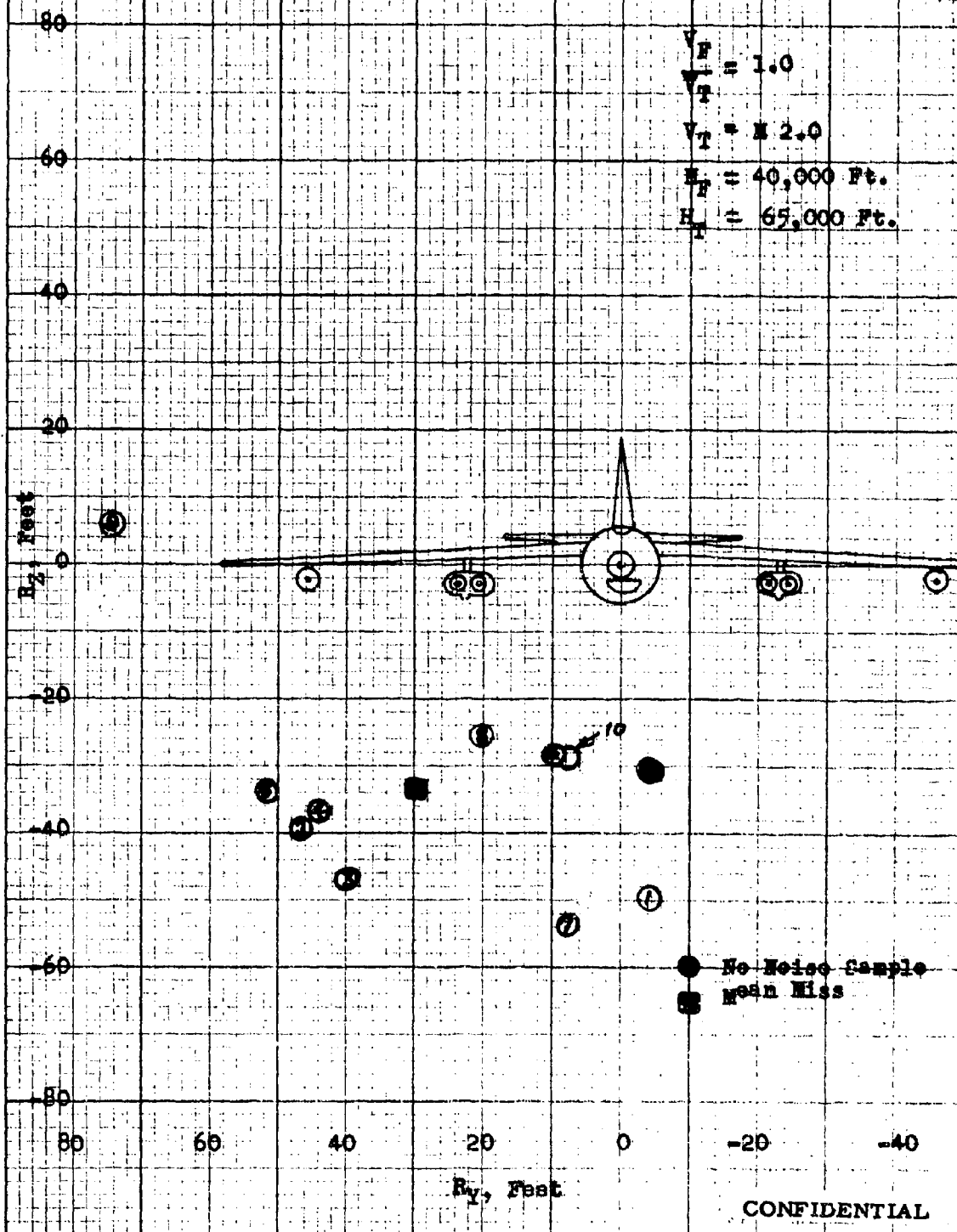
Fig. 6a- Sparrow III Miss Distance (Improved Missile) Pull-up Attacks Y-2 Miss Distance at the Target \gamma_0 = 45^\circ , R_{\max} Launch, Fighter Course A-1
