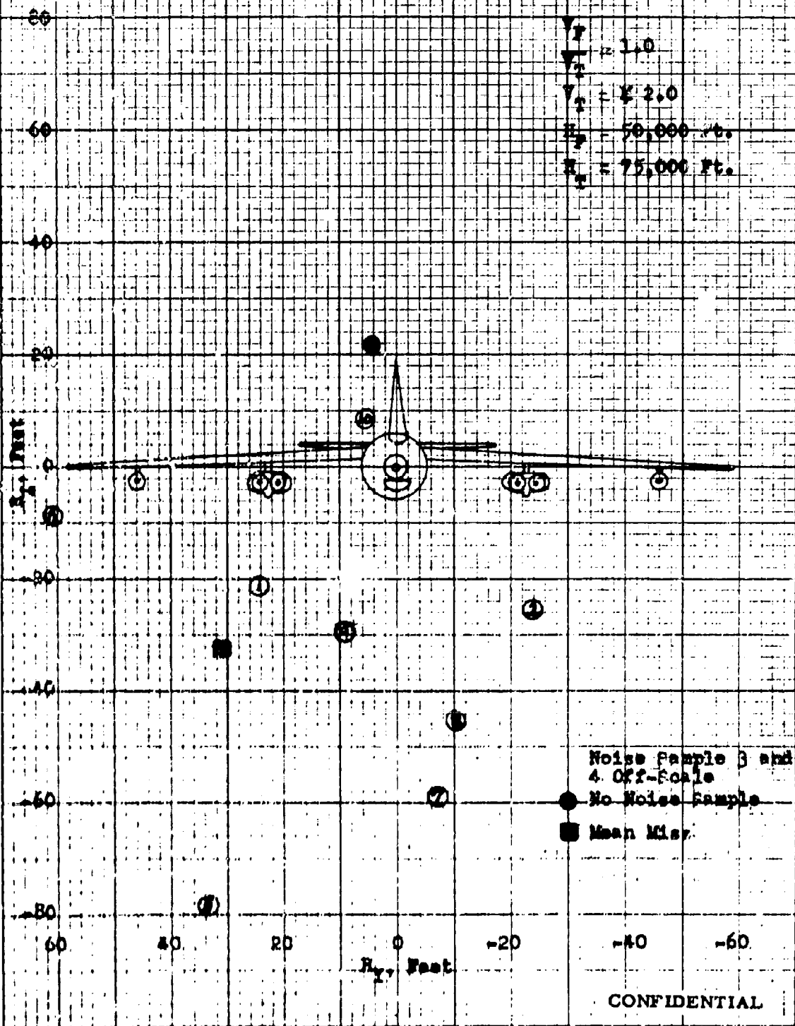
Fig. 4c - Sparrow III Miss Distance (Improved Missile) Pull-up Attacks X-Z Miss Distance at the Target \gamma_0 = 0^\circ , R_{\max} Launch, Fighter Course - D-4
