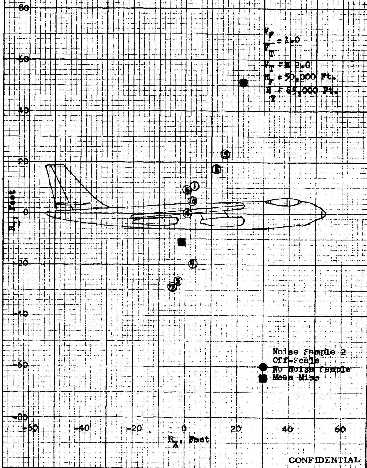
Fig. 2b - Sparrow III Miss Distance (Improved Missile) Pull-up Attacks K-2 Miss Distance at the Target \theta = 0^\circ , R_{\text{max}} Launch, Fighter Course - D-2
