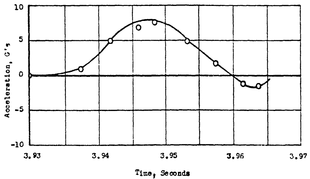
Fig. 4.8 ERA Acceleration of Structure, Site B, Shot 9
