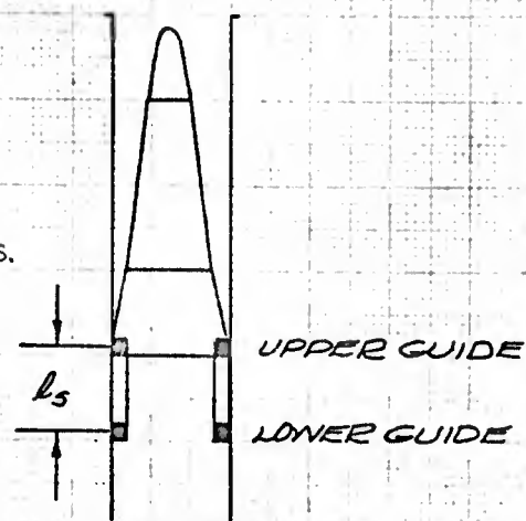
SABOT CONFIGURATION
