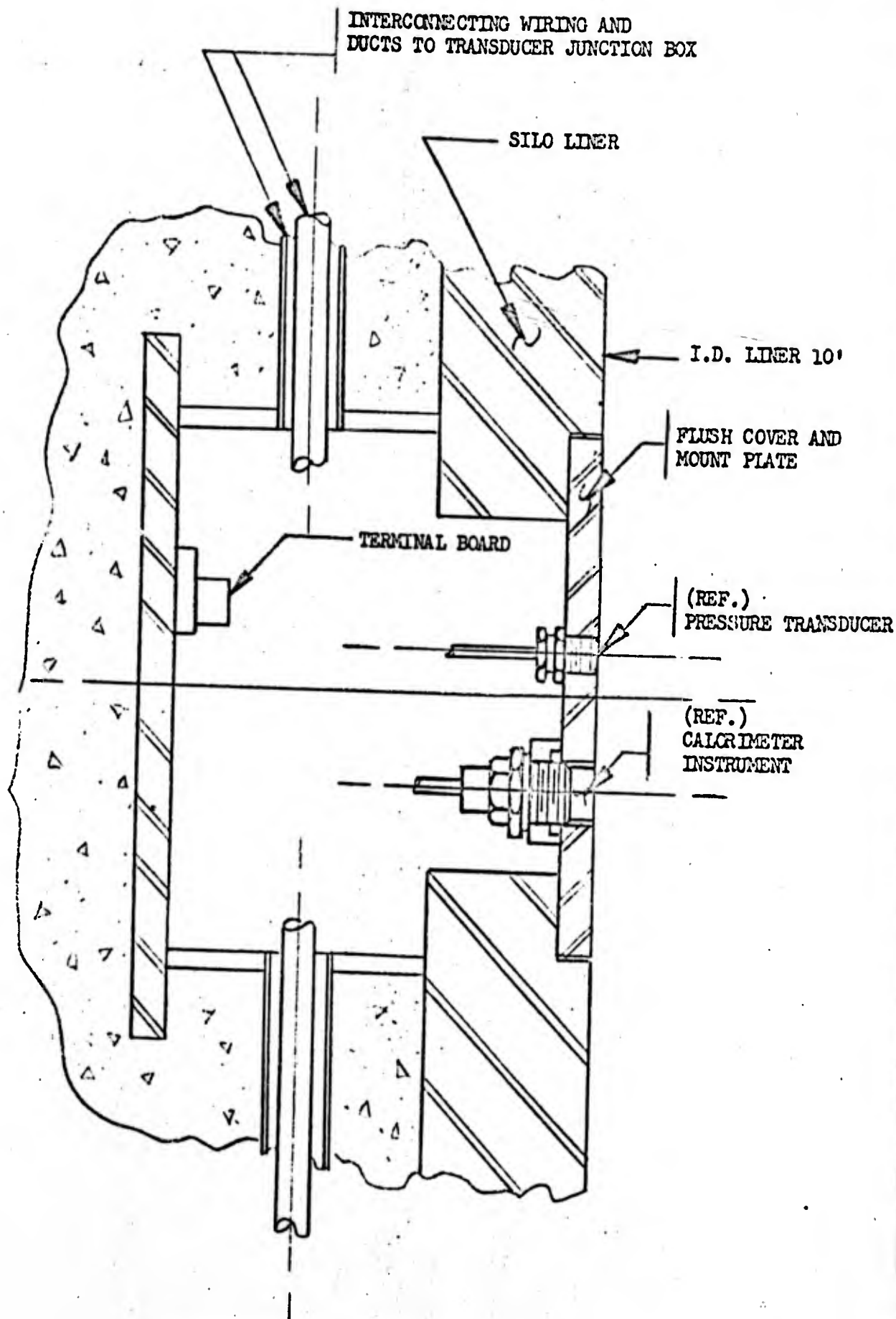
TYPICAL SILO INSTRUMENT INSTALLATION
