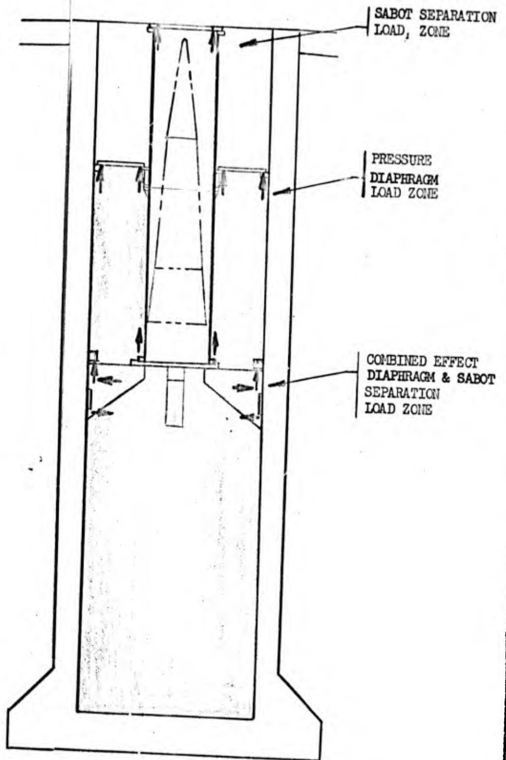
FIGURE 32 - SILO LOAD SCHEMATIC - PRESSURIZED PLENUM
