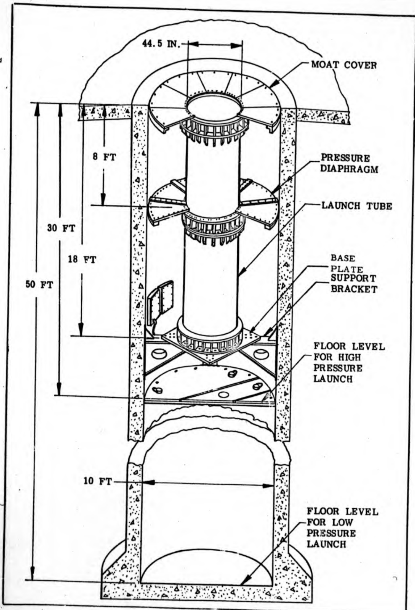
FIGURE 30 - HIBEX SILO
