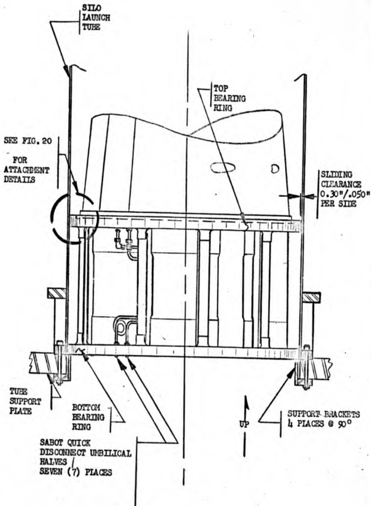
FIGURE 26 - SABOT DESIGN
