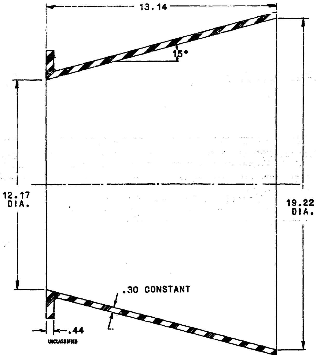
Figure 32. Demonstration V-44 ® Exit Cone Page 60
