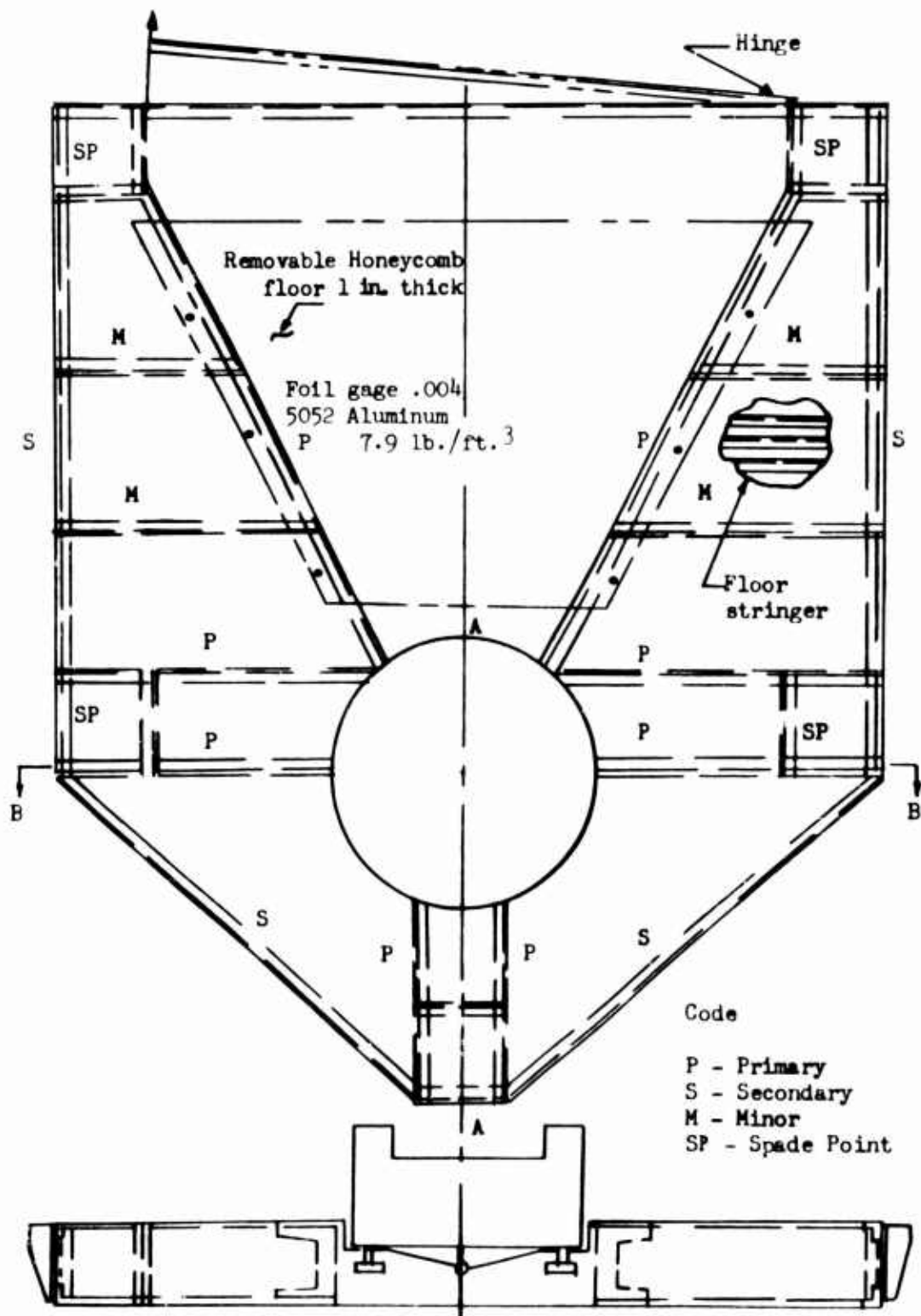
Section B B Figure 80. (U) 318-mm Rocket - Firing Platform
