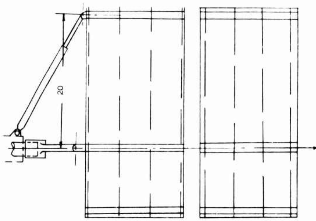
1800 1800 Figure 84. (U) Rocket Pod Support - Flight Loads
