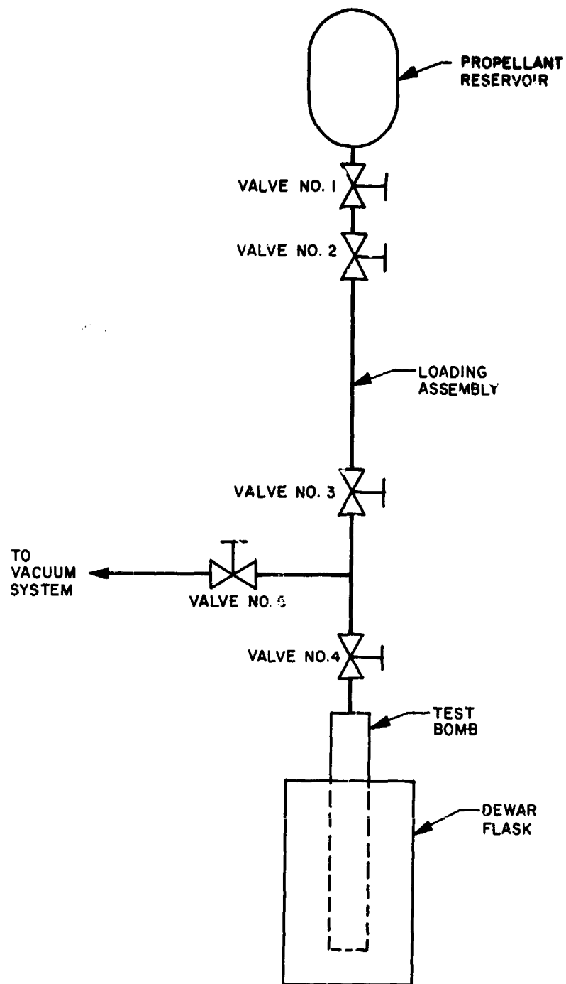
Figure 2. Loading Schematic
