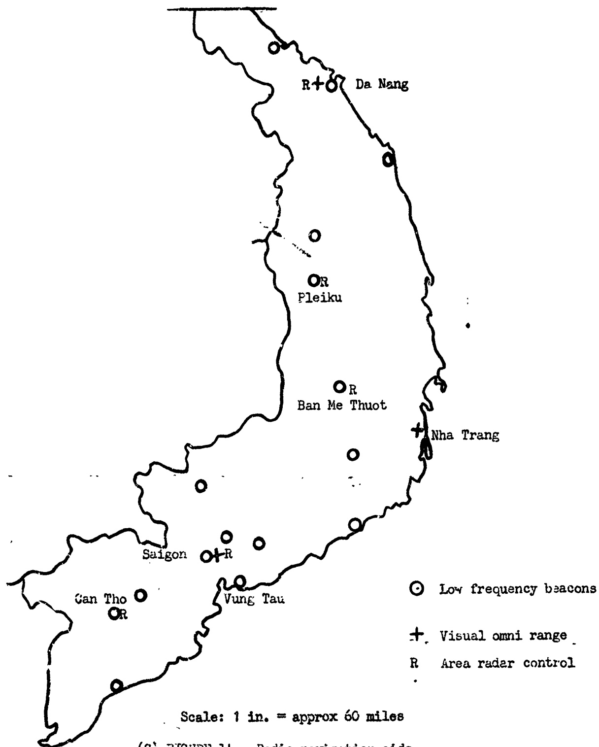
(C) FIGURE 14. Radio navigation aids.
