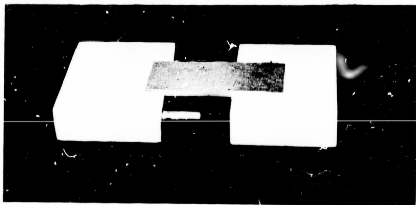
Figure 6. Remote Propellant Mold, Open
