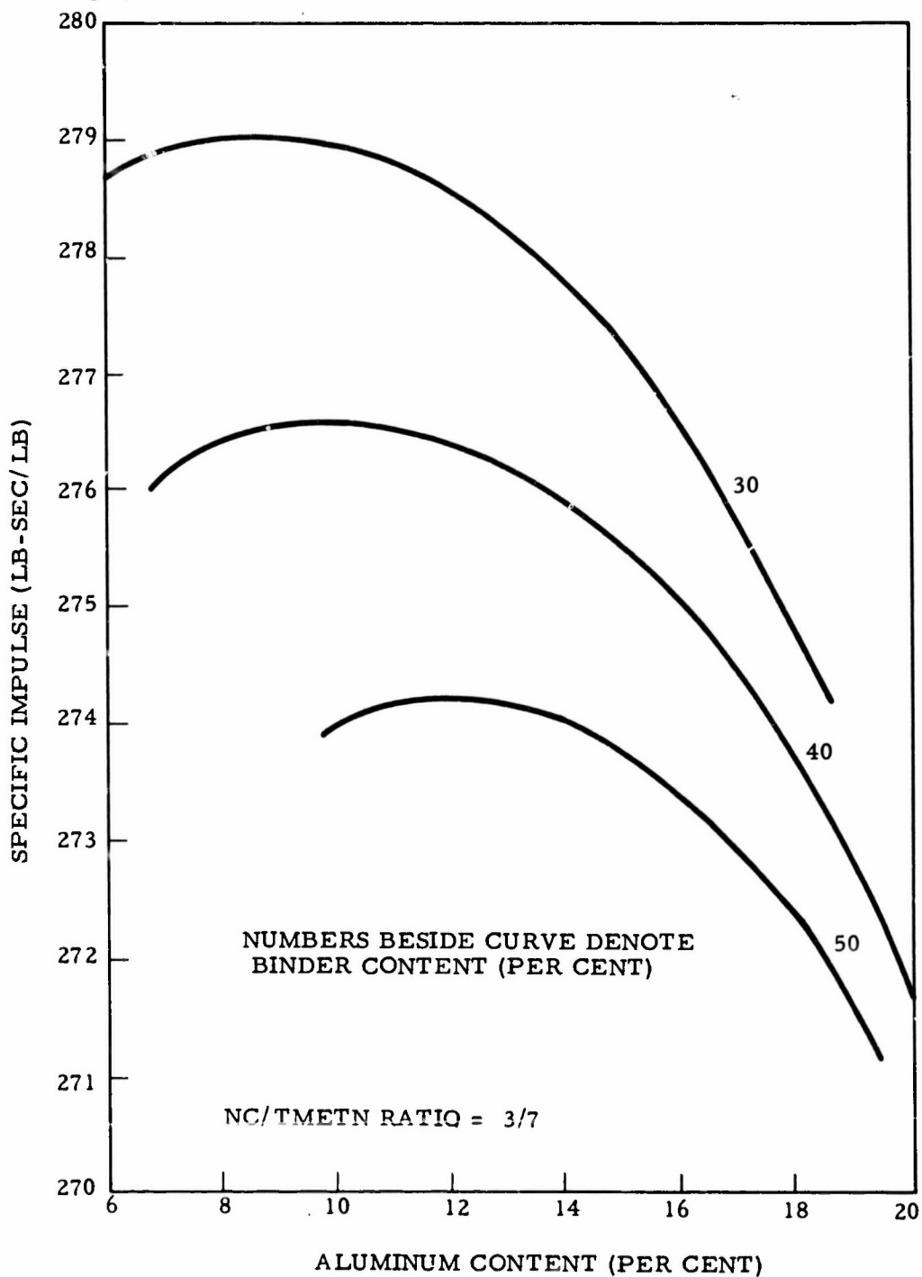
Figure 7. Theoretical Specific Impulse of Formulations Consisting of NC, TMETN, Aluminum, and INFO-635 (Reference 5)
