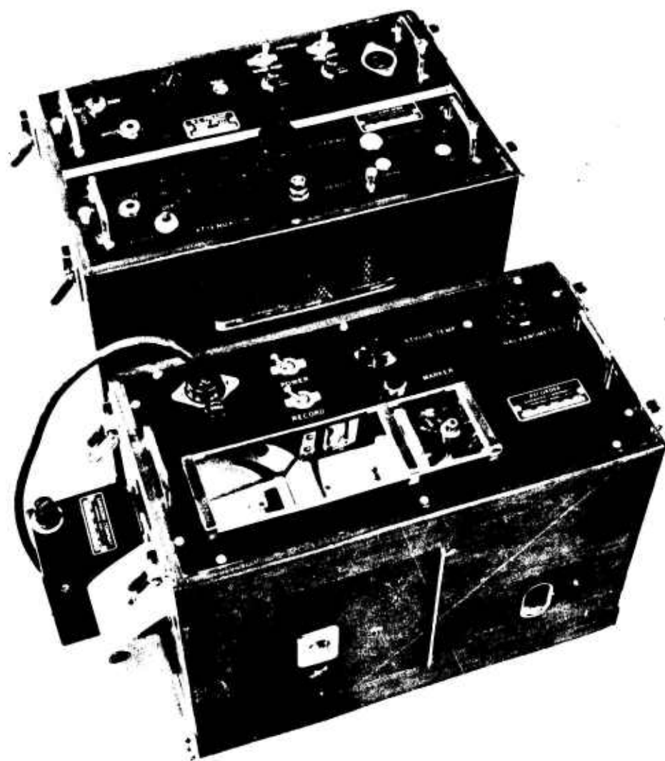
Fig. A.55 D-c Amplifier and Associated Recorder with Paper Take-up Unit
