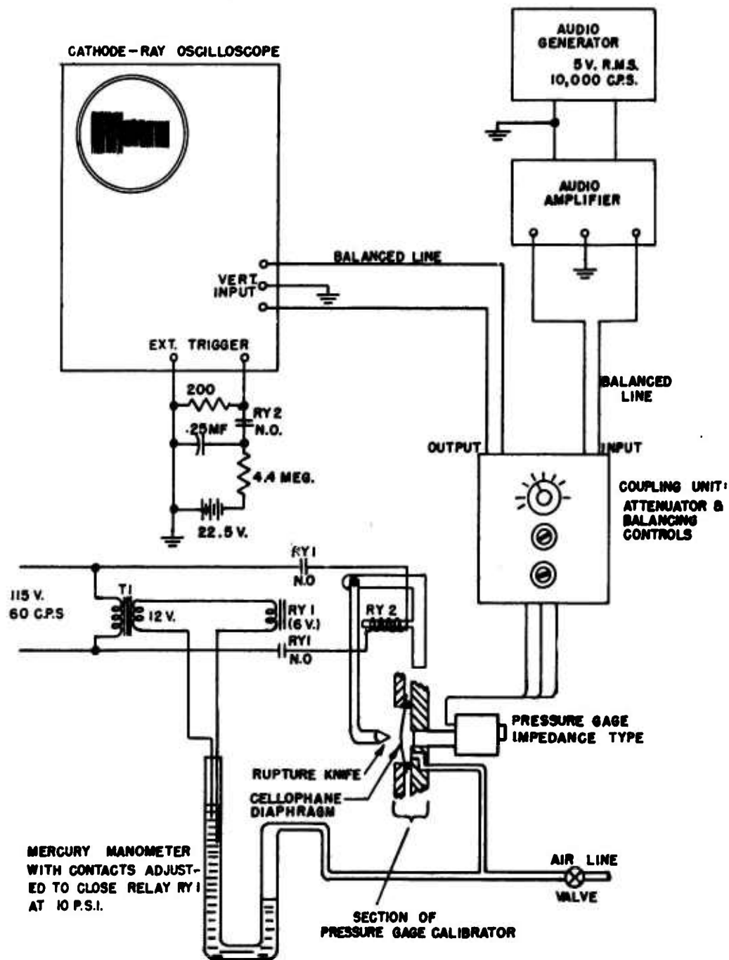
Fig. A.54 Test Arrangement for Determining Response Characteristic of Impedance Type Pressure Gauges
