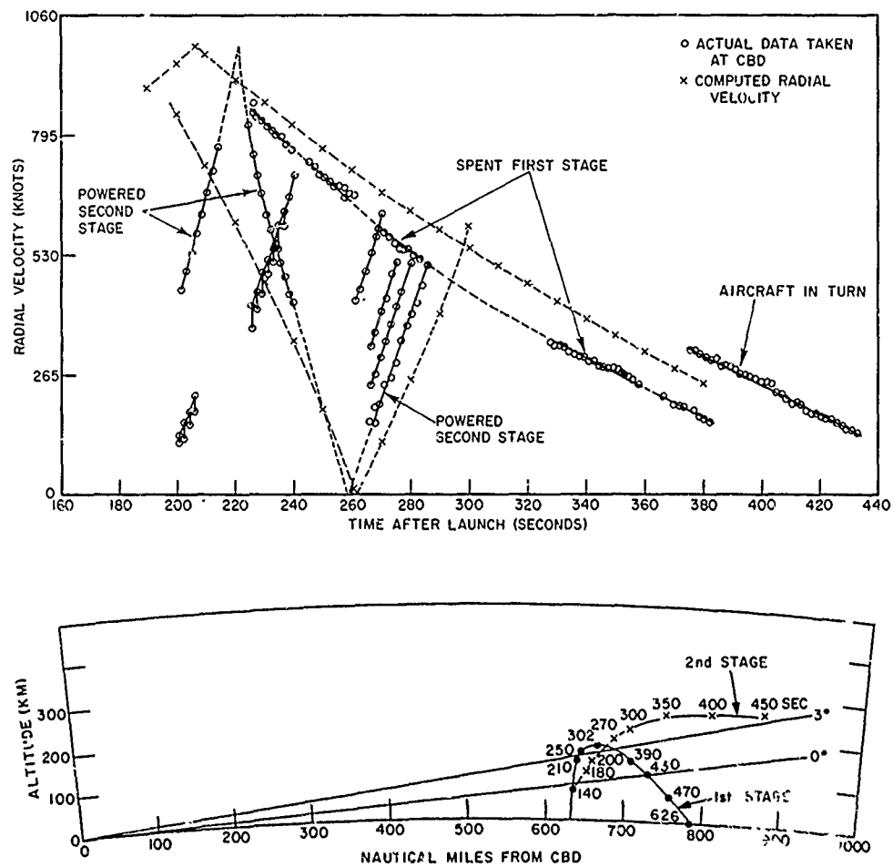
Fig. 2 - (top) Calculated velocity-time profiles of ETR Test 0169 from ETR postflight information compared with actual radar data points transcribed from Fig. 1; (Bottom) ray path diagram applicable to ETR Test 0169. Numbers on target trajectories in the bottom figure indicate the time after launch (in seconds).
