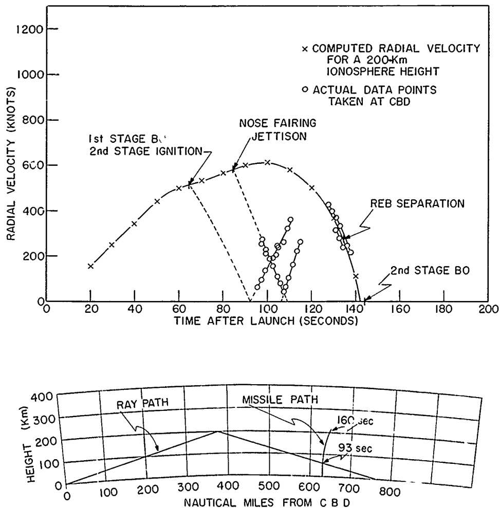
Fig. 4 - (top) Calculated velocity-time profiles of ETR Test 3670 from ETR postflight information compared with actual radar data points transcribed from Fig. 3; (bottom) signal ray path applicable to ETR Test 3670. Times shown on missile path in bottom figure indicate the time after launch.
