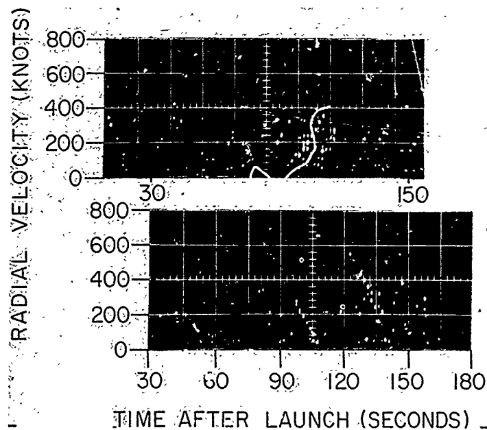
Fig. 3 - Velocity-time profiles of ETR Test 3670 (A3 Polaris launch). Upper profile is for accelerating targets; bottom profile is for decelerating targets.
