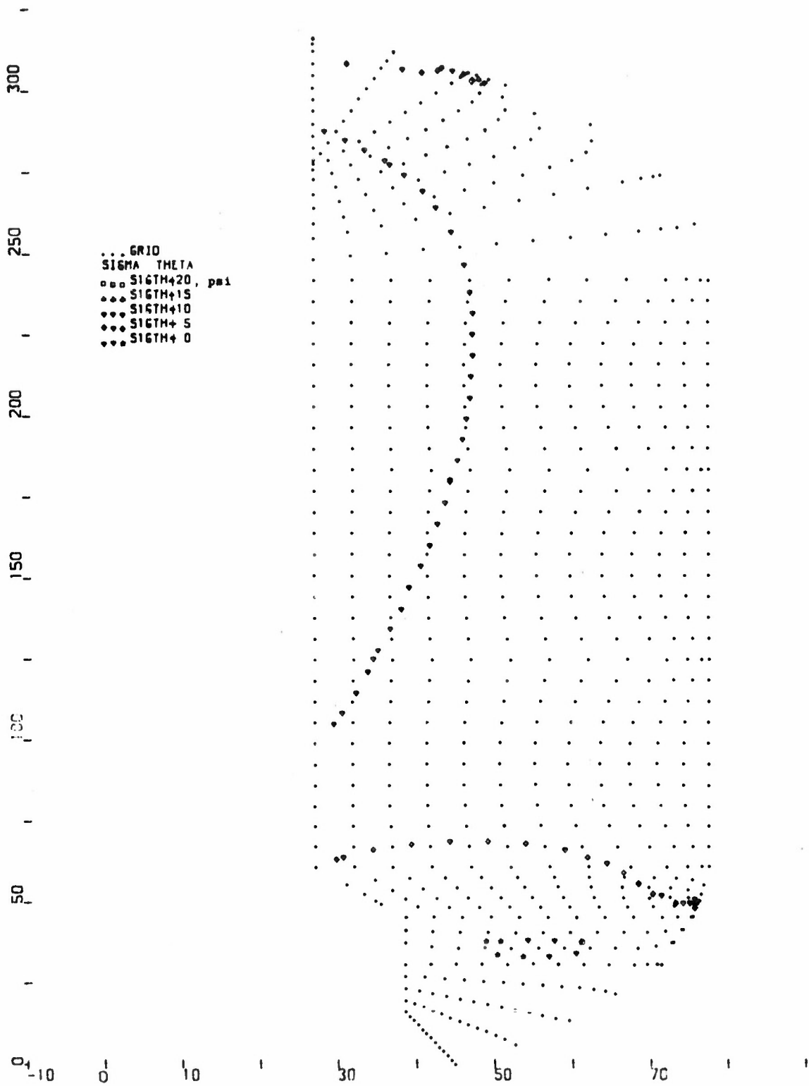
FIG 5-15. 156-9 Cure-Thermal Shrinkage Stress Analysis Tangential (Principal) Stress (Sigma Theta)
