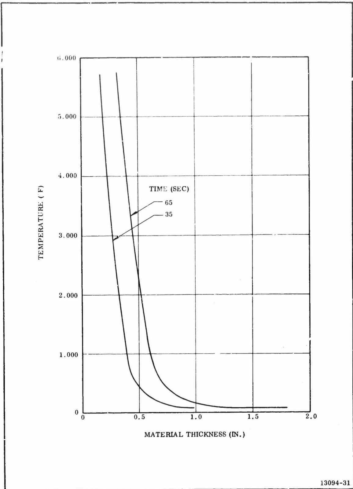
Figure 2-17. 156-9 Nozzle Entrance Temperature Profile, A/A^* = 2.52 (Back Side) Carbon Cloth
