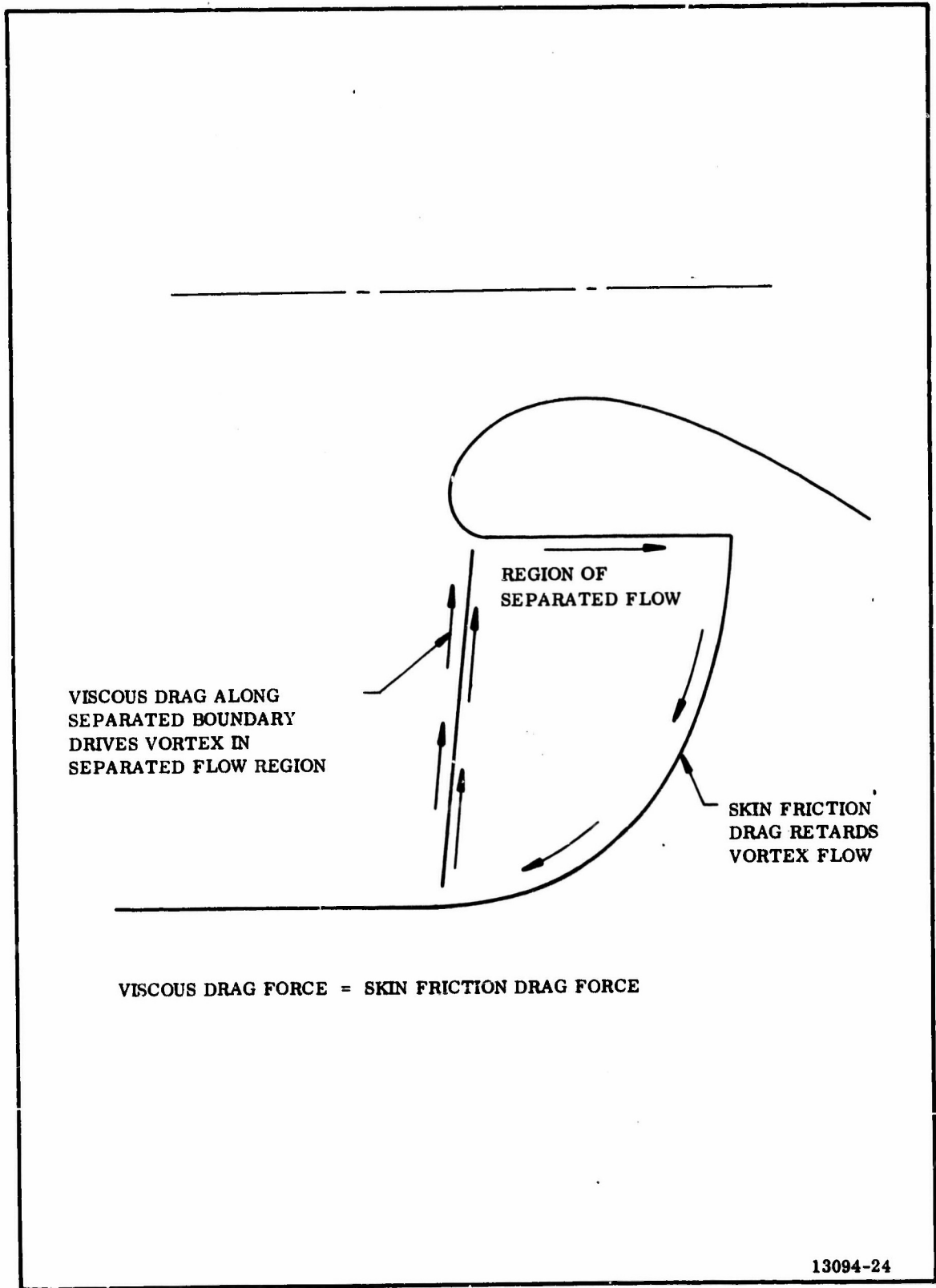
Figure 2-6. Description of Viscous and Skin Friction Drag Parameters
