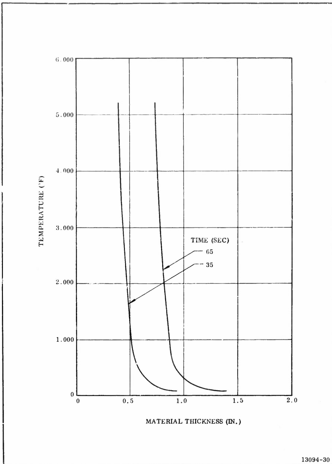
Figure 2-18. 156-9 Nozzle Entrance Temperature Profile, A/A^* = 1.17 Carbon Cloth
