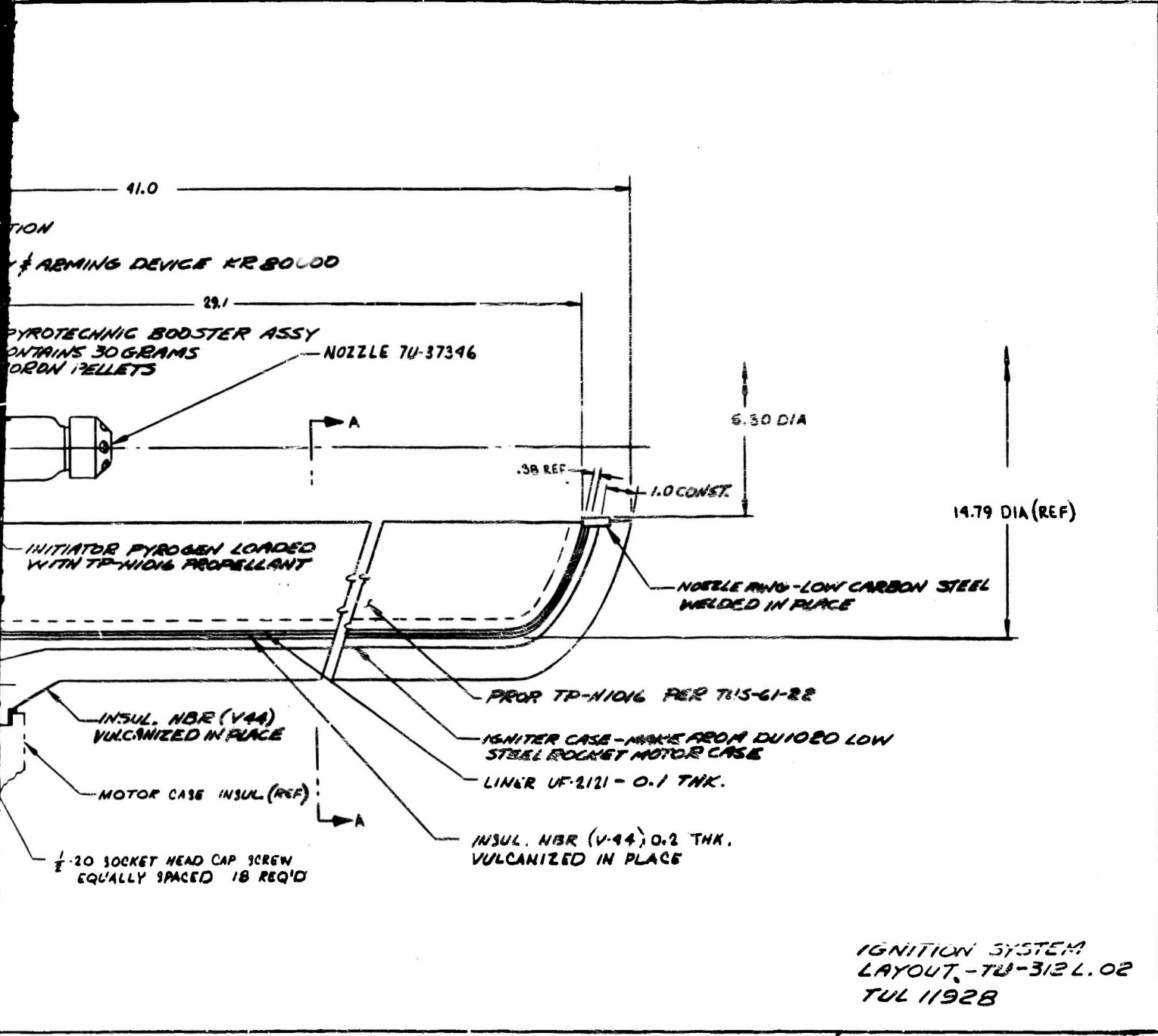
Figure 6-2. 156-8 Ignition System
