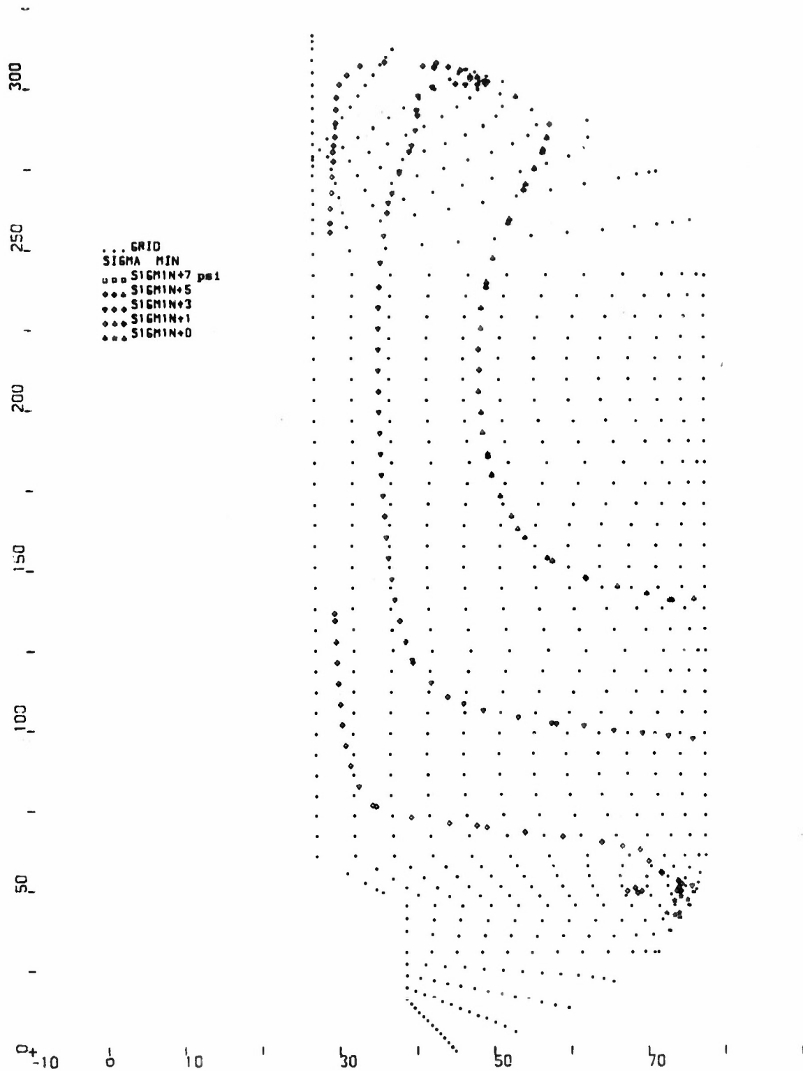
Figure 5-14. 156-9 Cure-Thermal Shrinkage Stress Analysis Minimum Principal Stress (Sigma Min)
