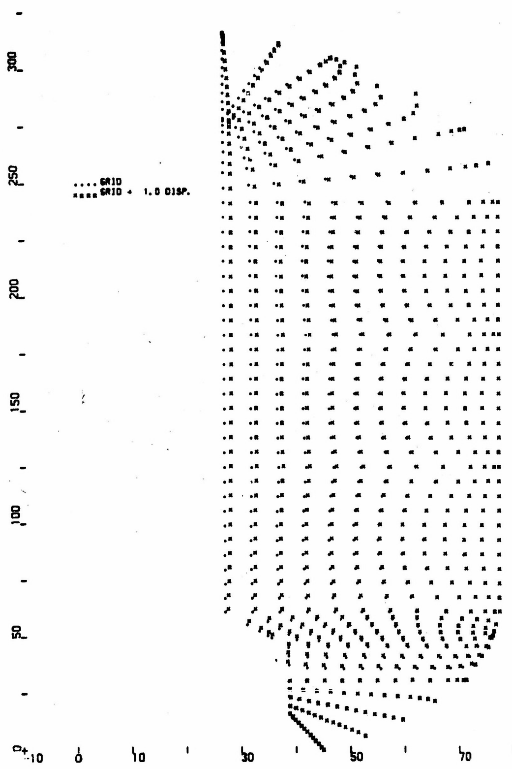
Figure 5-9. 156-9 Cure-Thermal Shrinkage Stress Analysis Grain Deformation
