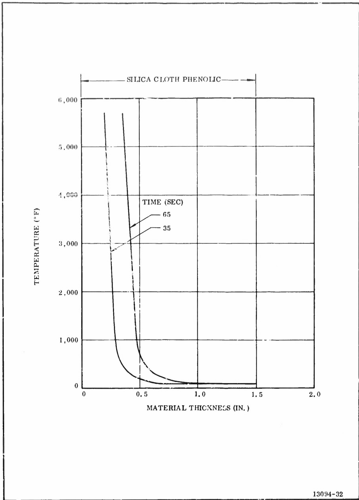
Figure 2-16. 156-9 Nozzle Entrance Temperature Profile, A/A^* = 3.88 (Backside)
