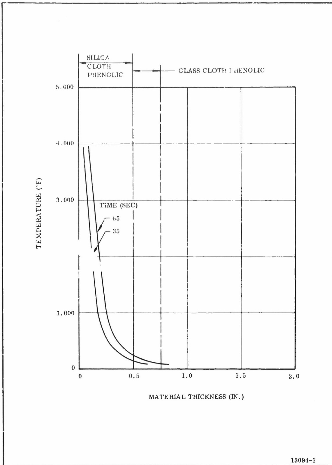
Figure 2-20. 156-9 Nozzle Exit Cone Temperature Profile, A/A^* = 8.16
