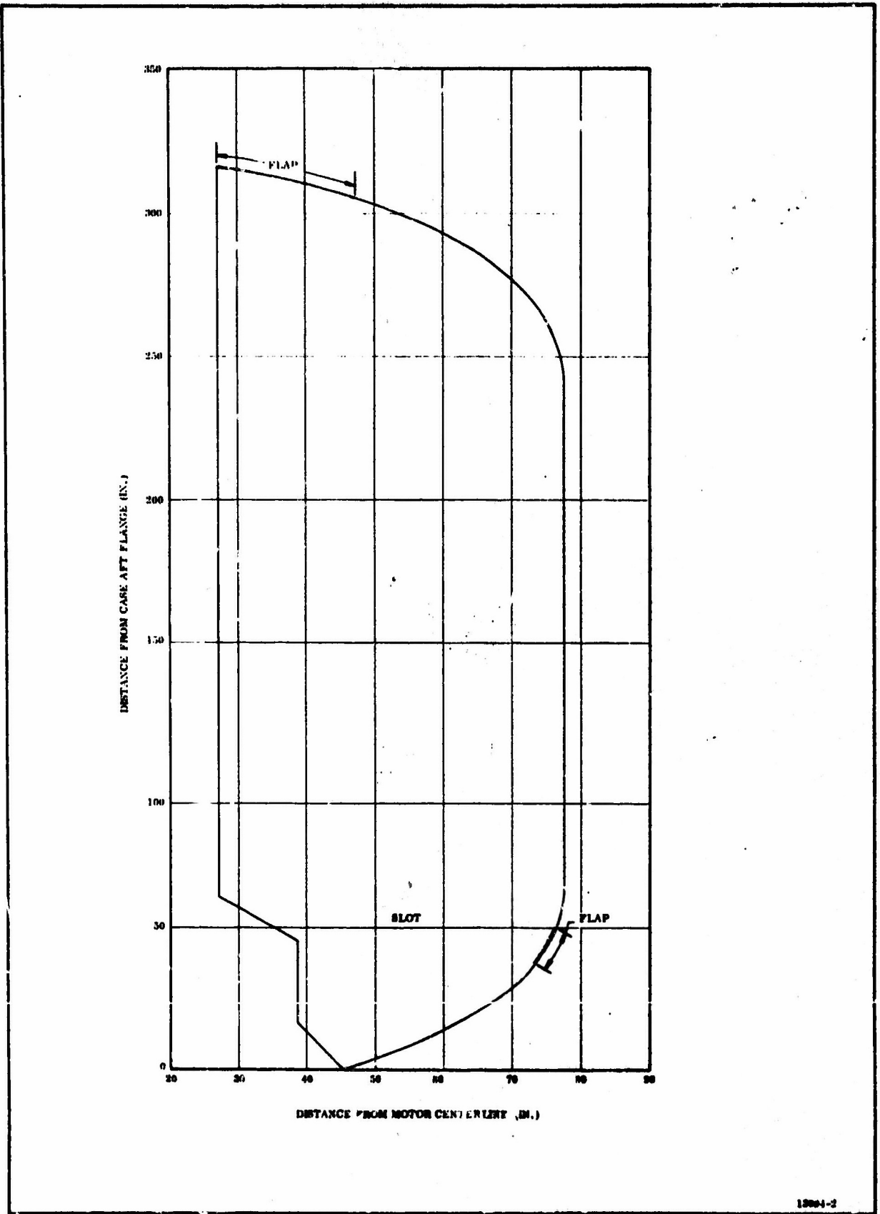
Figure 5-4. 156-9 Grain Configuration
