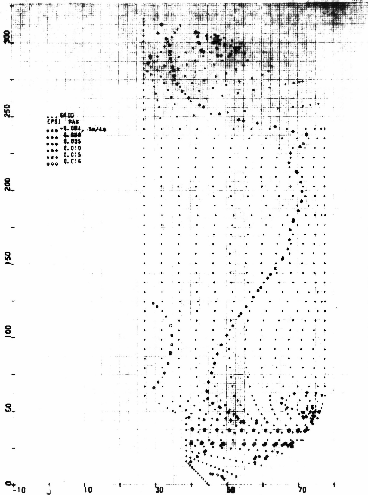
Figure 5-16. 156-9 Ignition Pressure 602 psi Stress Analysis Maximum Principal Strain (EPSI Max)
