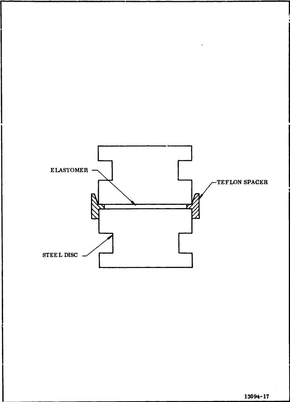
Figure 3-4. Tensile Adhesion, Steel to Steel Disc
