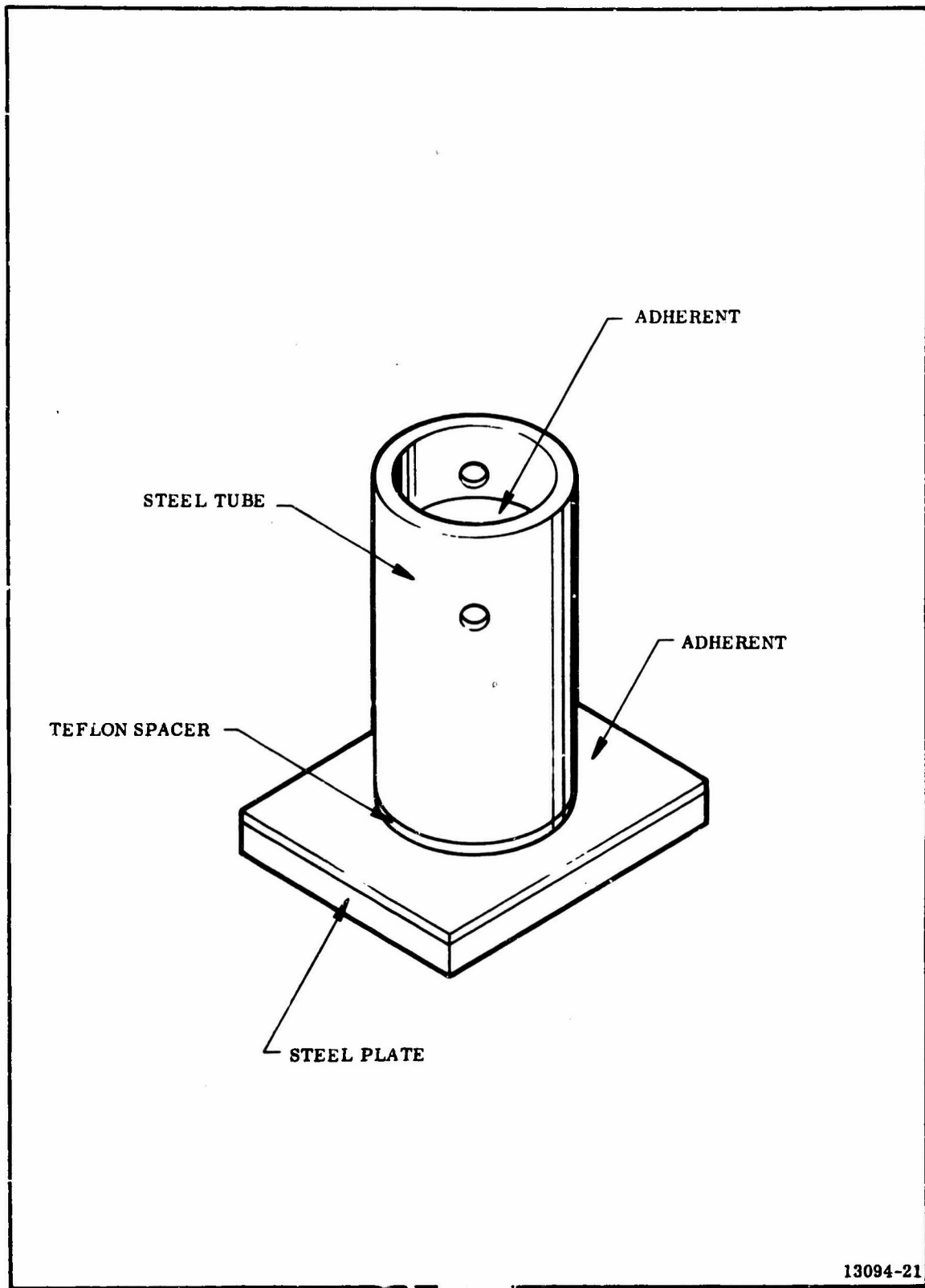
Figure 3-6. Adherent Cup Test Specimen
