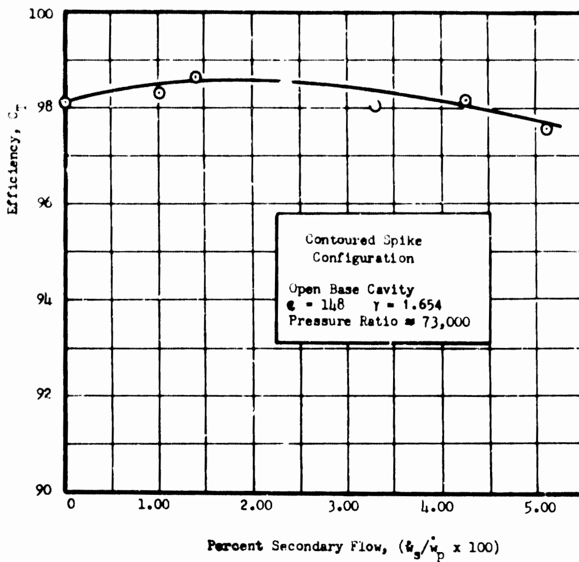
Fig. 18 Efficiency vs Secondary Flow Contoured Aerodynamic Spike Configuration
