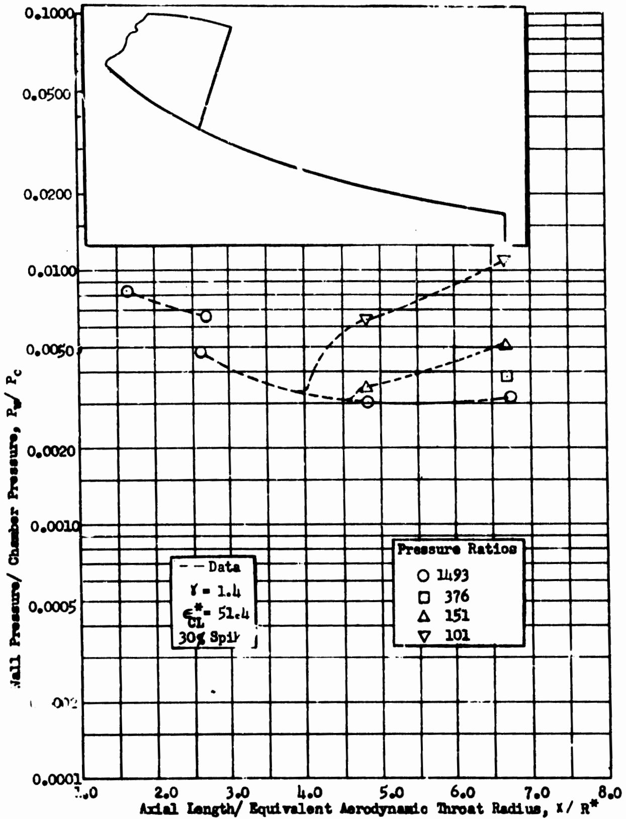
Fig. 108 Module Centerline Wall Pressure vs Axial Length, 16 Module Multichamber, 30 percent Length
