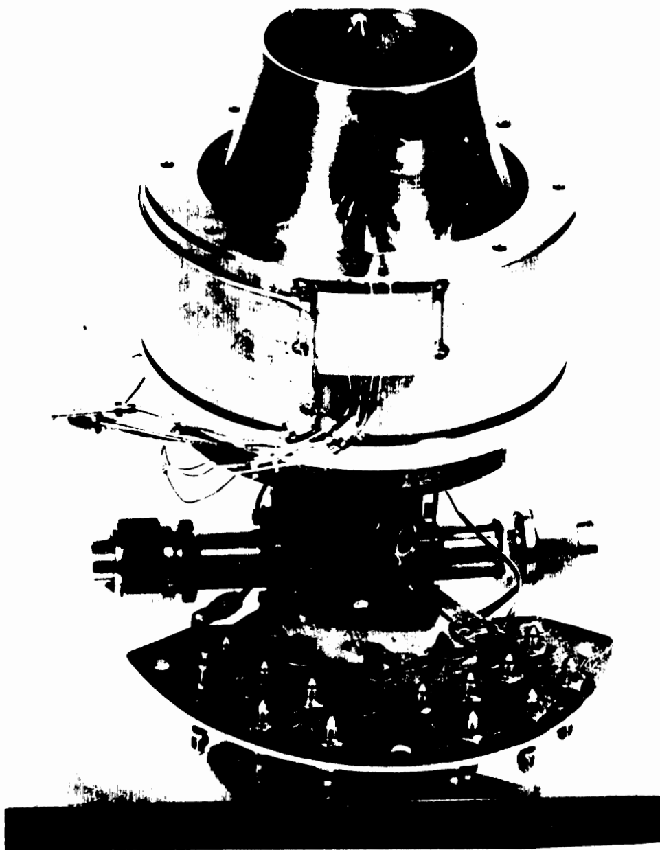
Fig. 49 Shrouded Annular Nozzle, \epsilon = 50
