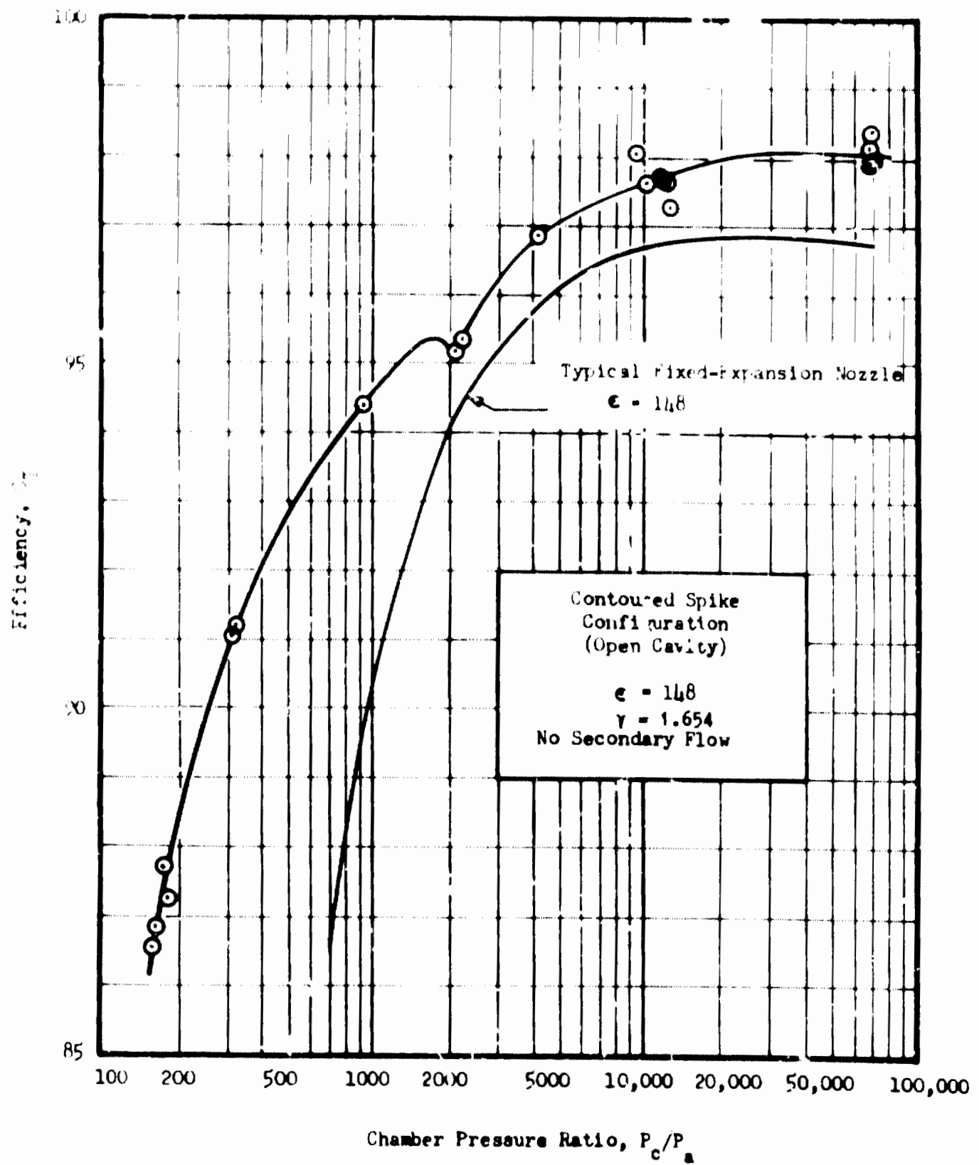
Fig. 15. Efficiency vs Chamber Pressure Ratio, Contoured Aerodynamic Spike Nozzle
