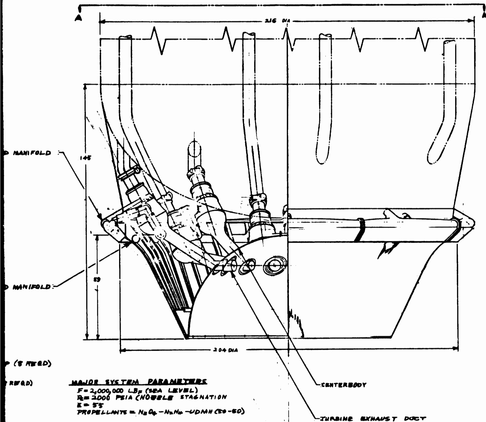
Fig. 171 Toroidal Aerodynamic Spike Engine System. High Thrust, High Chamber Pressure.
