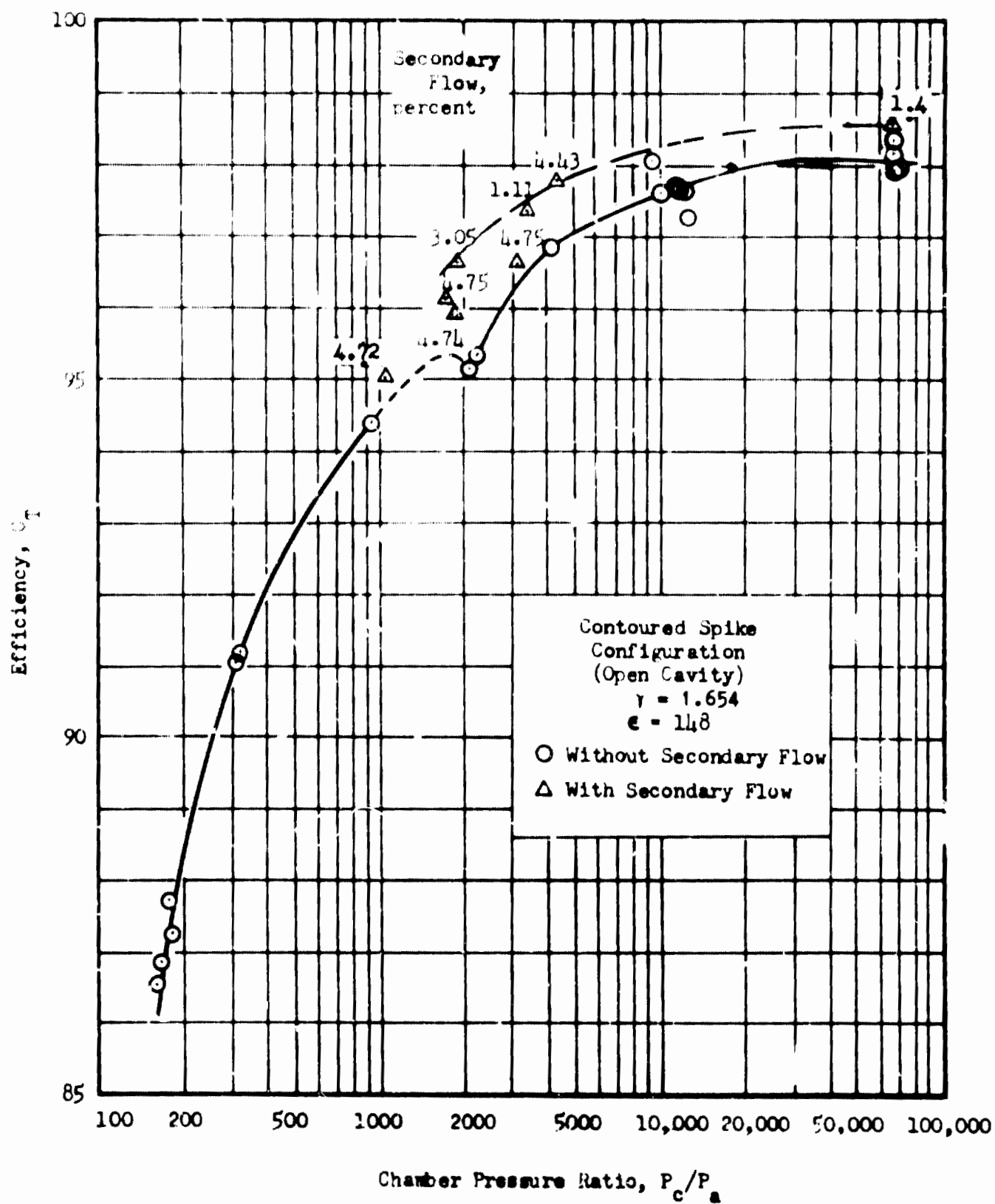
Fig. 20. Efficiency vs Chamber Pressure Ratio Contoured Aerodynamic Spike Nozzle
