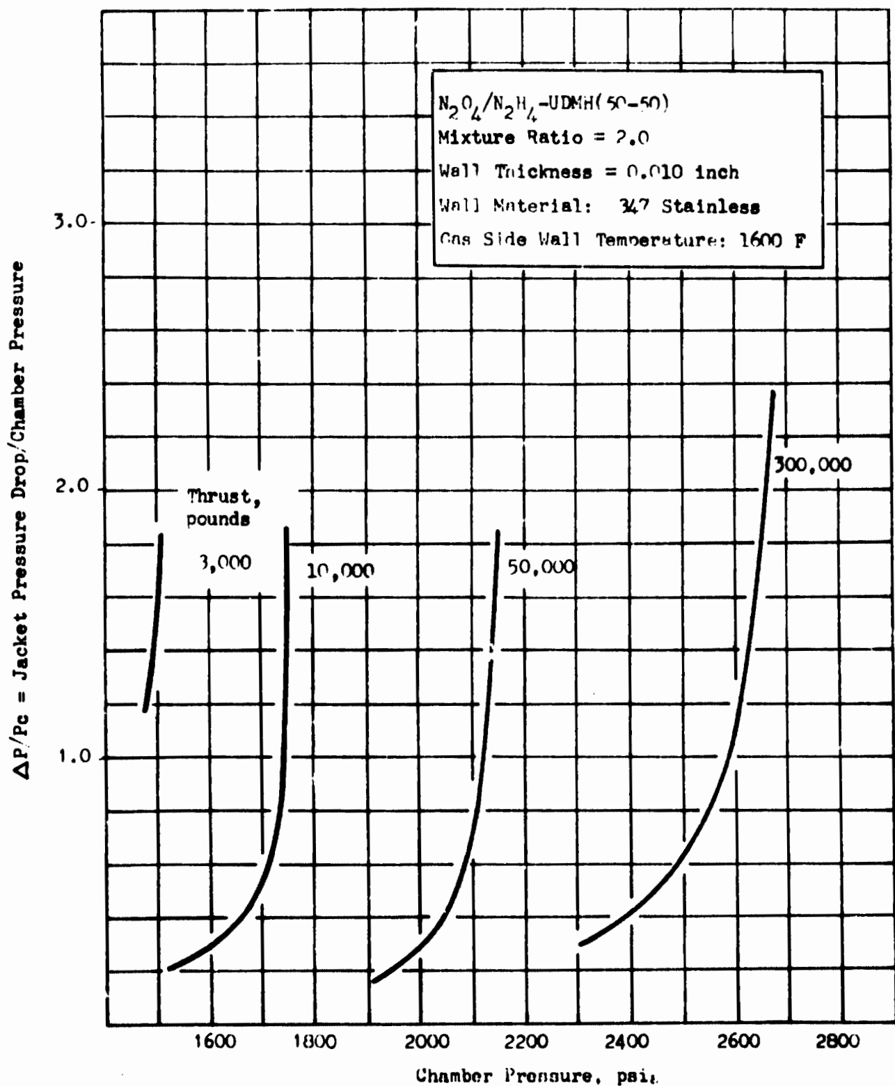
Fig.144. Tube Bundle Pressure Drop vs Chamber Pressure for Bell Thrust Chamber Using N_2O_4 Coolant
