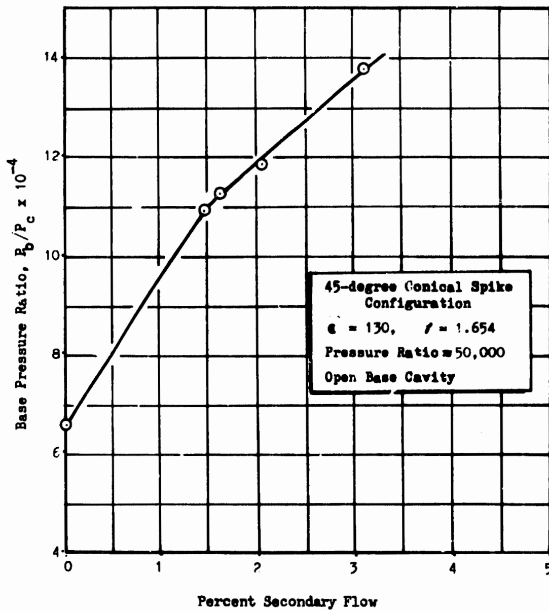
Fig. 36. Base Pressure Ratio vs Secondary Flowrate, 45-degree Aerodynamic Spike
