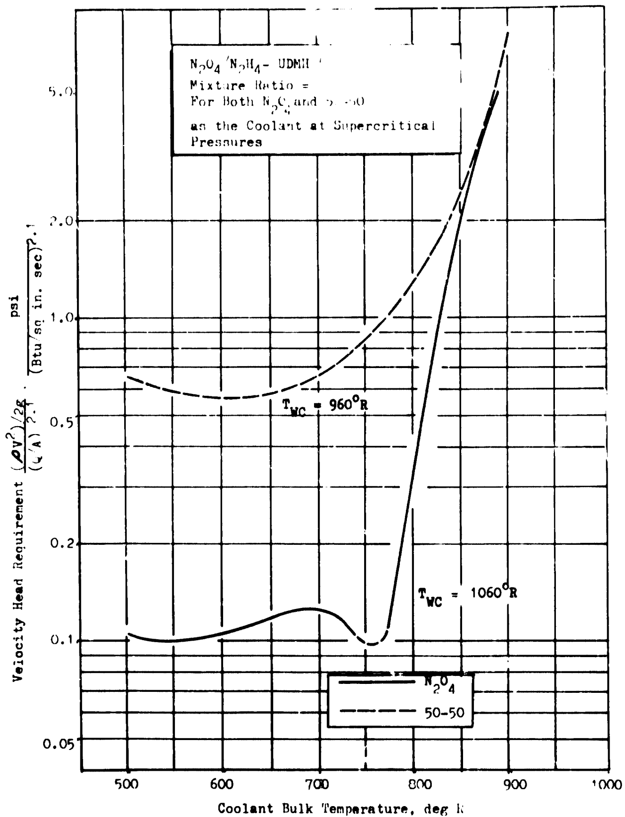
Fig. 141 Coolant Velocity Head Requirements vs Coolant Bulk Temperature and Wall Temperature
