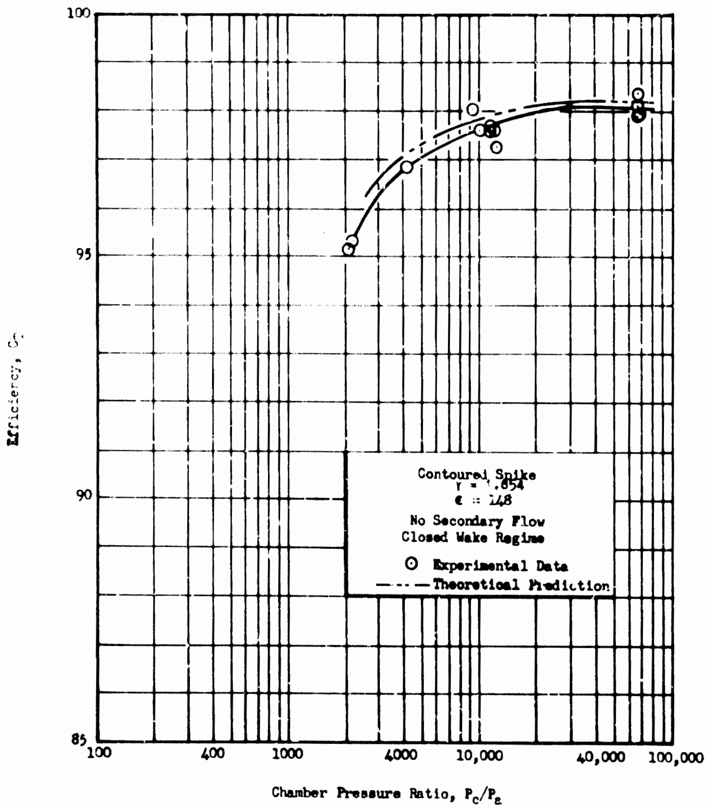
Fig. 22a Experimental and Theoretical Efficiencies of Contoured Model versus Pressure Ratio, Closed Wake Regime
