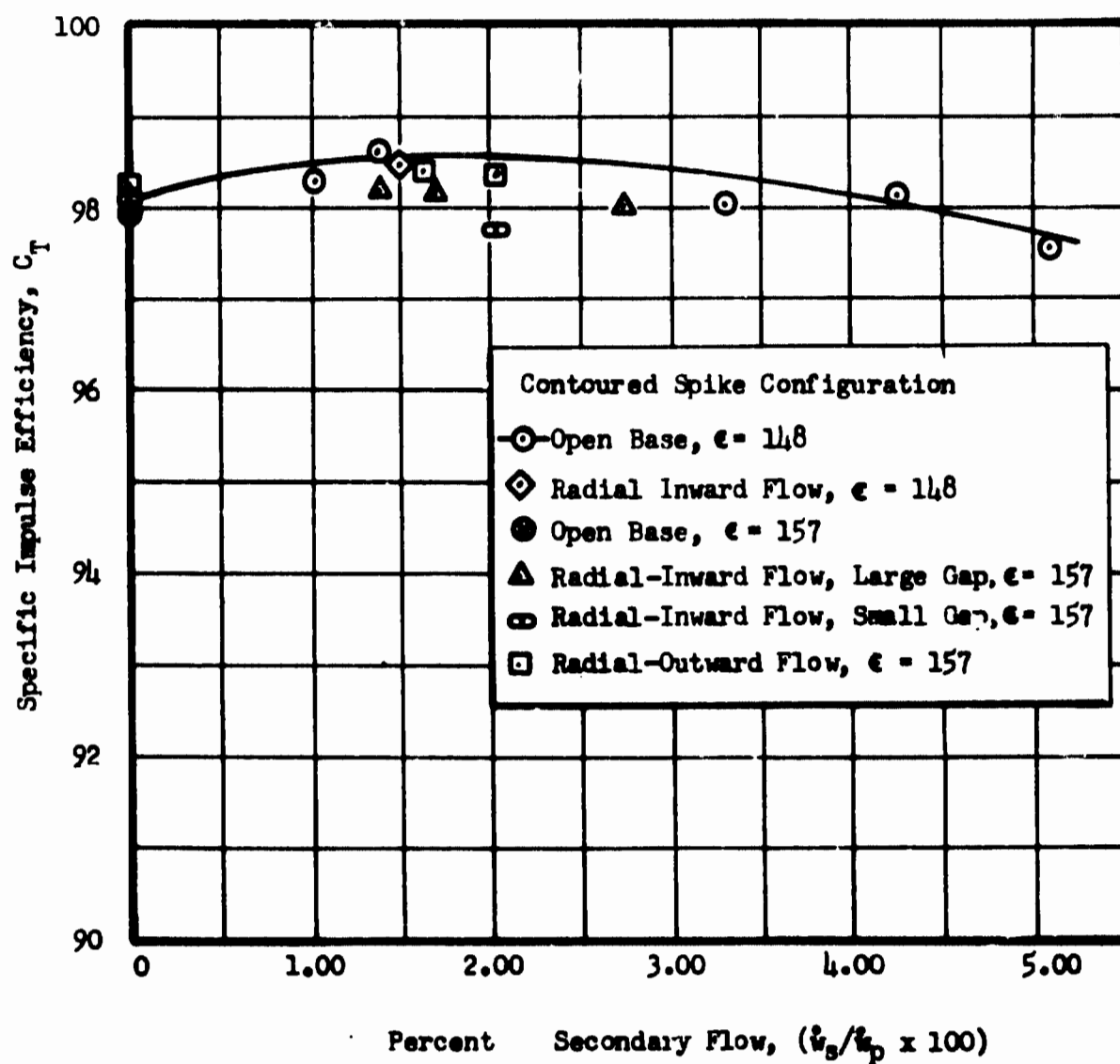
Fig. 32. Specific Impulse Efficiency vs Secondary Flow, Contoured Aerodynamic Spike Configuration, Pressure Ratio \approx 57,000 .
