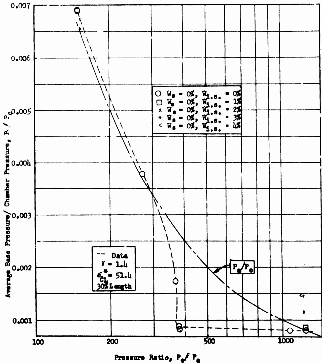
Fig. 111 Base Pressure vs Pressure Ratio, 16 Module Multichamber with Intersegmental Filler Plate
