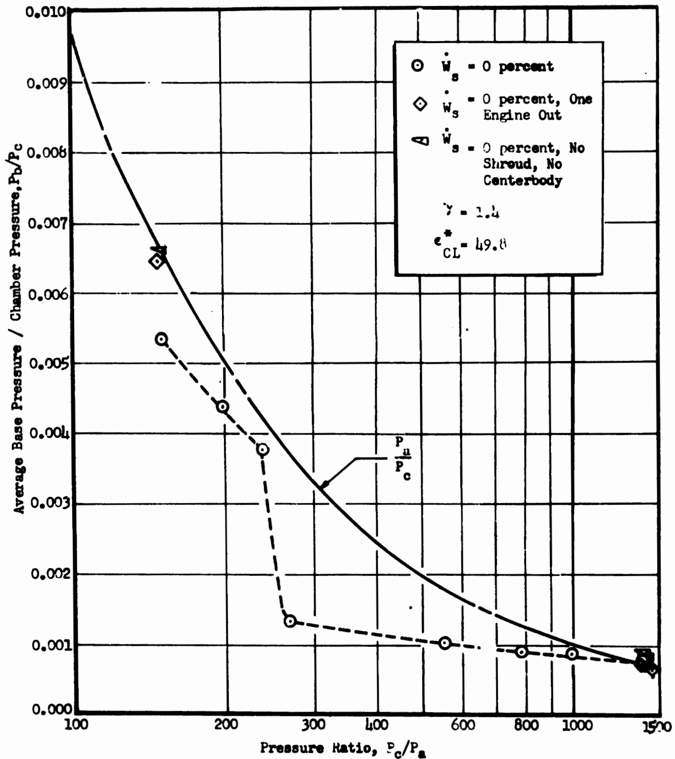
Figure 84 . Base Pressure vs Pressure Ratio, 8 Module Touching Multichamber, No Spike
