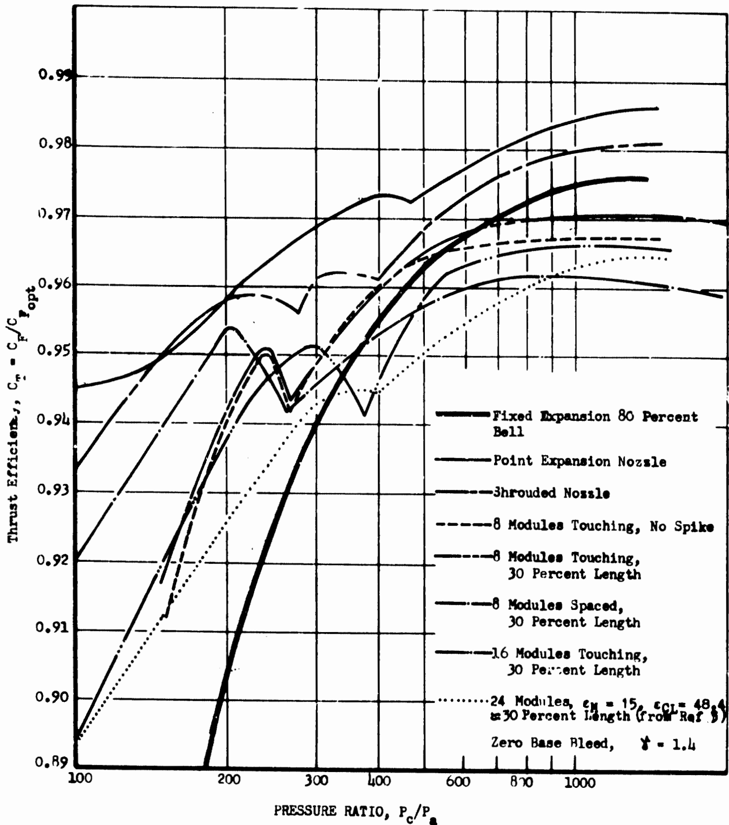
Figure 112 Comparison of Experimental Performance of \epsilon_{CL} = 50 Annular and Multichamber Nozzles
