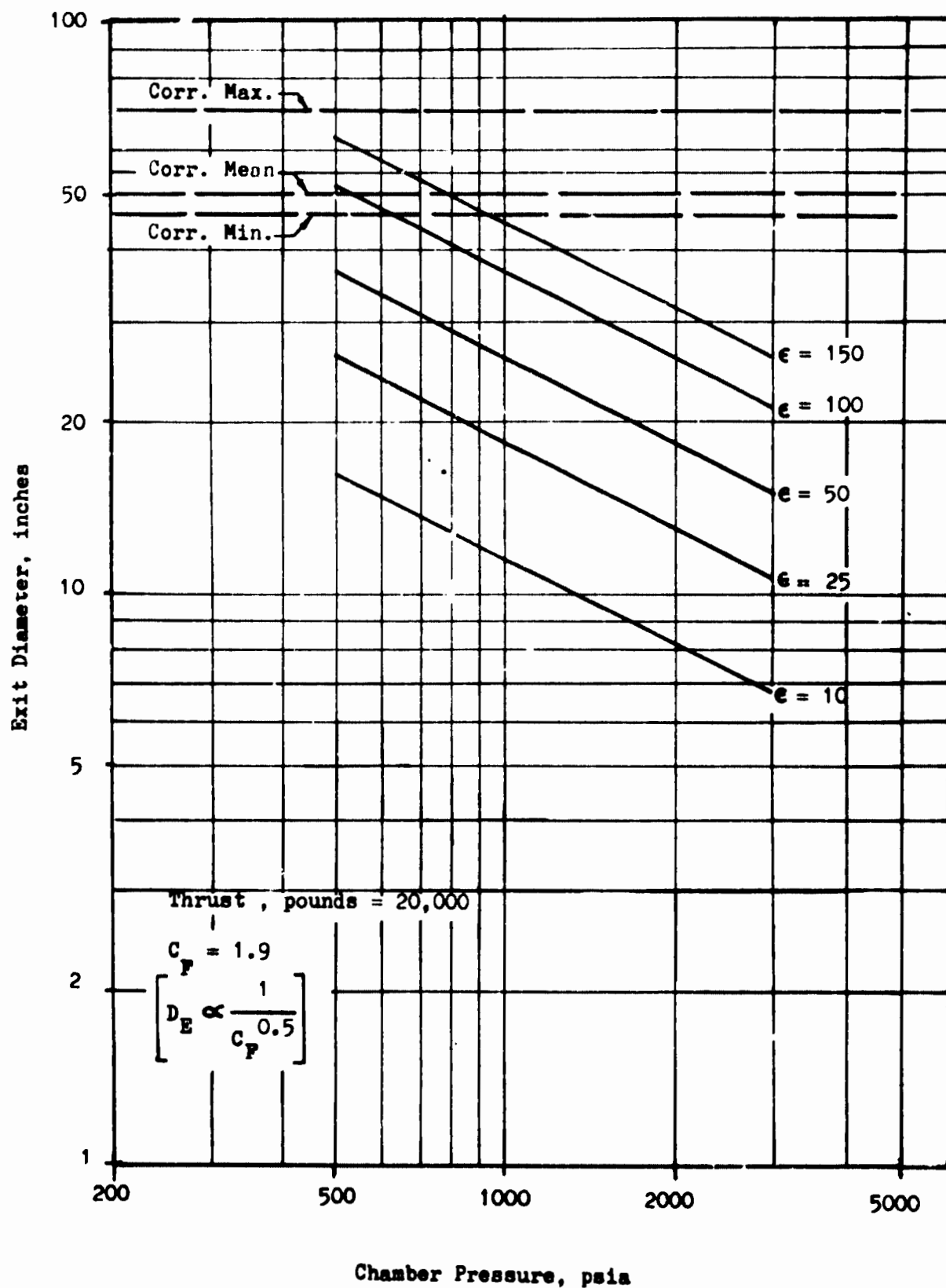
Fig.121 Toroidal Engine Envelope( F = 20,000 pounds)
