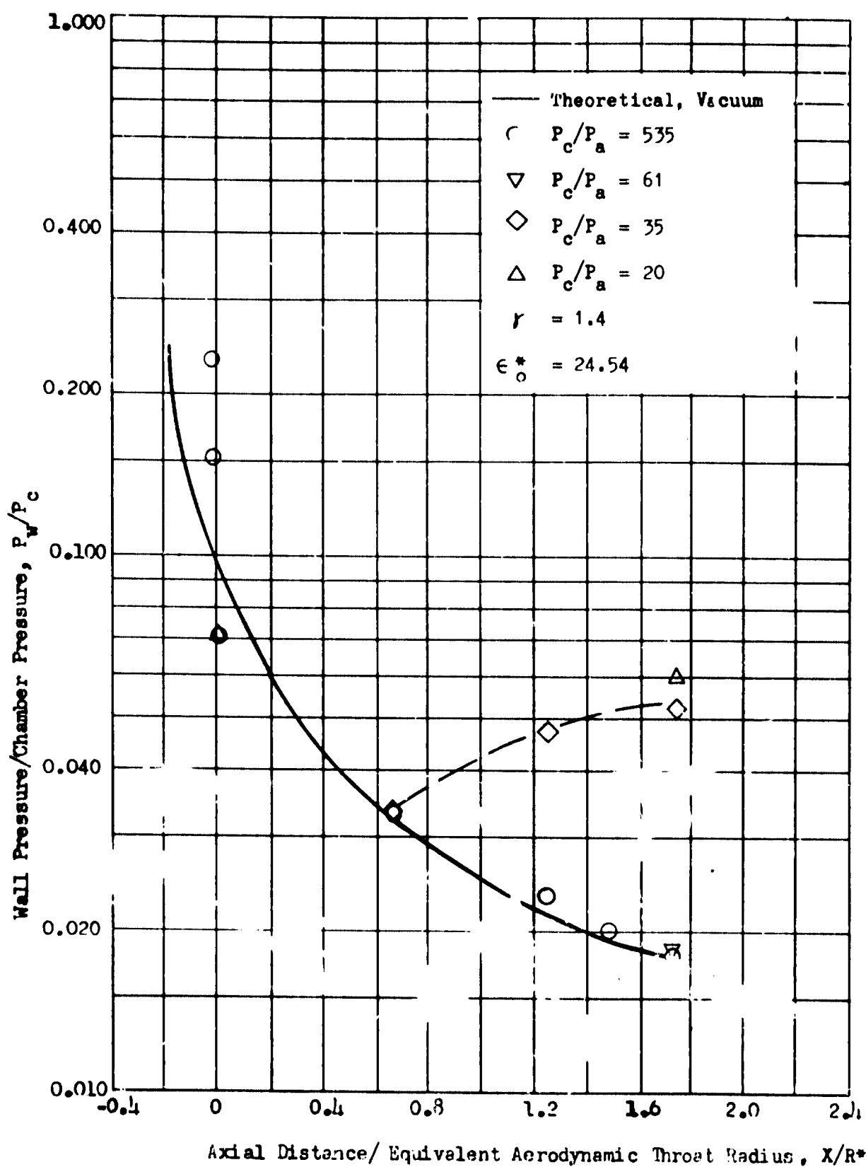
Fig. 62. Wall Pressure Profile for Scaled Hot-Firing Model. \dot{w}_s = 0
