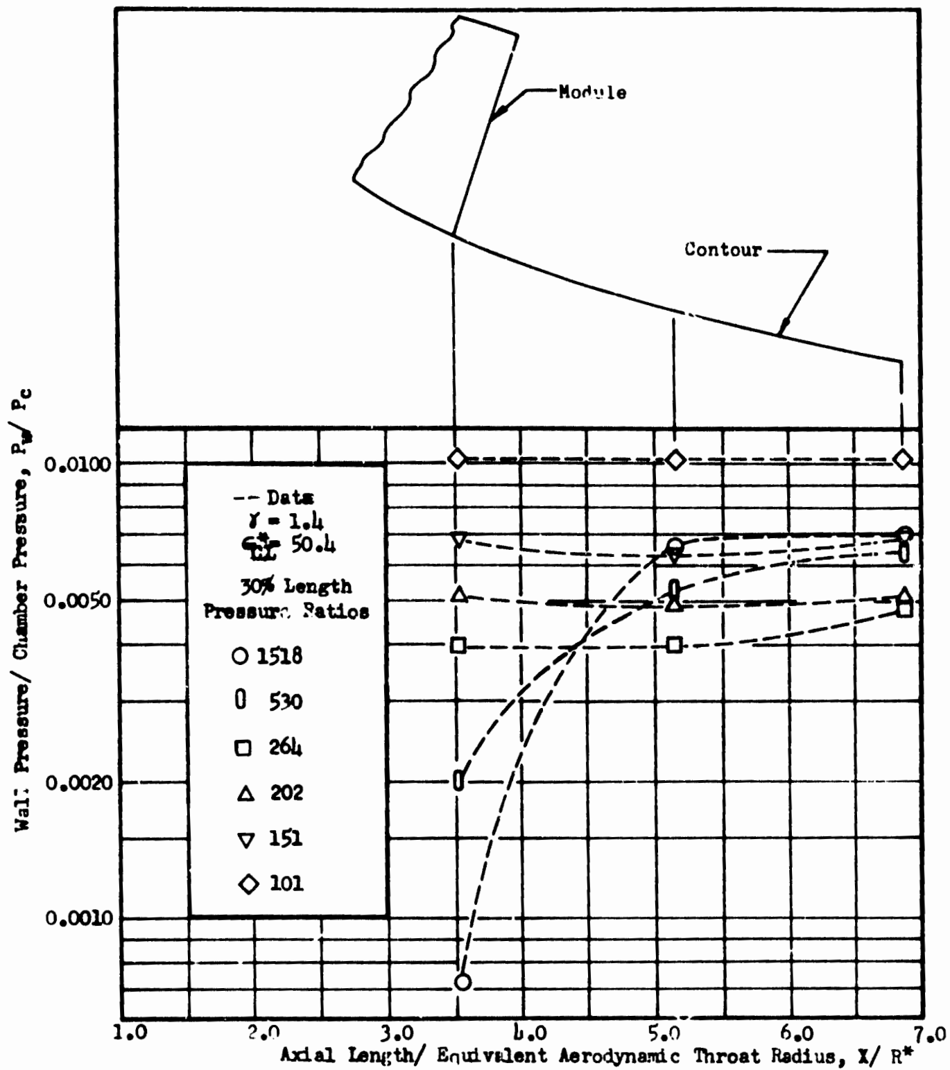
Fig. 102 Wall Pressure Profile Between Modules vs Axial Distance, 8 Module Spaced Multichamber, 30 Percent Length
