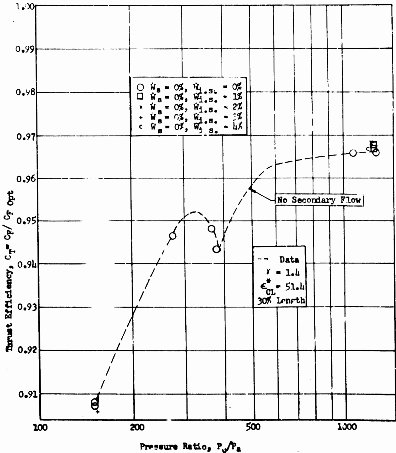
Fig. 110 Thrust Efficiency vs Pressure Ratio, 16 Module Multichamber with Intersegmental Filler Plate
