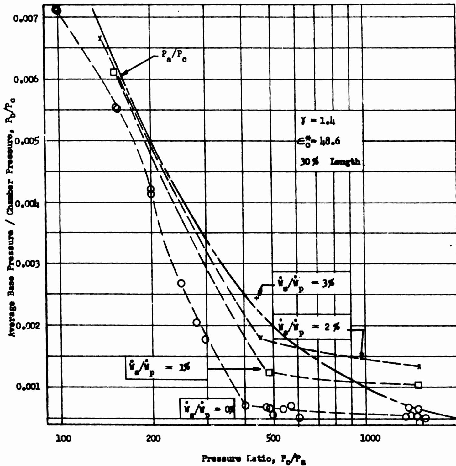
Fig. 77 Base Pressure vs Pressure Ratio for Shrouded Spike Nozzle
