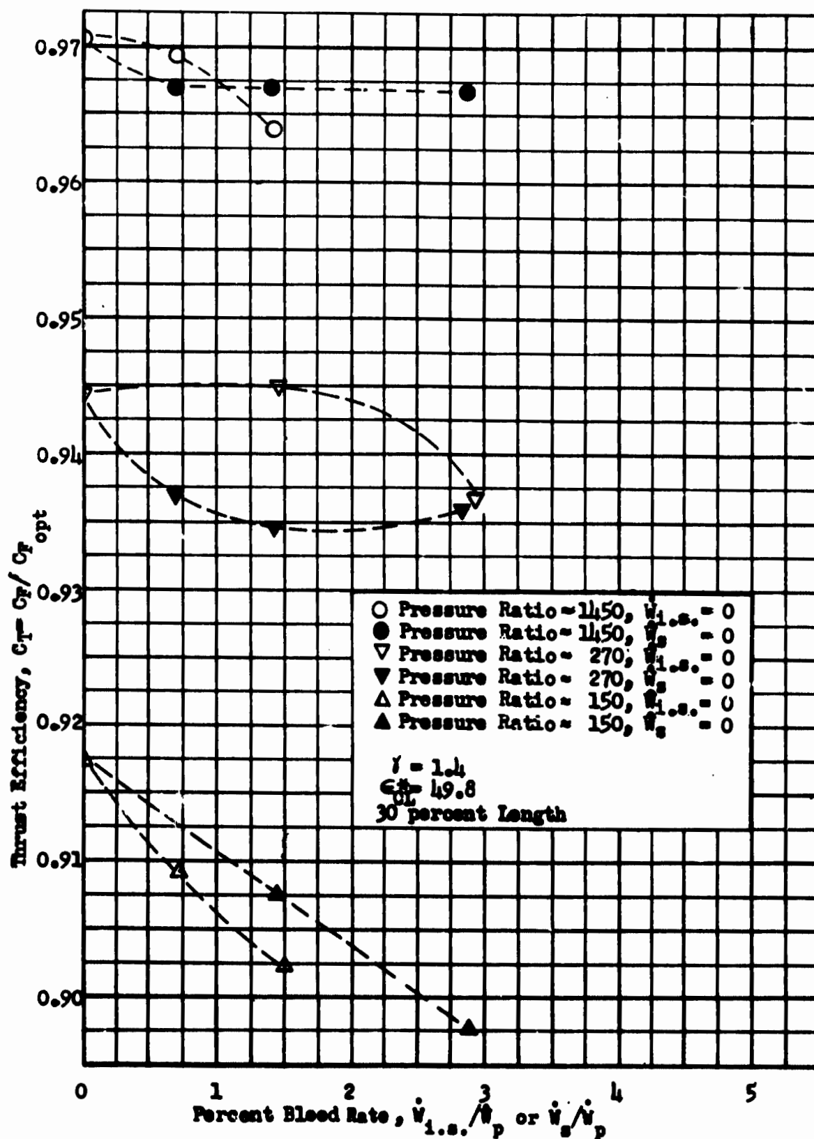
Fig. 89 Thrust Efficiency vs Bleed Rate, 8 Module Touching Multichamber, 30 percent Length
