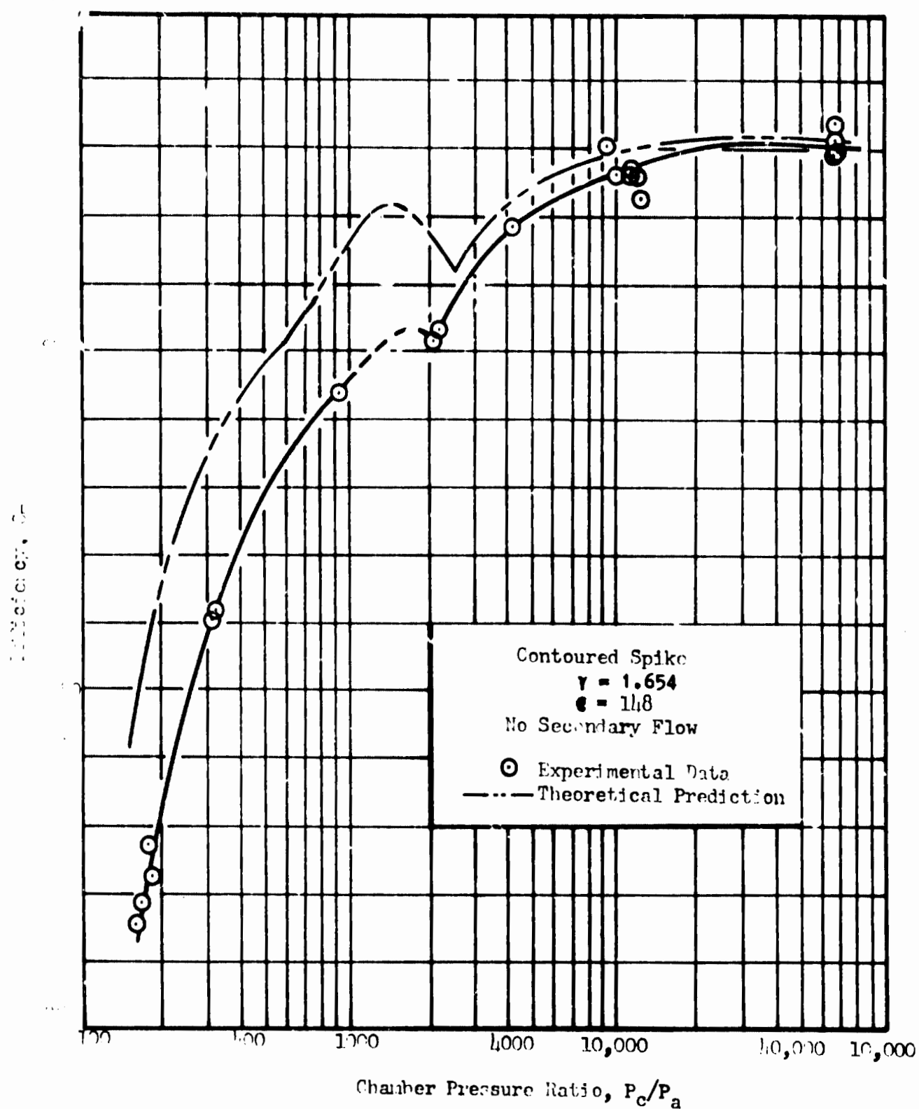
Fig. 26. Experimental and Theoretical Efficiencies of Contoured Model Versus Pressure Ratio
