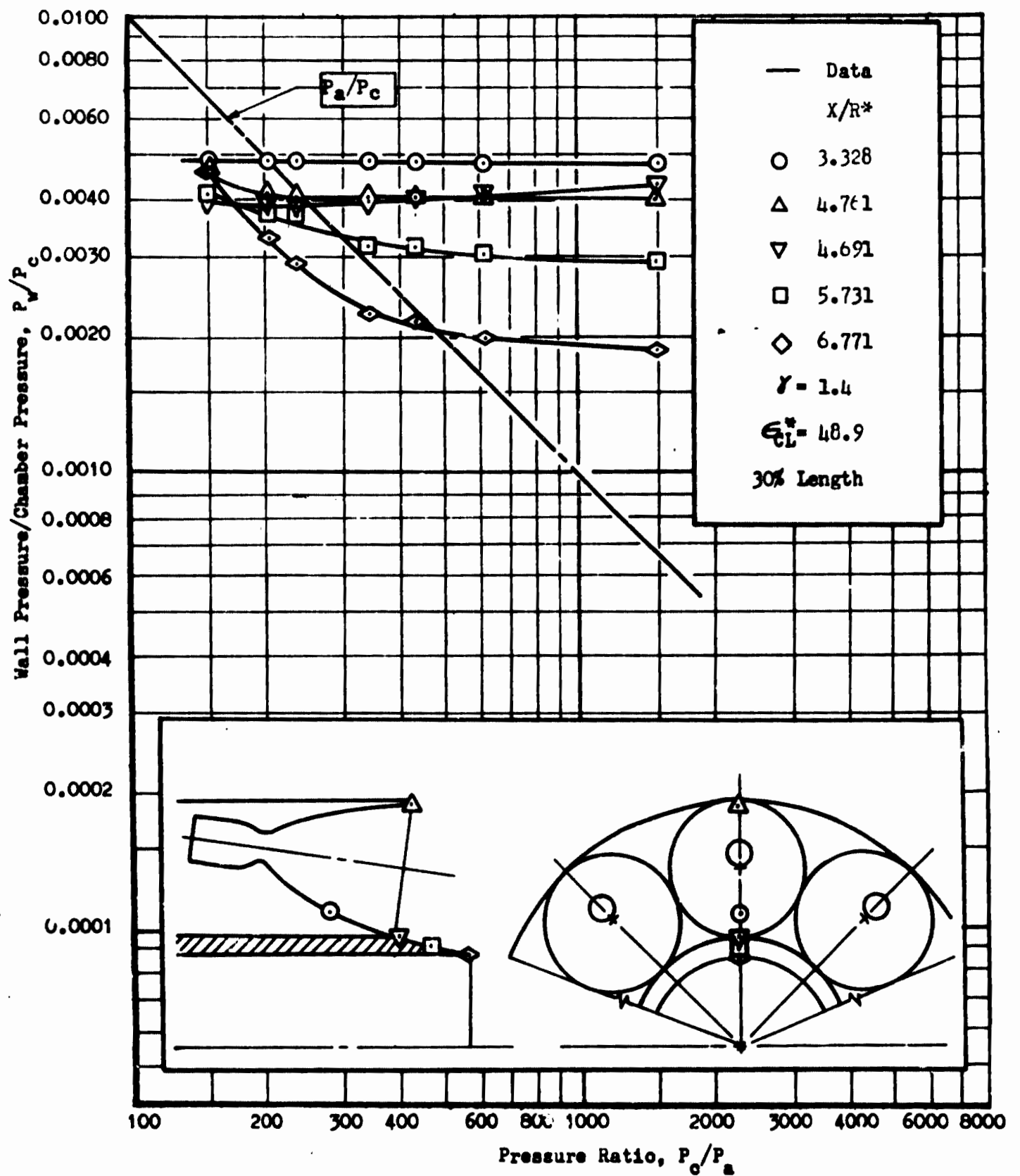
Fig. 92 Module Centerline Wall Pressure vs Pressure Ratio, 8 Modules Touching Multichamber, 30 Percent Length
