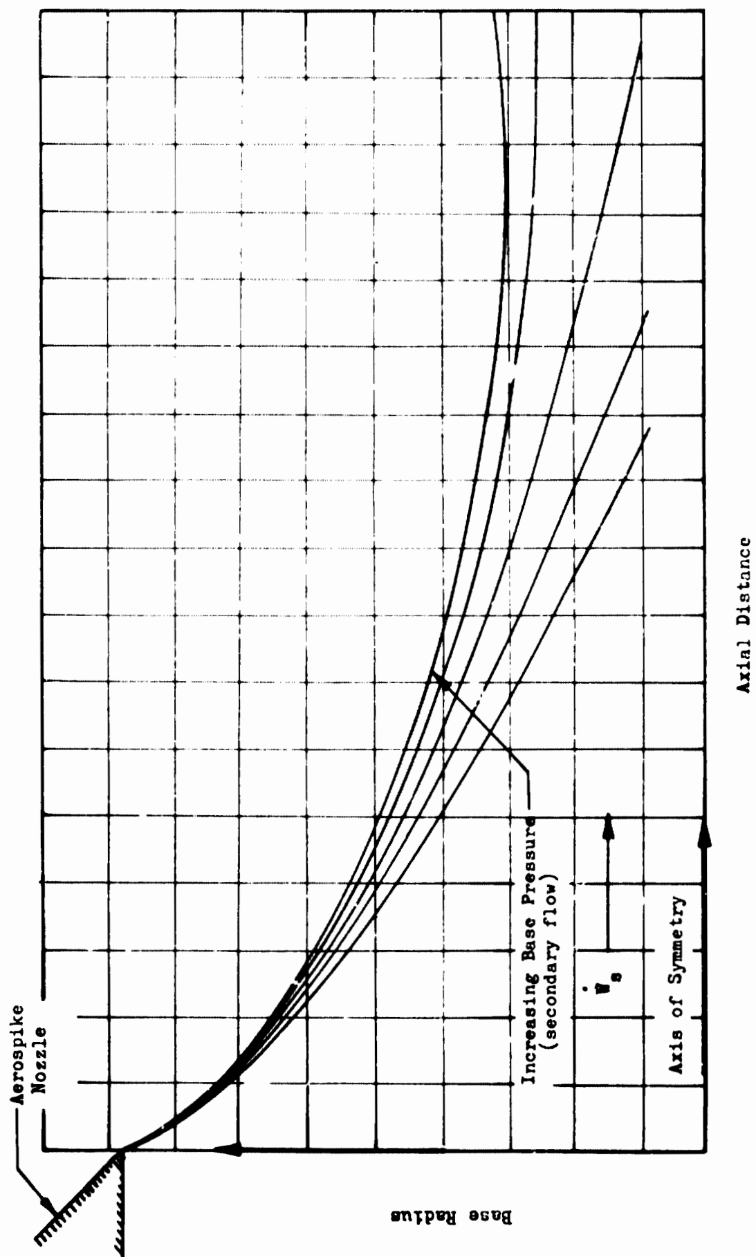
Fig. 5. Typical Solution of Aerodynamic Spike Free Jet Boundary with Various Secondary Flows
