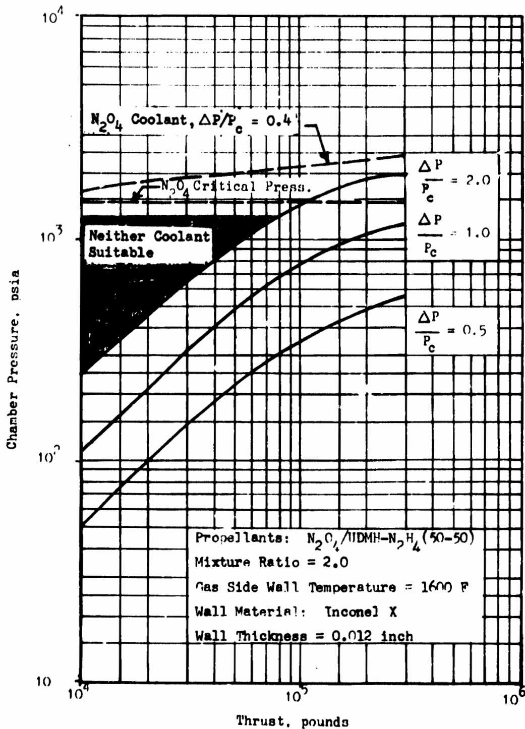
Fig. 147 Regenerative Cooling Feasibility Limits for Bell Thrust Chambers Using UDMH - N_2H_4 (50-50) as Coolant
