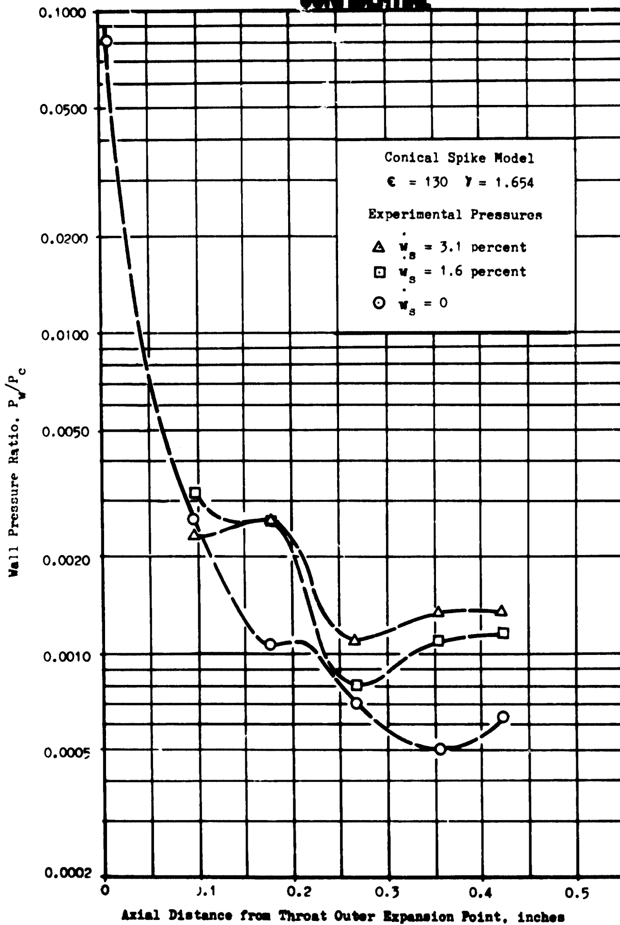
Fig. X Experimental Wall Pressure Profile with and without Secondary Flow, Conical Spike Model
