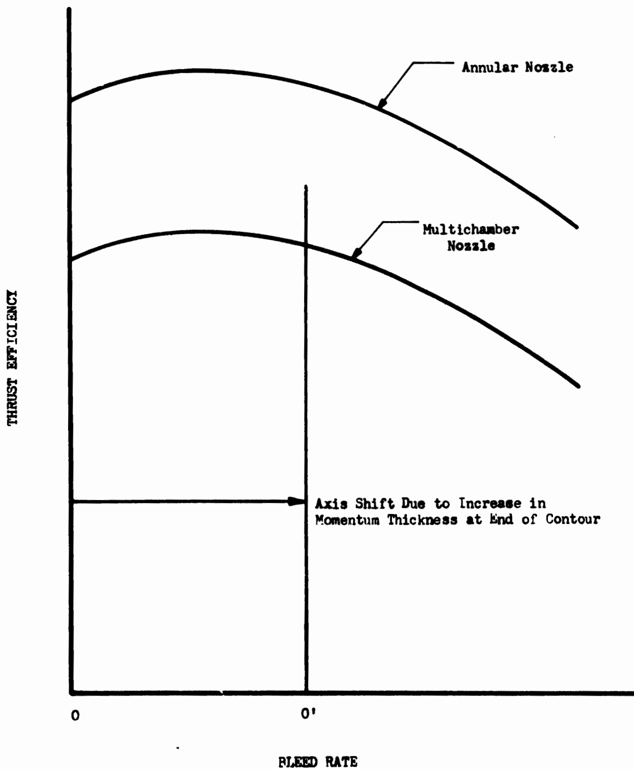
Fig. 91 Thrust Efficiency vs Bleed Rate for Annular and Multichamber Nozzle
