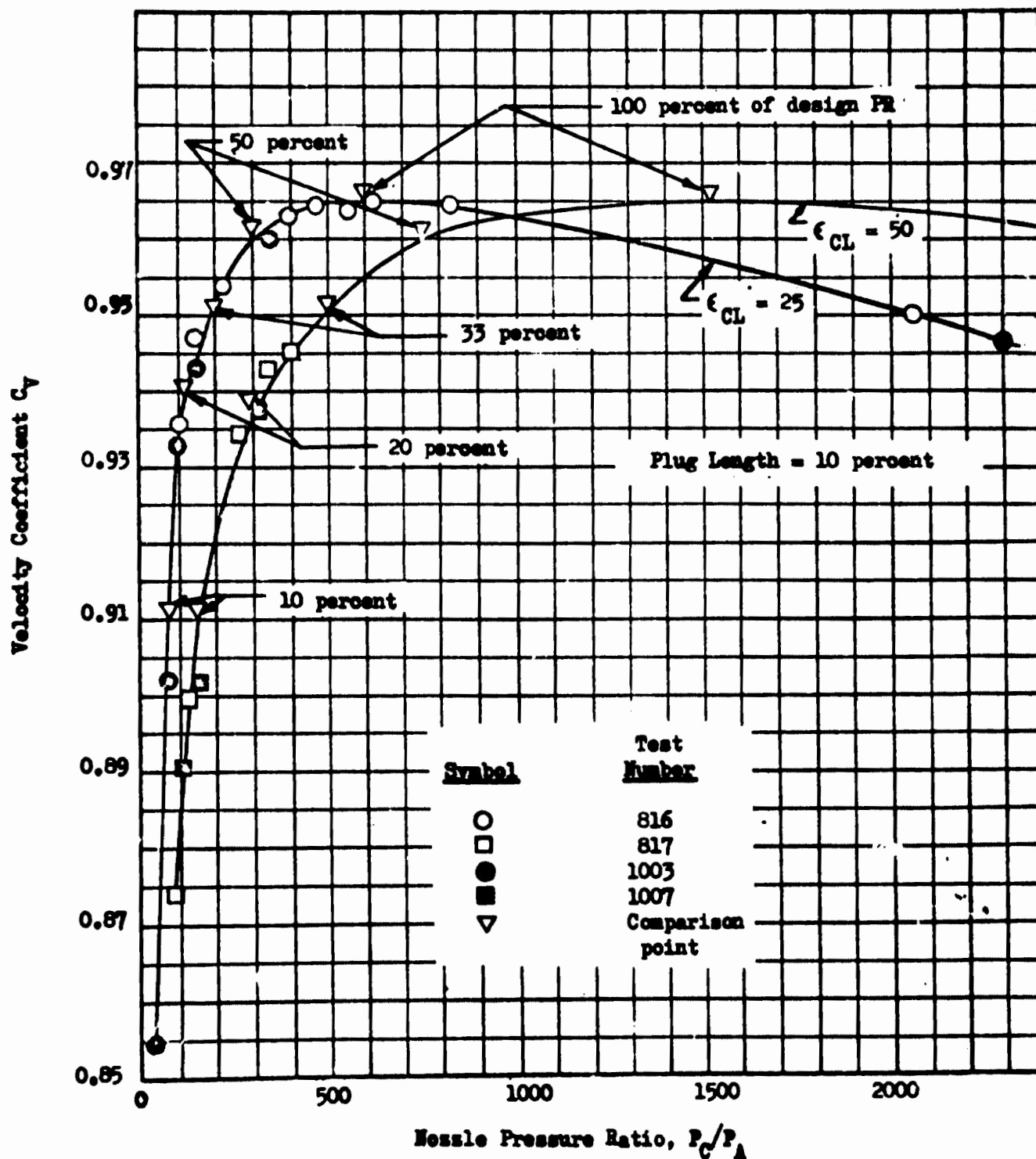
Figure 132. Effects of Cluster and Modular Area Ratio on Design Performance
