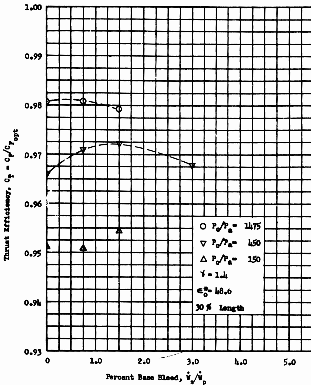
Fig. 76 Thrust Efficiency vs Percent Base Bleed, Shrouded Spike Nozzle
