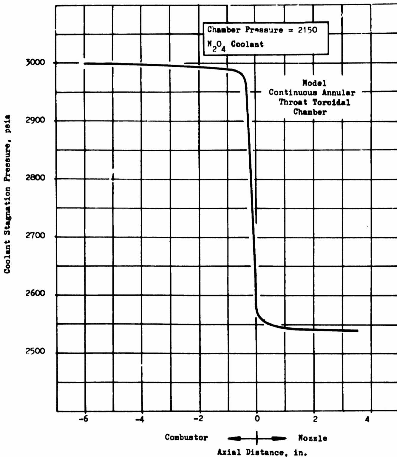
Fig.153. Typical Stagnation Pressure of Coolant vs. Axial Length
