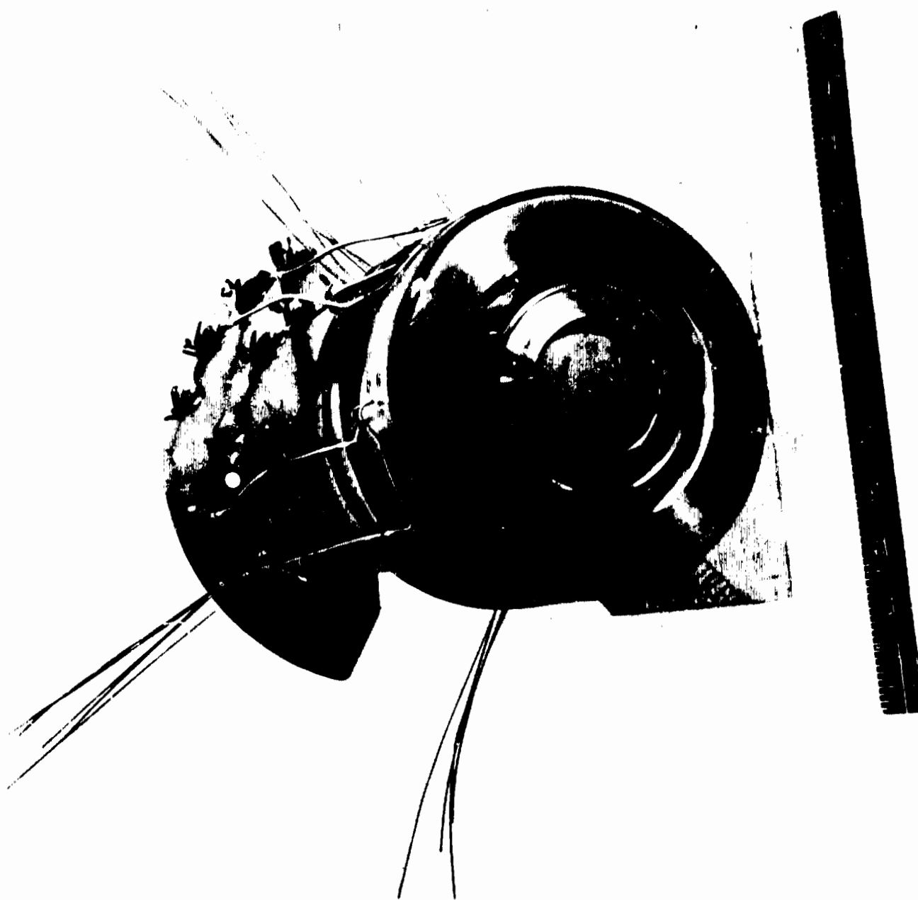
Fig. 29. Radial-Inward Secondary Injection Configuration Mounted on the Contoured Nozzle
