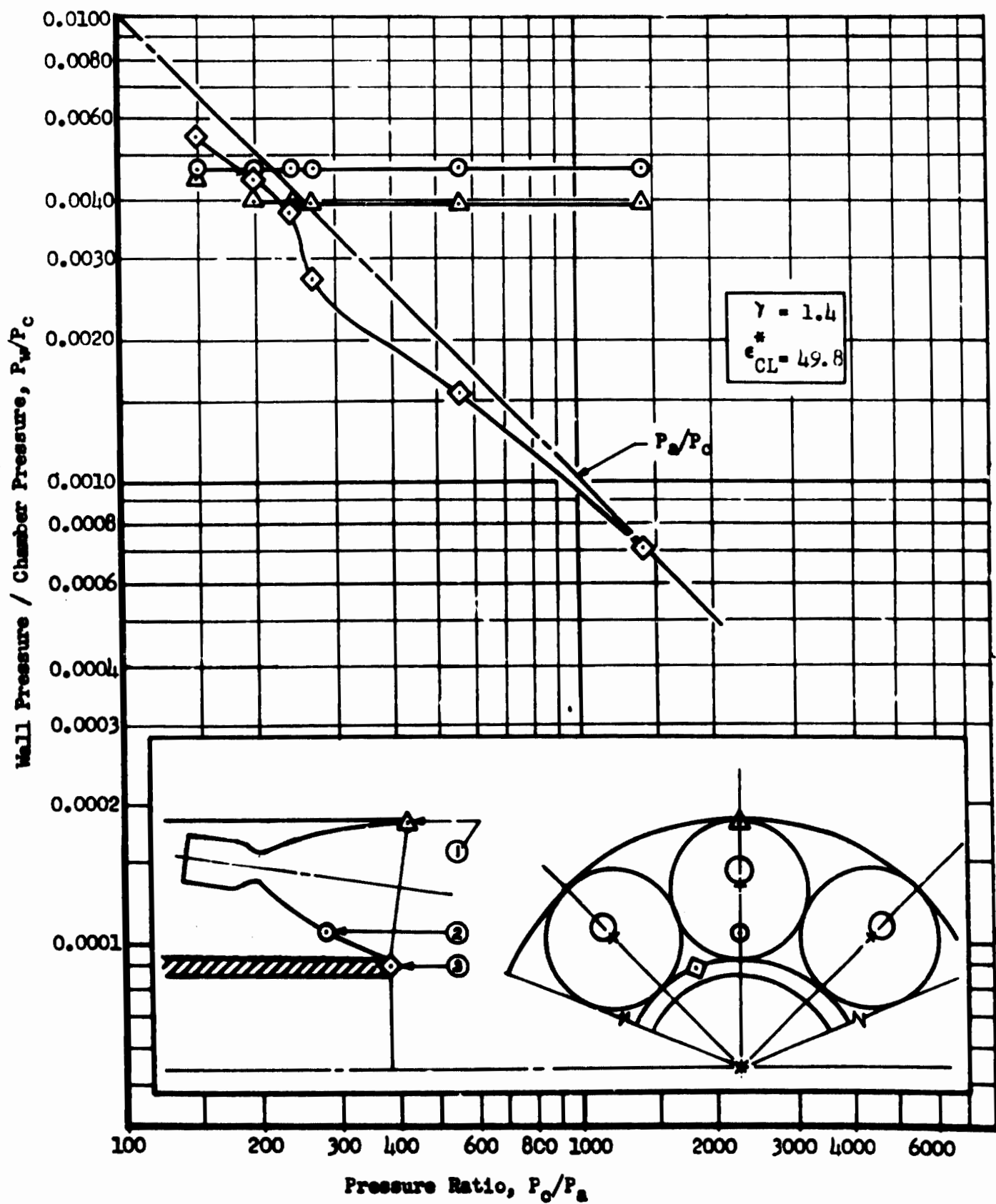
Figure 85 . Wall Pressure vs Pressure Ratio, 8 Module Touching Multichamber No Spike
