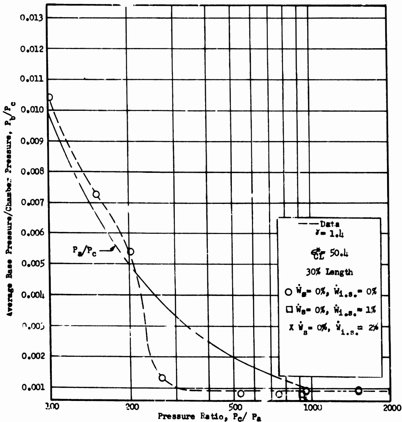
Fig. 98 Base Pressure vs Pressure Ratio, 8 Module Spaced Multichamber, 30 percent Length
