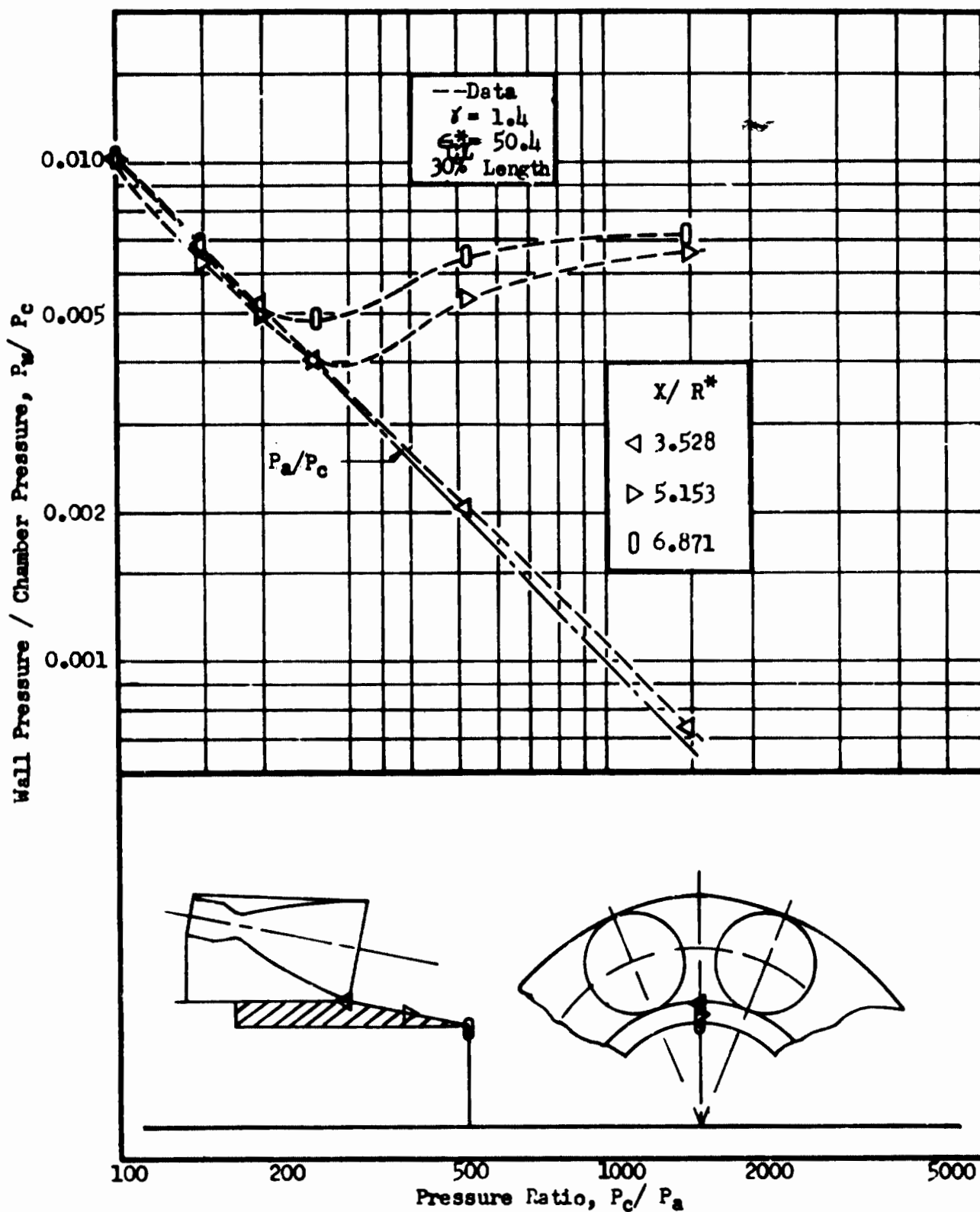
Fig.100 Wall Pressure Between Modules vs Pressure Ratio, 8 Modules Spaced Multichamber, 30 Percent Length
