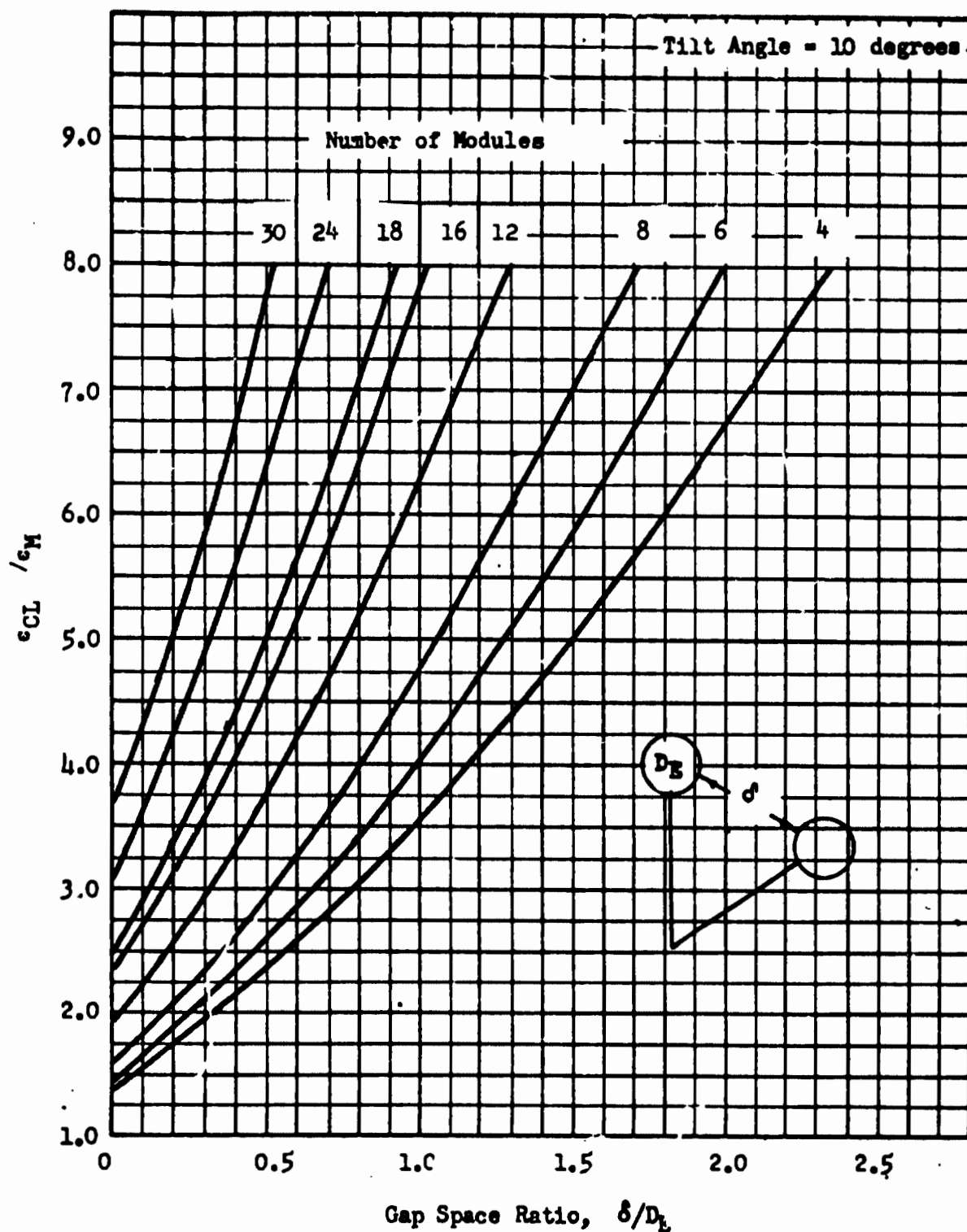
Figure 117. Geometric Amplification Factor as a Function of Circular Gap Spacing Ratio and Number of Modules
