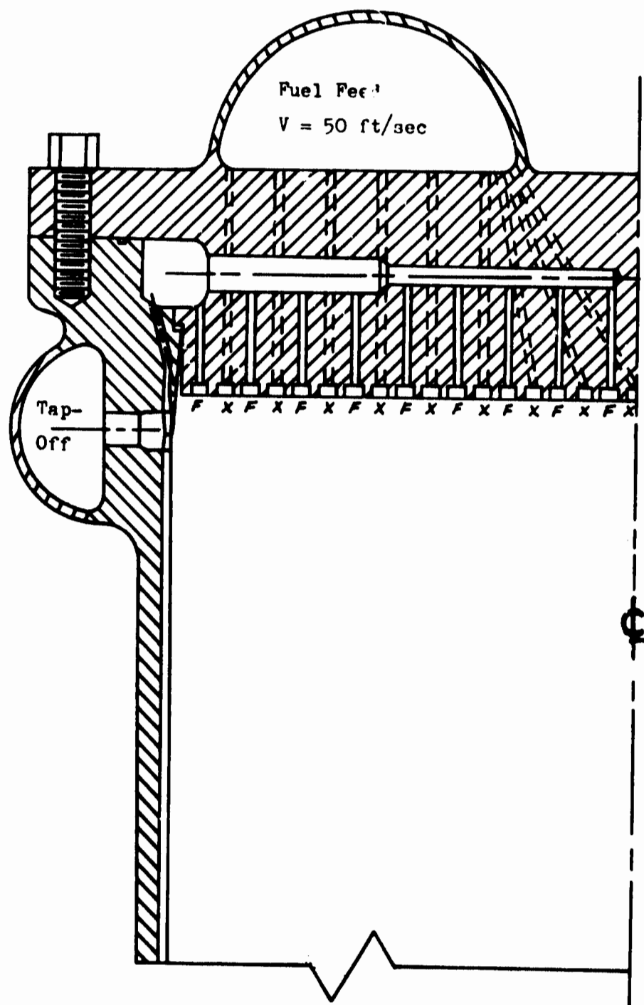
Fig. 173. Up Pass Flow Path Injector
