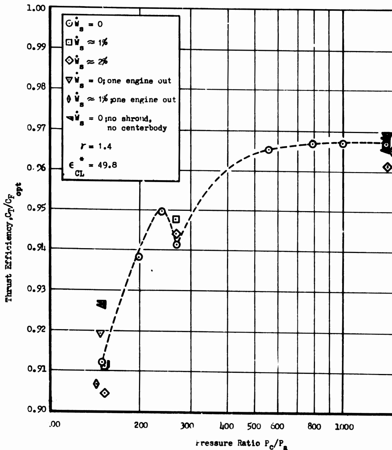
Fig. 82 Thrust Efficiency vs Pressure Ratio, 6 Module Touching Multichamber, No Spike
