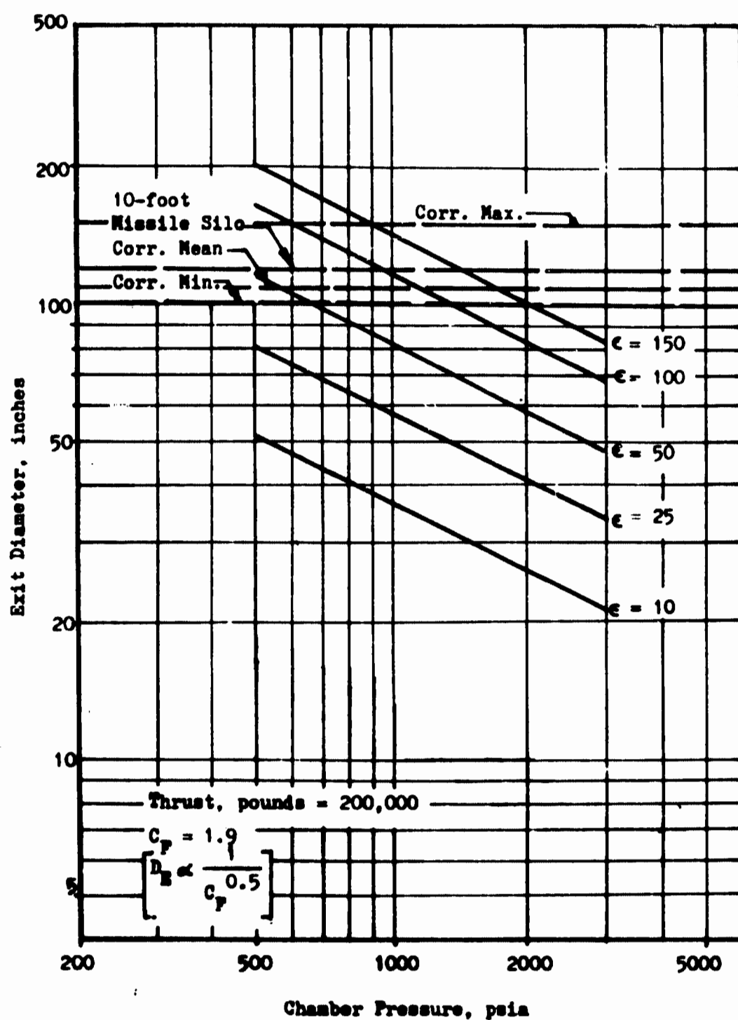
Fig. 22. Toroidal Engine Envelope ( F = 200,000 pounds)
