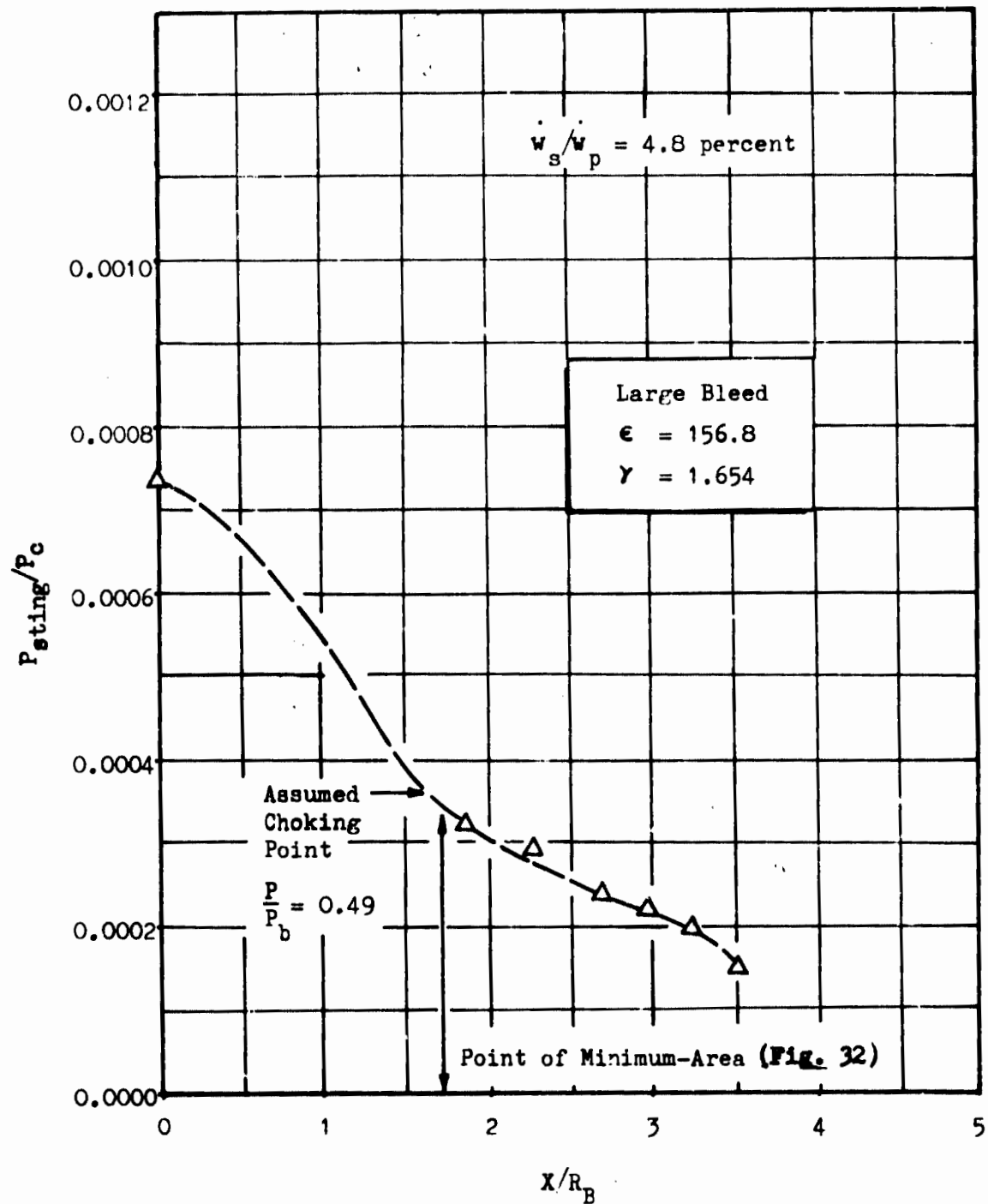
Fig.44. Centerline Wake Pressure Profile Contoured Spike Configuration . Large Bleed
