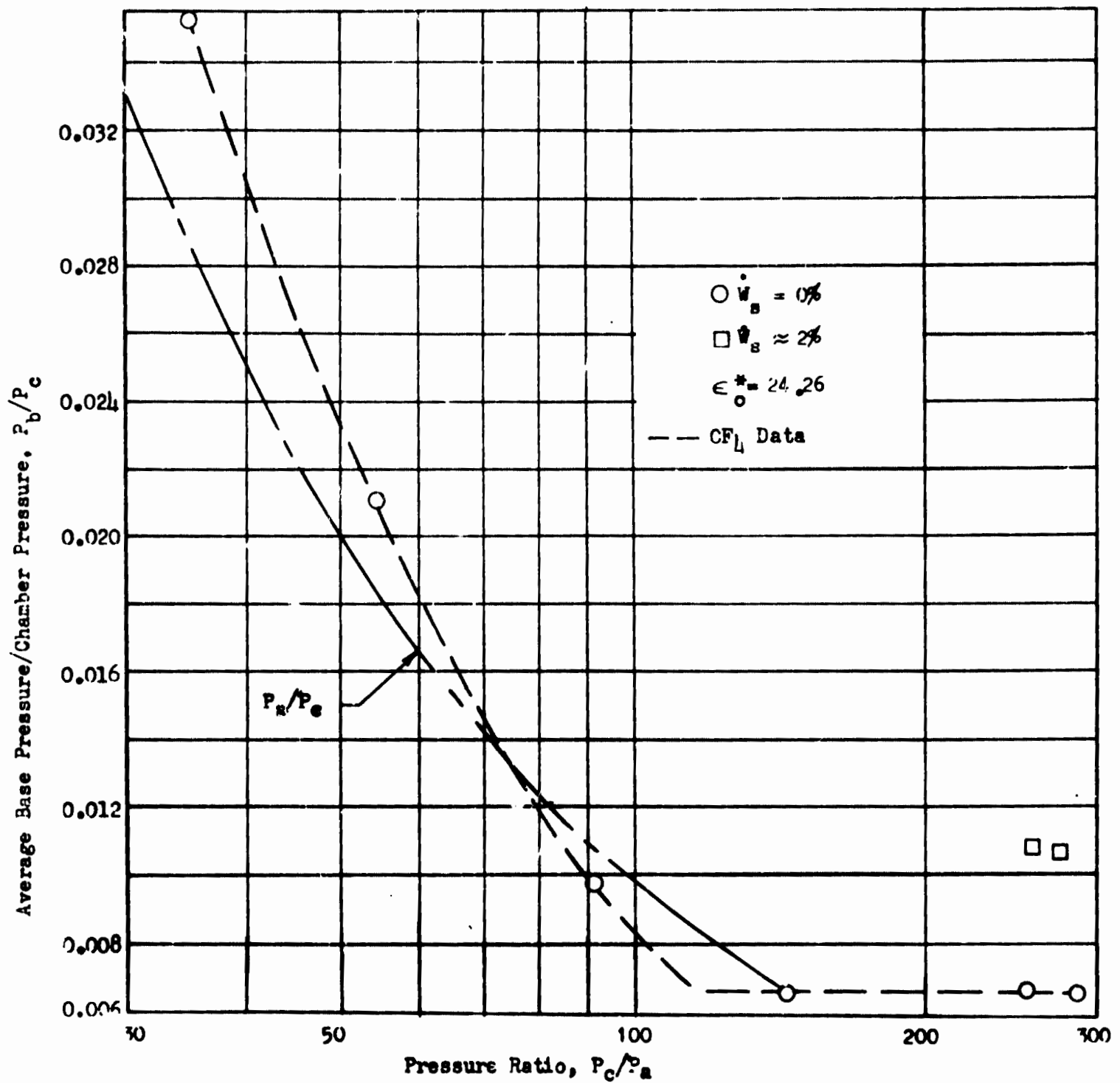
Fig. 66. Base Pressure vs Pressure Ratio, cooled Hot-Firing Model, CF_4 Tests
