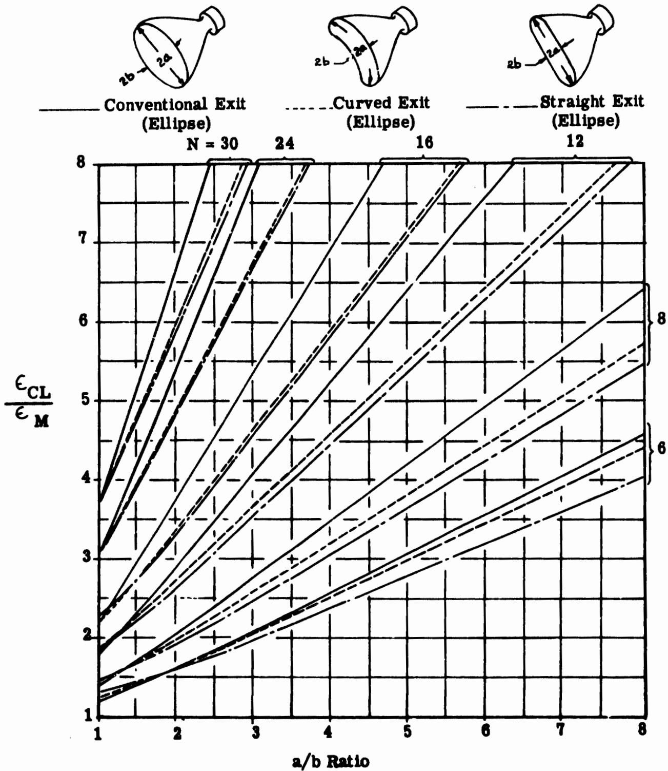
Figure 118 Amplification Factor as a Function of Ellipse Ratio and Number of Modules
