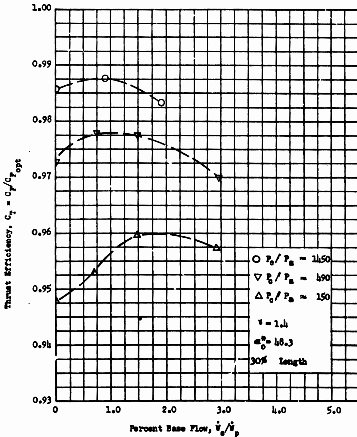
Fig. 71 Thrust Efficiency vs Percent Base Flow, Point Expansion Spike Nozzle
