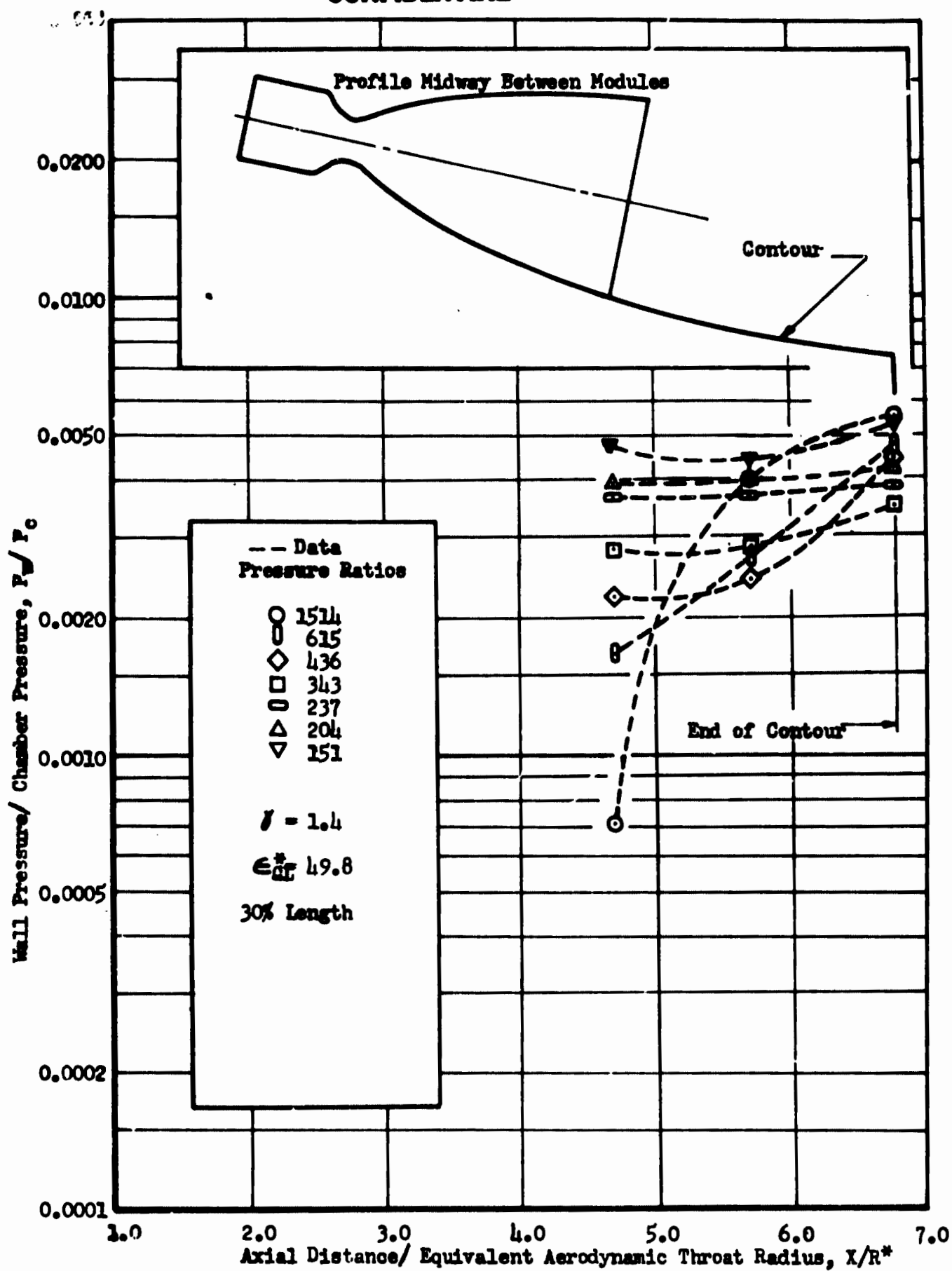
Fig. 9b Wall Pressure Between Modules vs Axial Length, 8 Modules Touching Multichamber, 30 Percent Length
