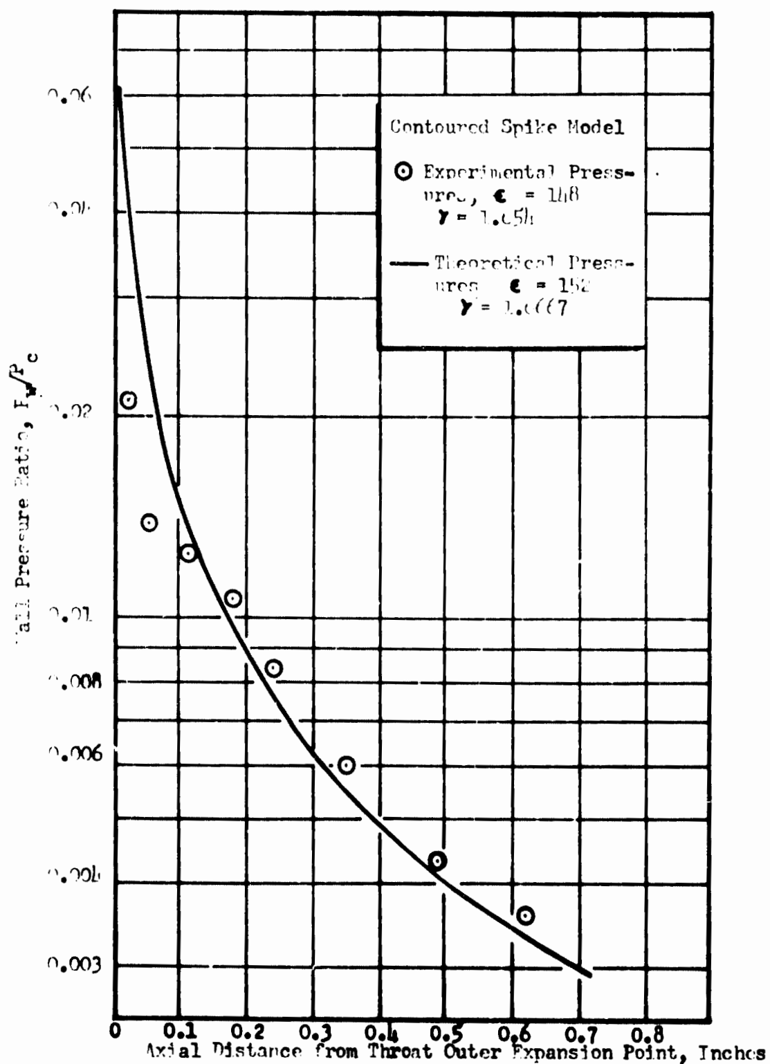
Fig.23. Theoretical and Experimental Wall Pressure Profiles, Contoured Spike Model
