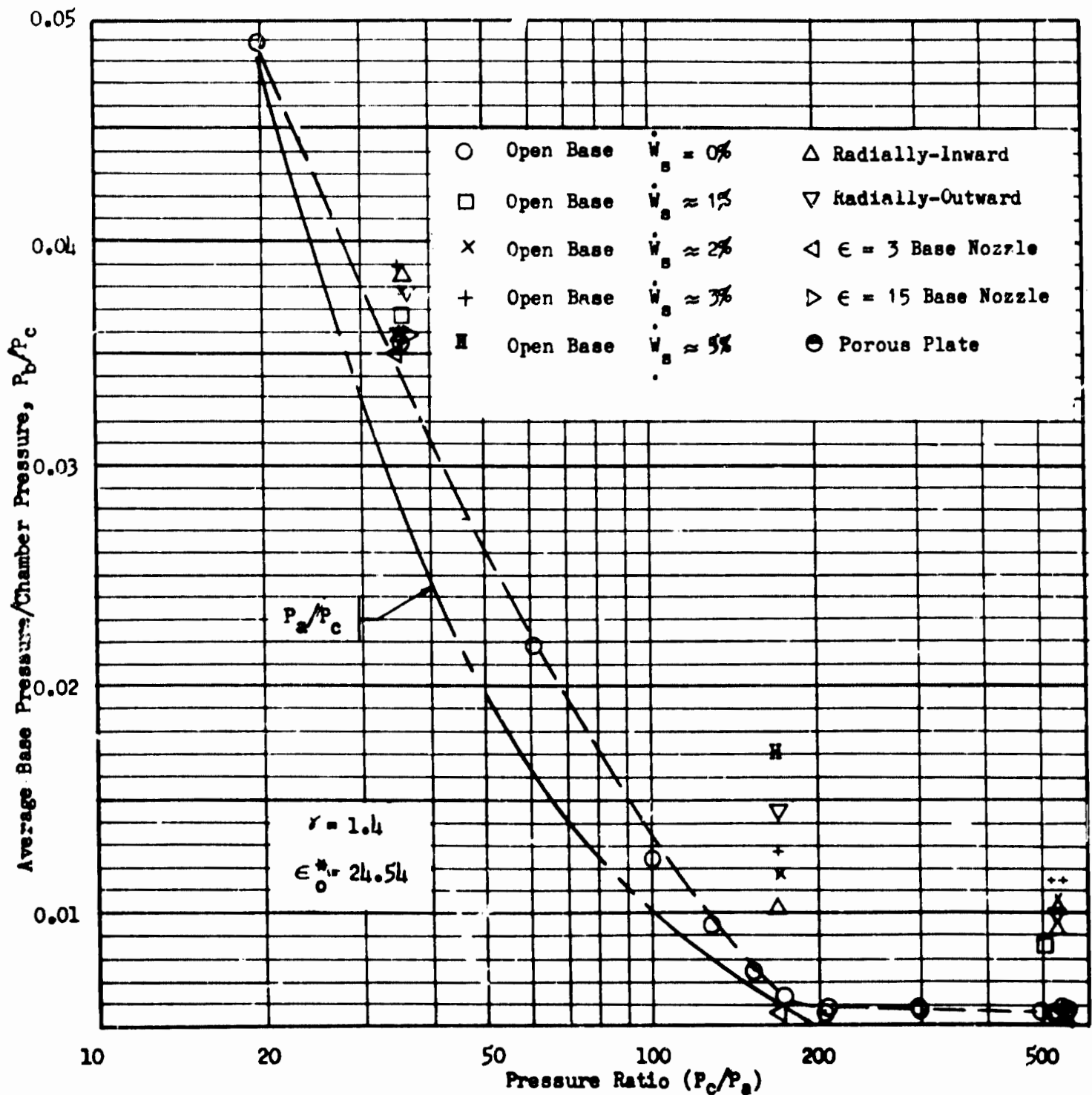
Fig. 61. Base Pressure Curves for Scaled Hot-Firing Model
