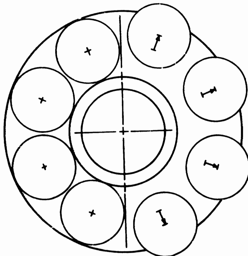
Fig. 175 Multichamber Thrust Vector Control By Module Displacement
