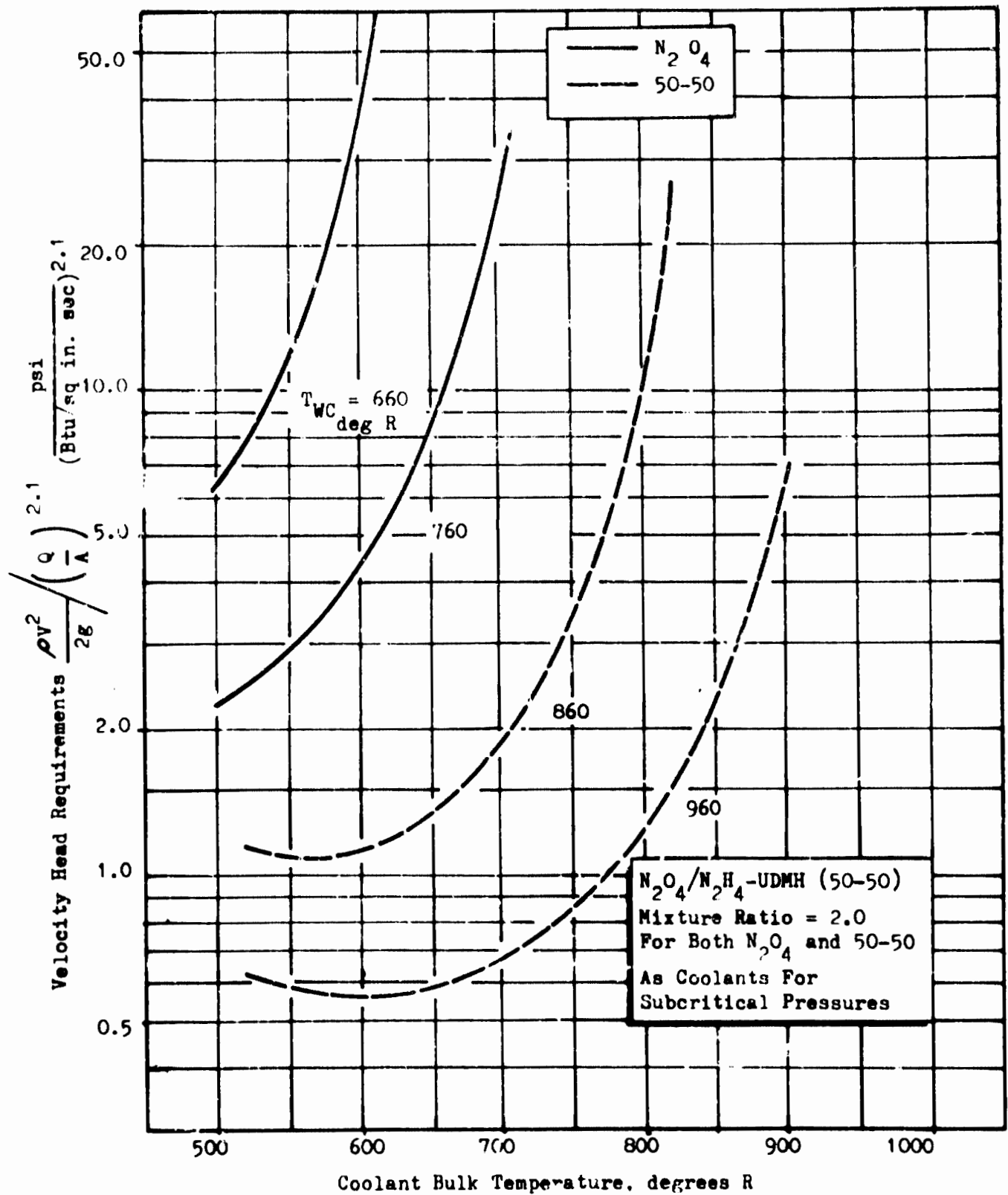
Fig. 140 Coolant Velocity Head Requirements vs Coolant Bulk and Wall Temperature
