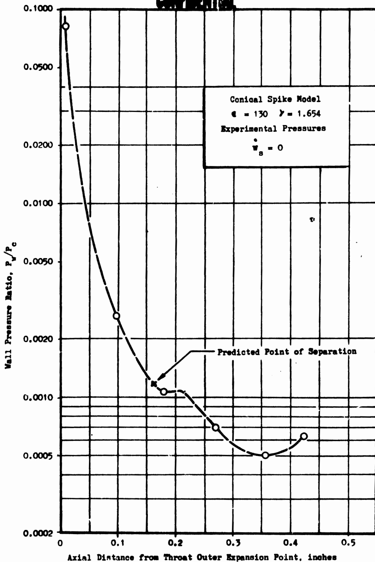
Fig. 37. Experimental Wall Pressure Profile Without Secondary Flow. Conical Spike Model
