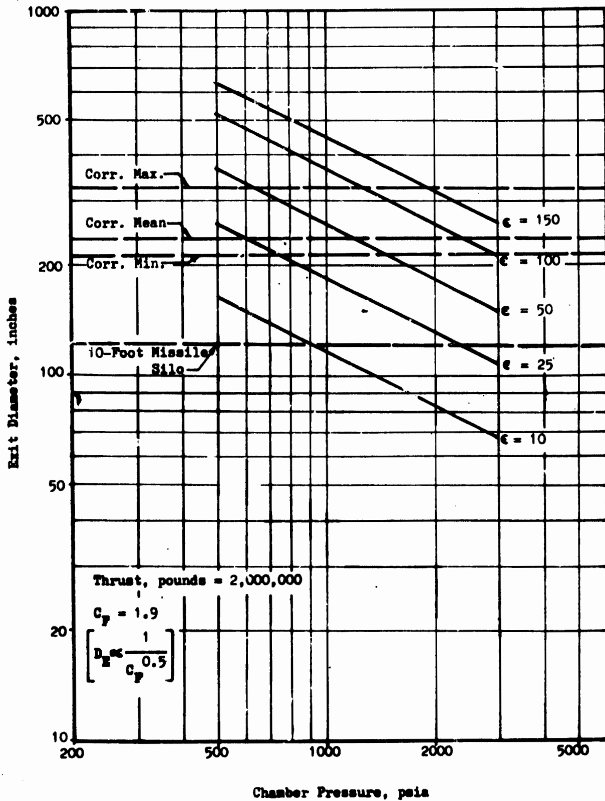
Fig 123 Toroidal Engine Envelope ( F = 2,000,000 pounds)
