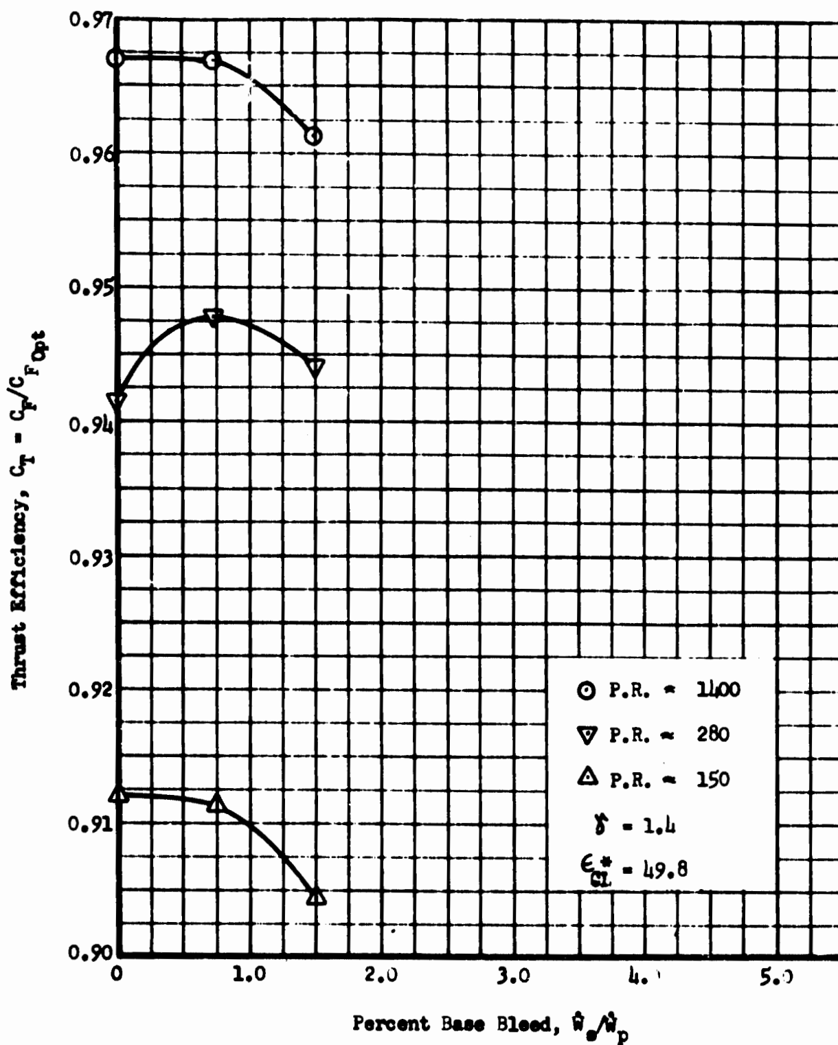
Fig. 83 Thrust Efficiency vs Percent Base Bleed, 8 Module Touching Multichamber, No Spike
