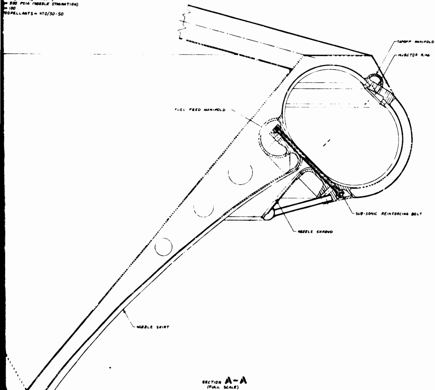
Fig. 157. Aerospike Engine System, Toroidal, Low Thrust, Low Chamber Pressure
