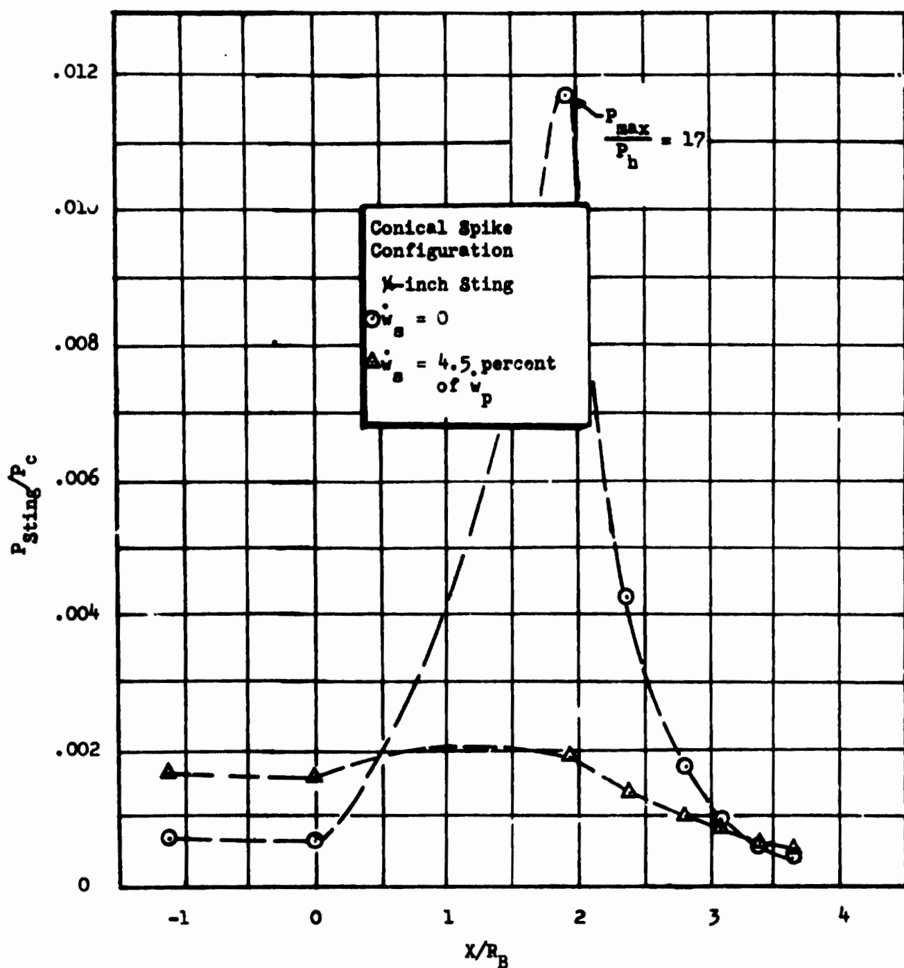
Fig. 42 Centerline Wake Pressure Profile, Conical Spike
