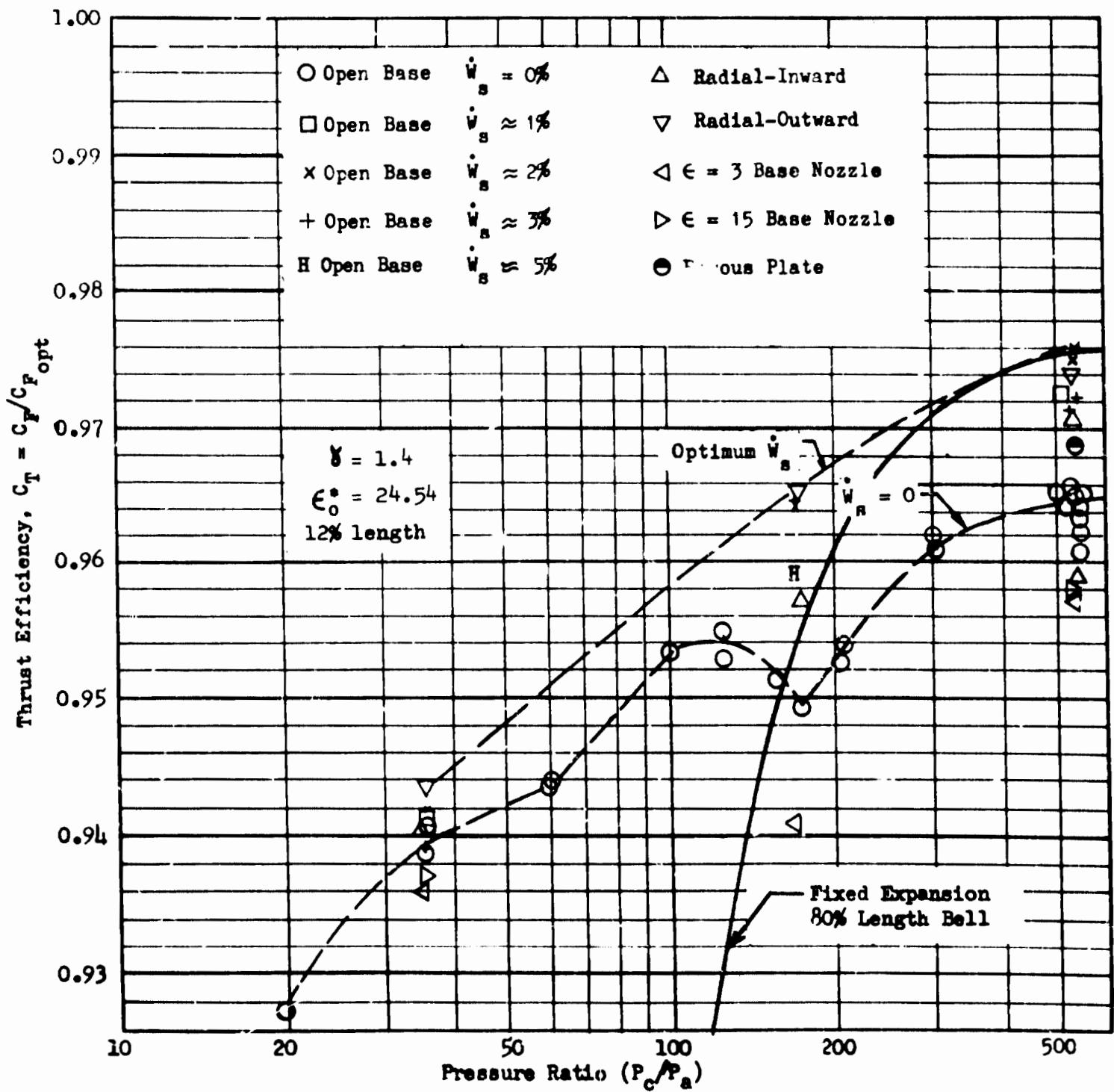
Fig. 58 Performance vs Pressure Ratio, Scaled Hot-Firing Model
