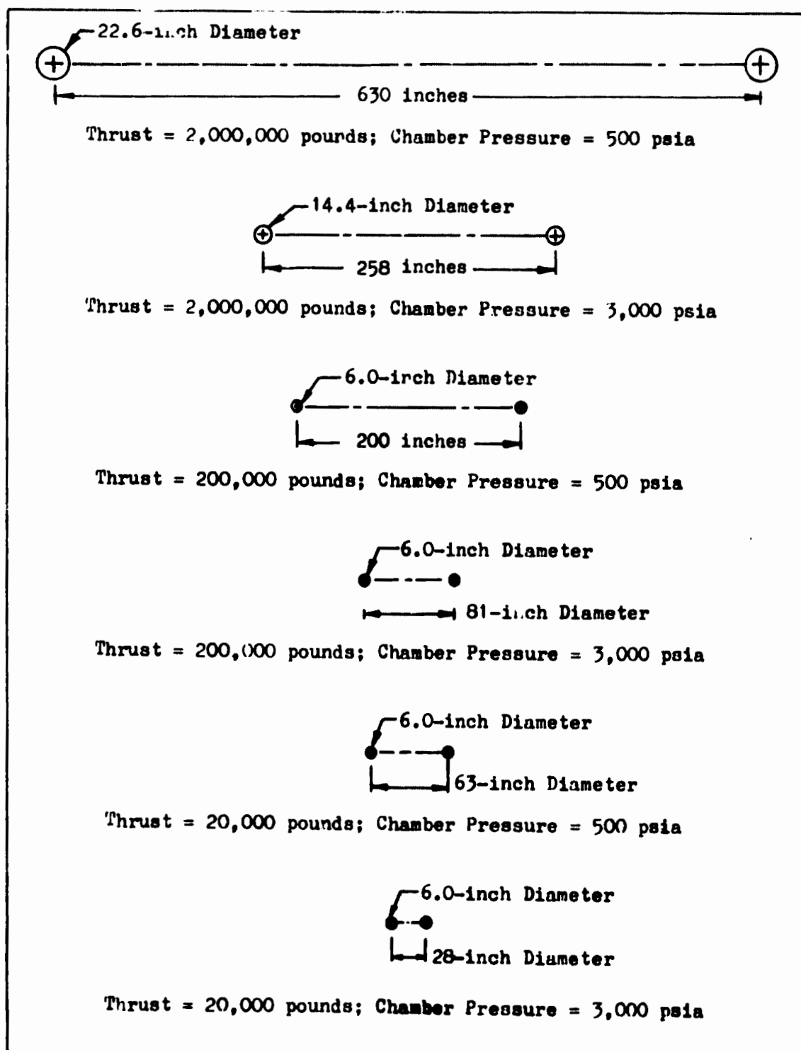
Fig. 119 Limit Combustor Dimensions, \epsilon = 150
