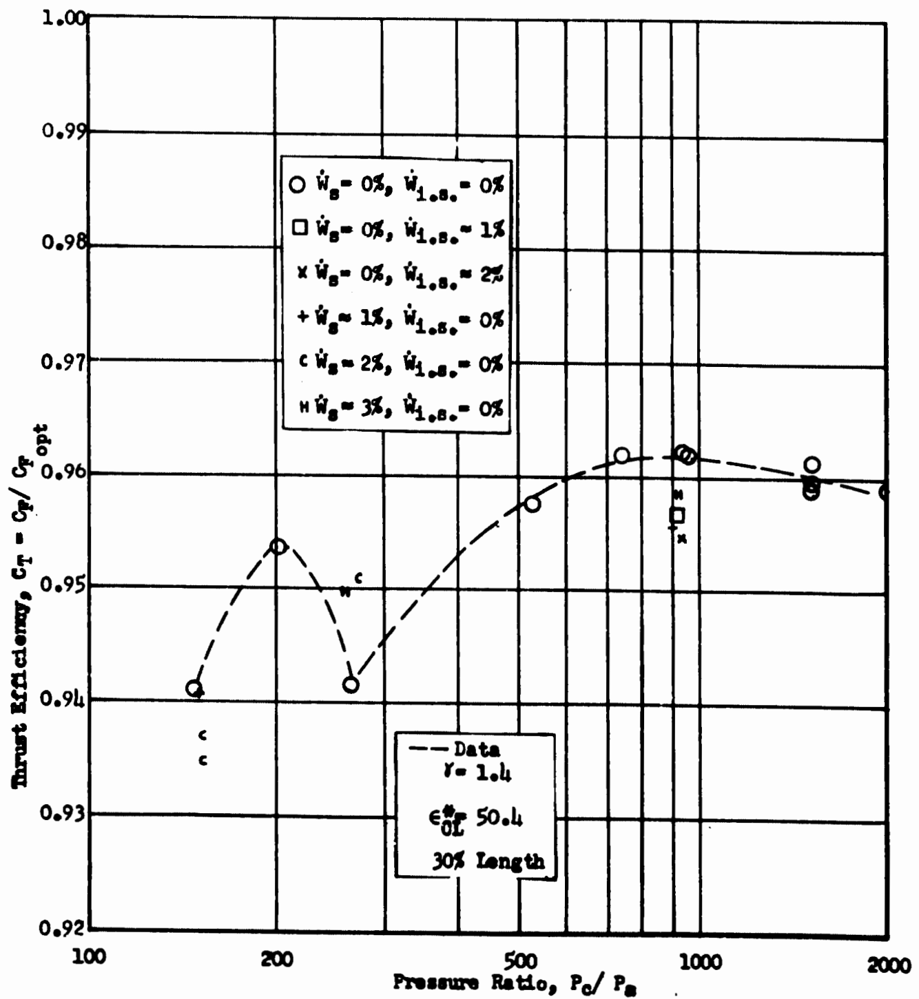
Fig. 96 Thrust Efficiency vs Pressure Ratio, 8 Modules Spaced Multichamber, 30 percent Length
