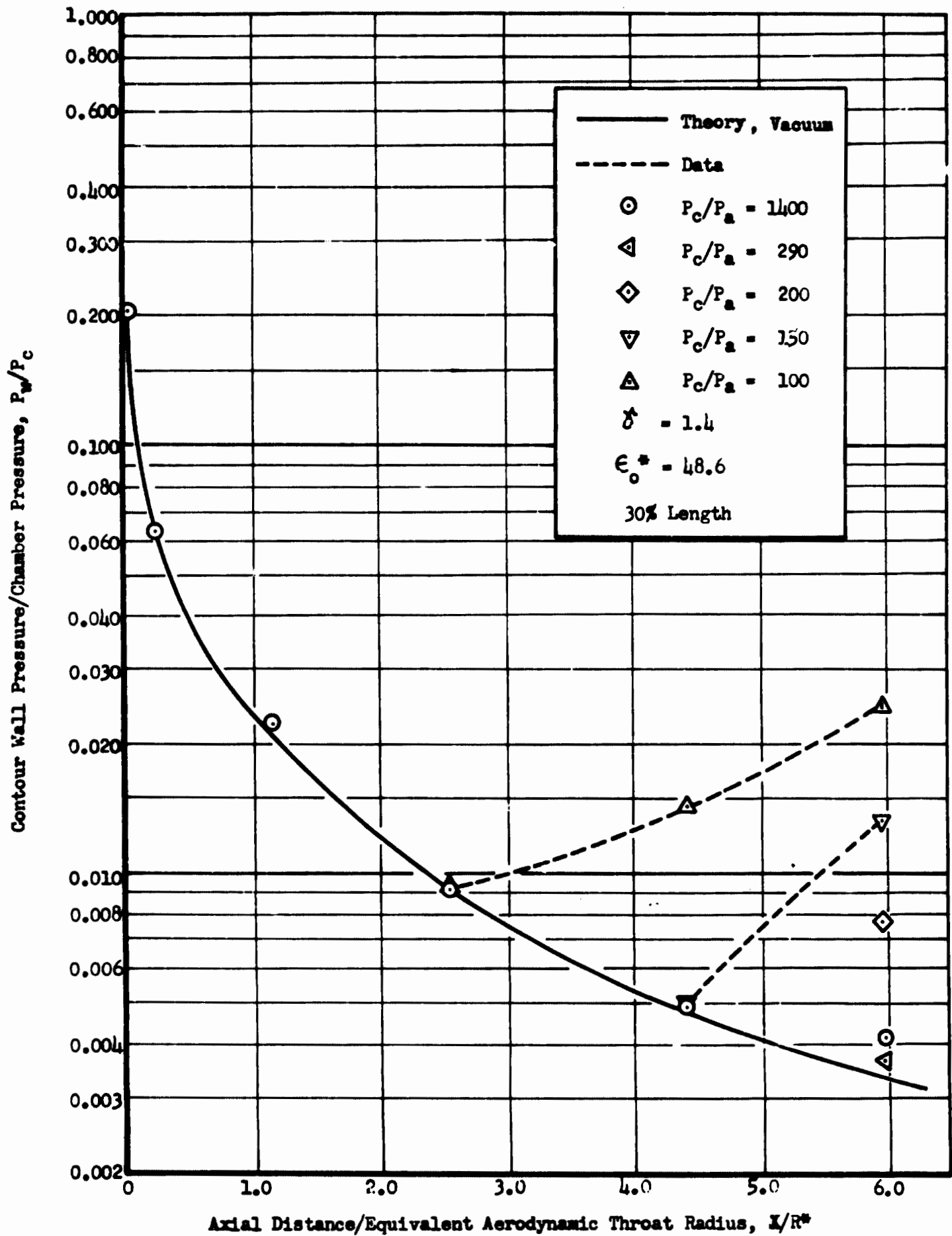
Fig. 78 Contour Pressure Profile, Shrouded Spike Nozzle.
