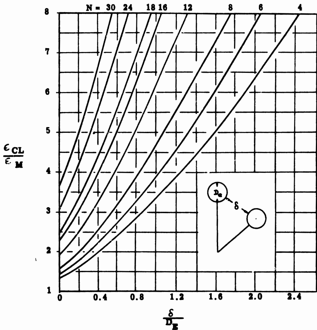
Figure 116. Geometric Amplification Factor as a Function of Circular Gap Spacing Ratio and Number of Modules
