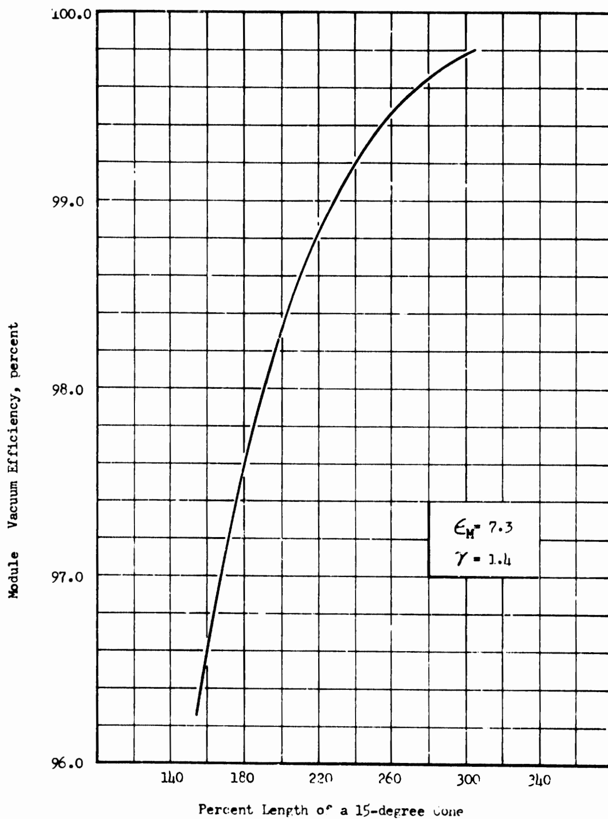
Fig. 164 Maximum Performance vs Percent Length for a Two-Dimensional Nozzle
