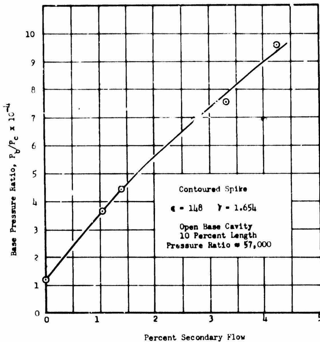
Fig. 19. Base Pressure Ratio versus Secondary Flow, Contoured Spike Model
