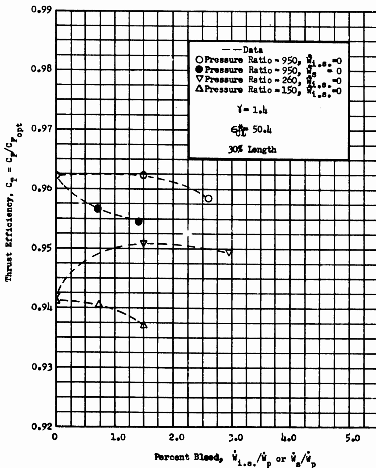
Fig. 97 Thrust Efficiency vs Percent Bleed, 8 Module Spaced Multichamber, 30 percent Length
