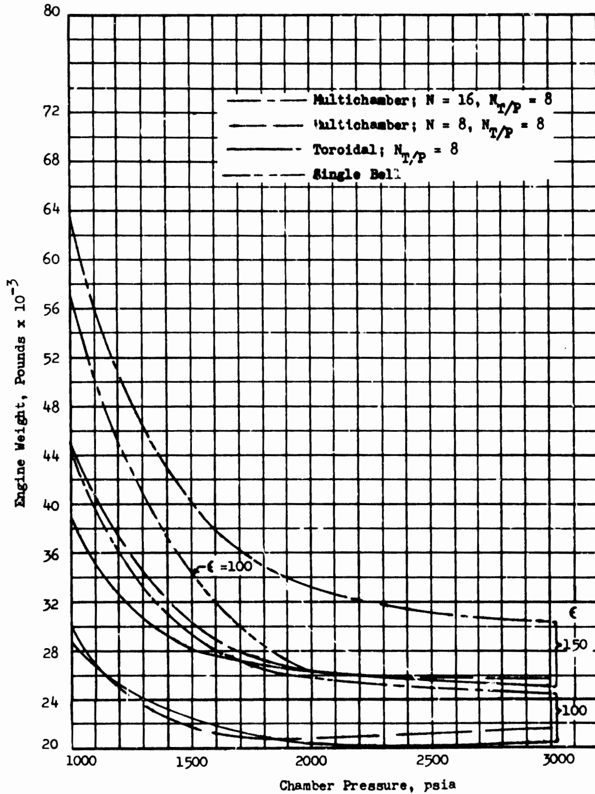
Fig. 139. Engine Weight vs Chamber Pressure - \epsilon = 100 and 150
