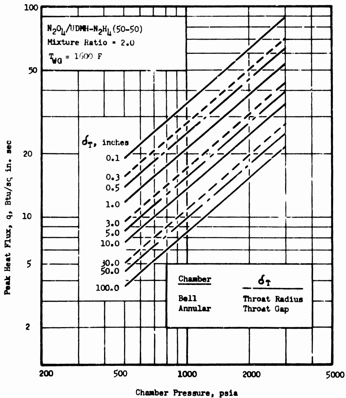
Fig. 142 Peak Heat Fluxes for Bell Nozzles and Continuous Annular Throat Toroidal Combustor
