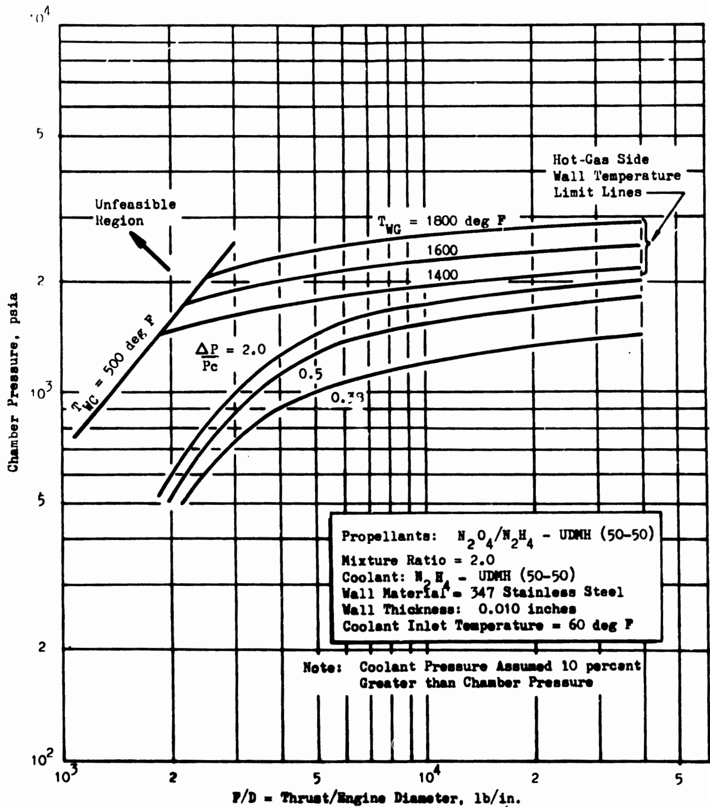
Fig.149 Cooling Feasibility Limits and Pressure Drops for Continuous Annular Throat Toroidal Combustors Using N_2H_4 -UDMH as Coolant
