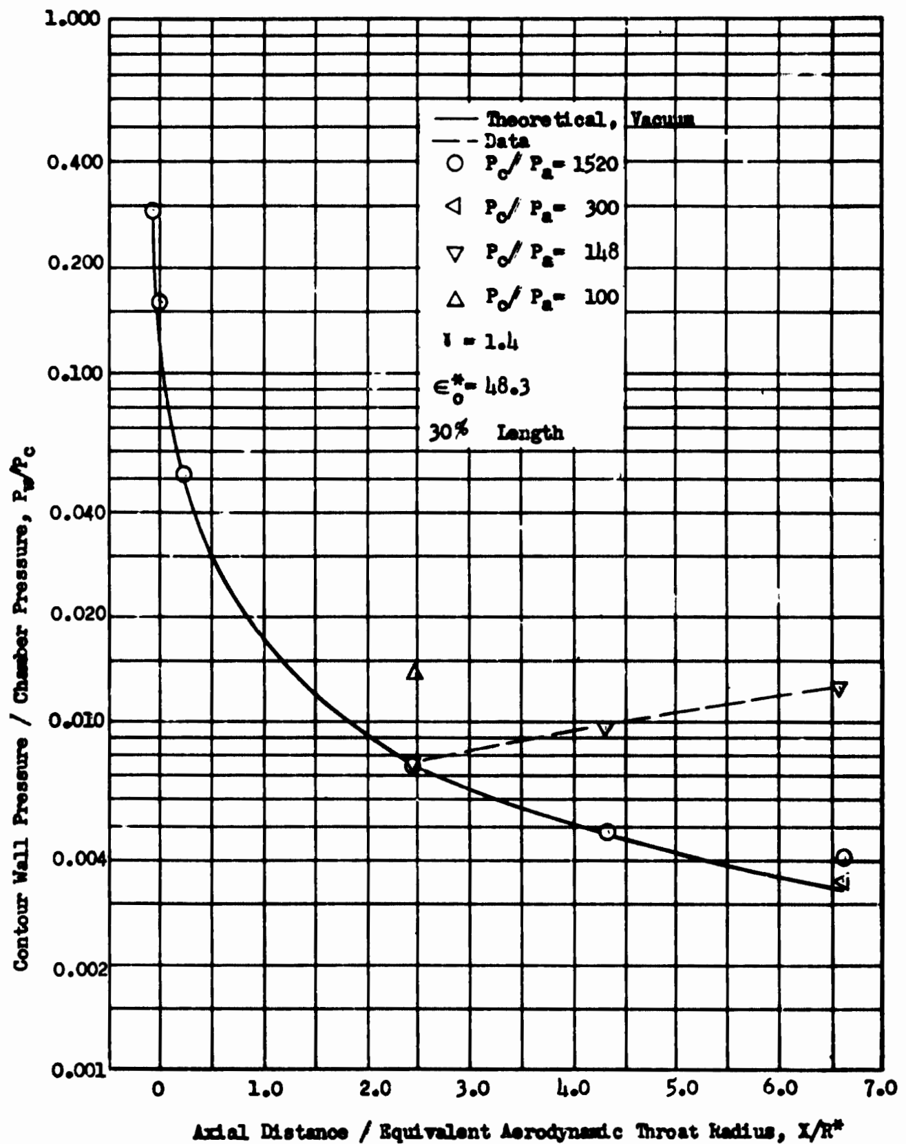
Fig. 73 Contour Pressure Profile, Point Expansion Spike Nozzle
