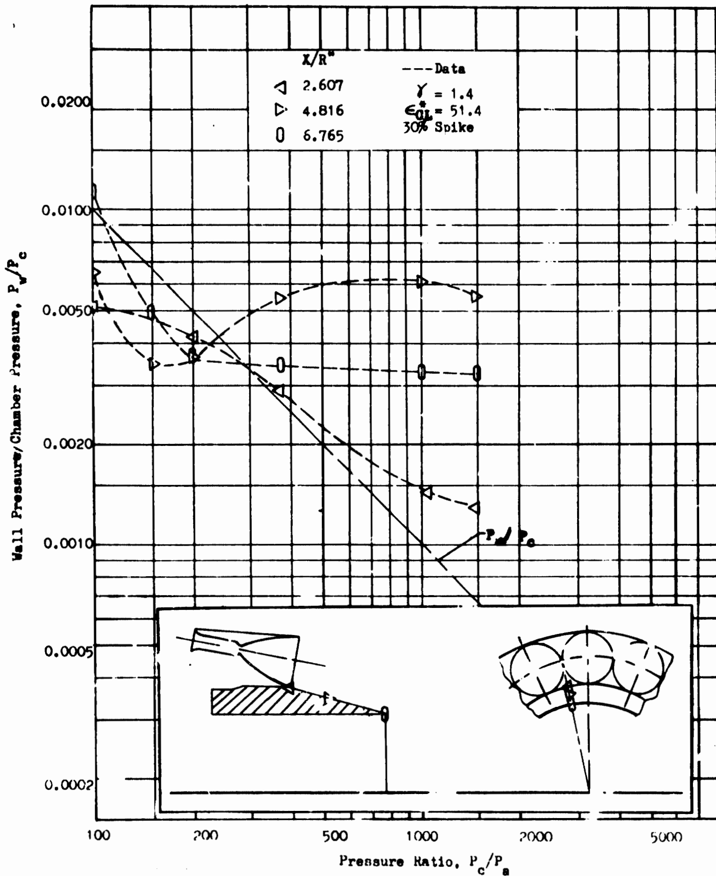
Fig. 107 Wall Pressure Between Modules vs Pressure Ratio, 16 Module Multichamber, 30 Percent Length
