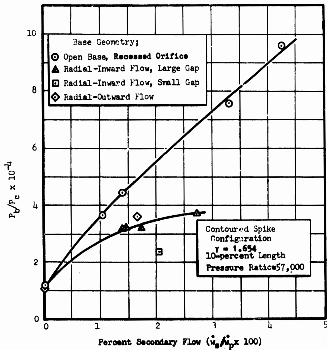
Fig. 31. Base Pressure Ratio vs Secondary Flowrate Contoured Aerodynamic Spike
