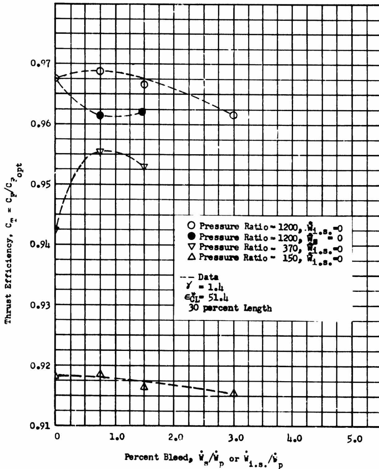
Fig. 105 Thrust Efficiency vs Percent Bleed, 16 Module Multichamber, 30 percent Length
