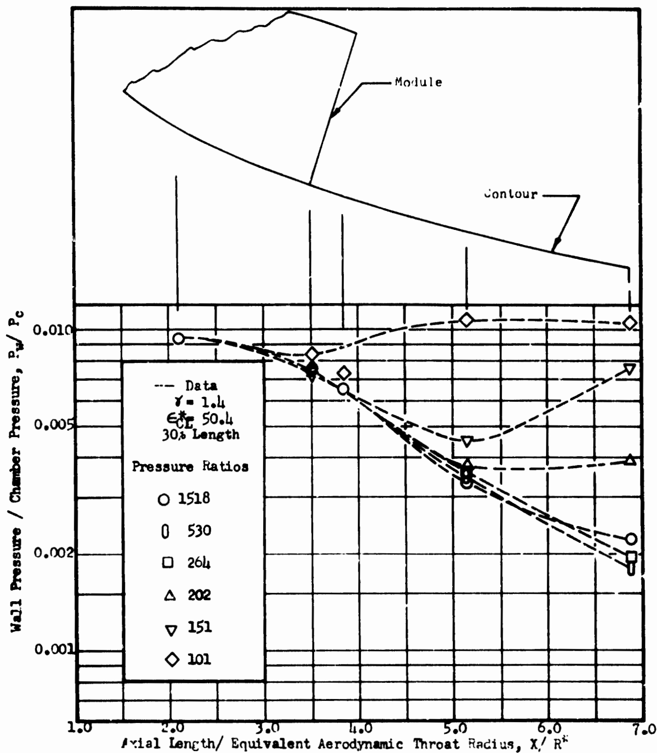
Fig.101 Module Centerline Wall Pressure vs Axial Distance, 8 Modules Spaced Multichamber, 30 percent Length
