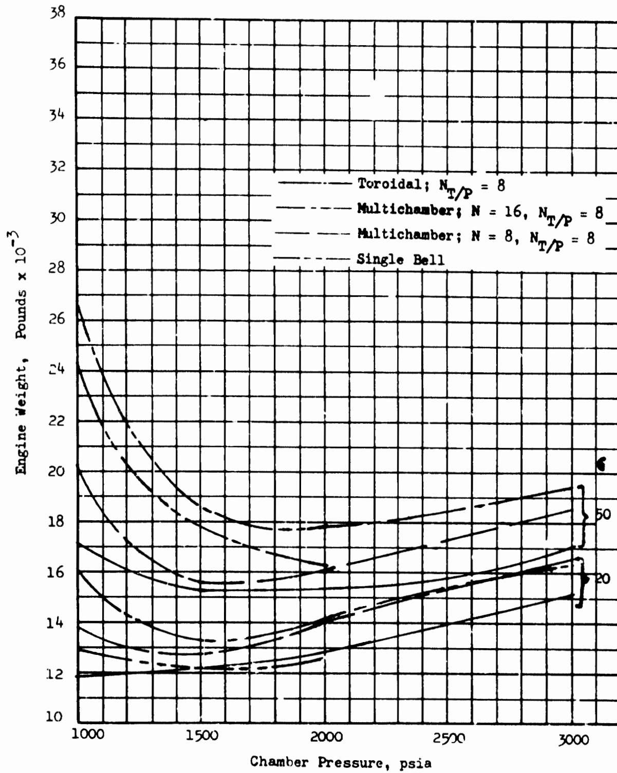
Fig. 138. Engine Weight vs Chamber Pressure - \epsilon = 20 and 50
