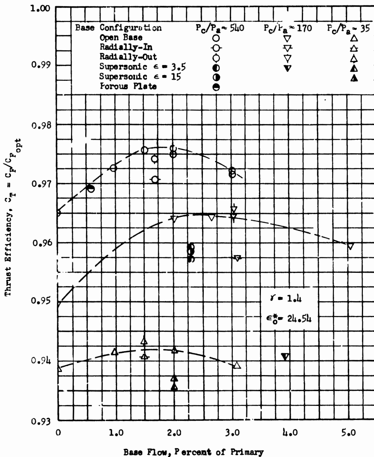
Fig. 59 Performance vs Base Flow Rate, Scaled Hot-Firing Model
