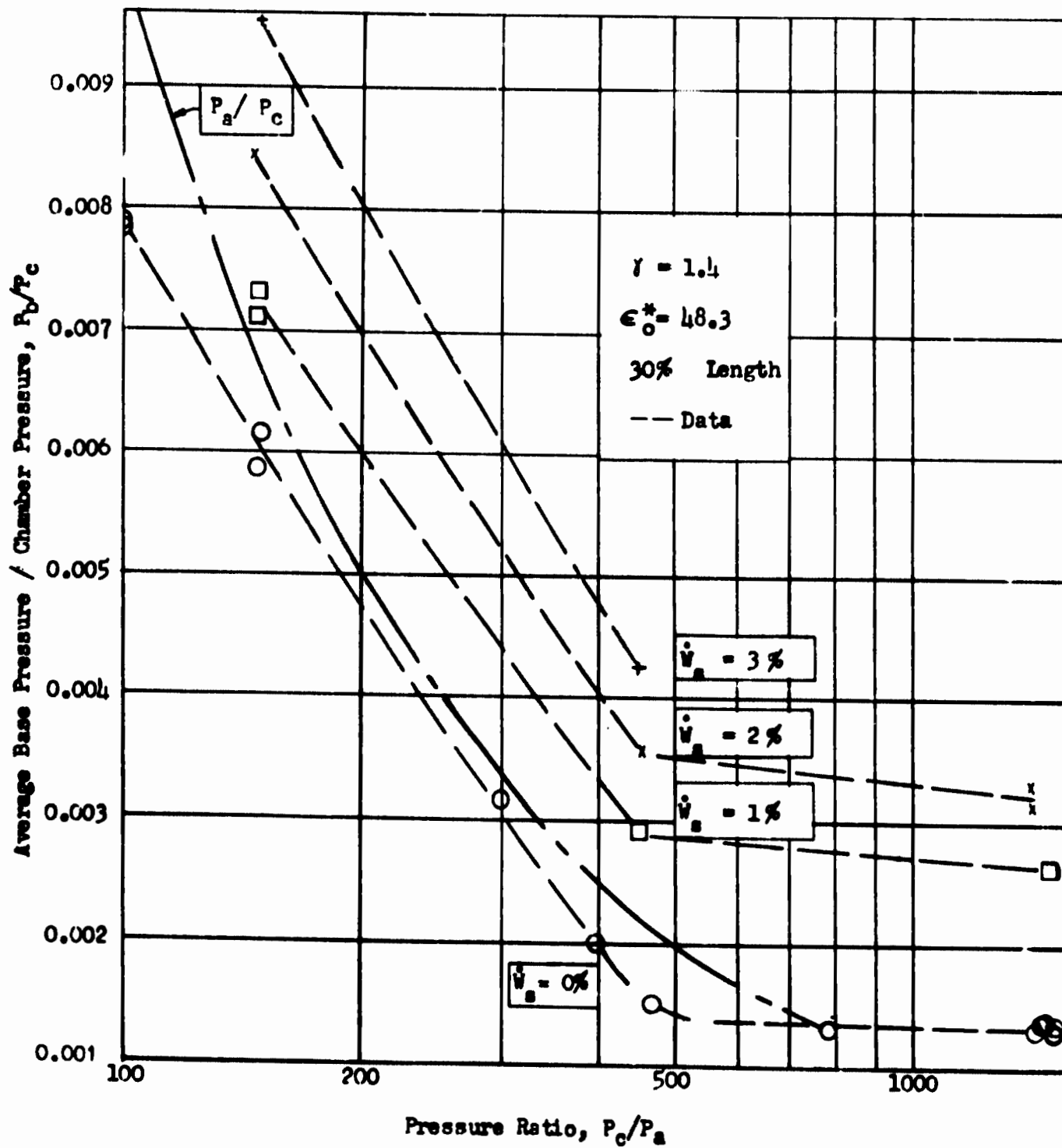
Fig. 72 Base Pressure vs Pressure Ratio for Point Expansion Spike Nozzle
