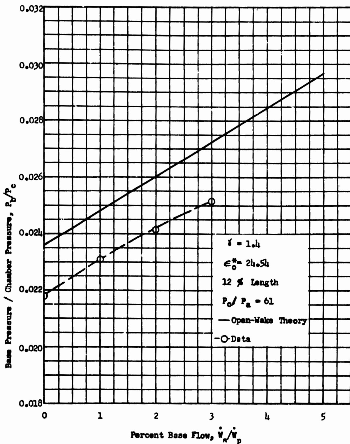
Fig. 69 Base Pressure vs Percent Base Bleed for Open-Wake Flow, Scaled Hot-Firing Model
