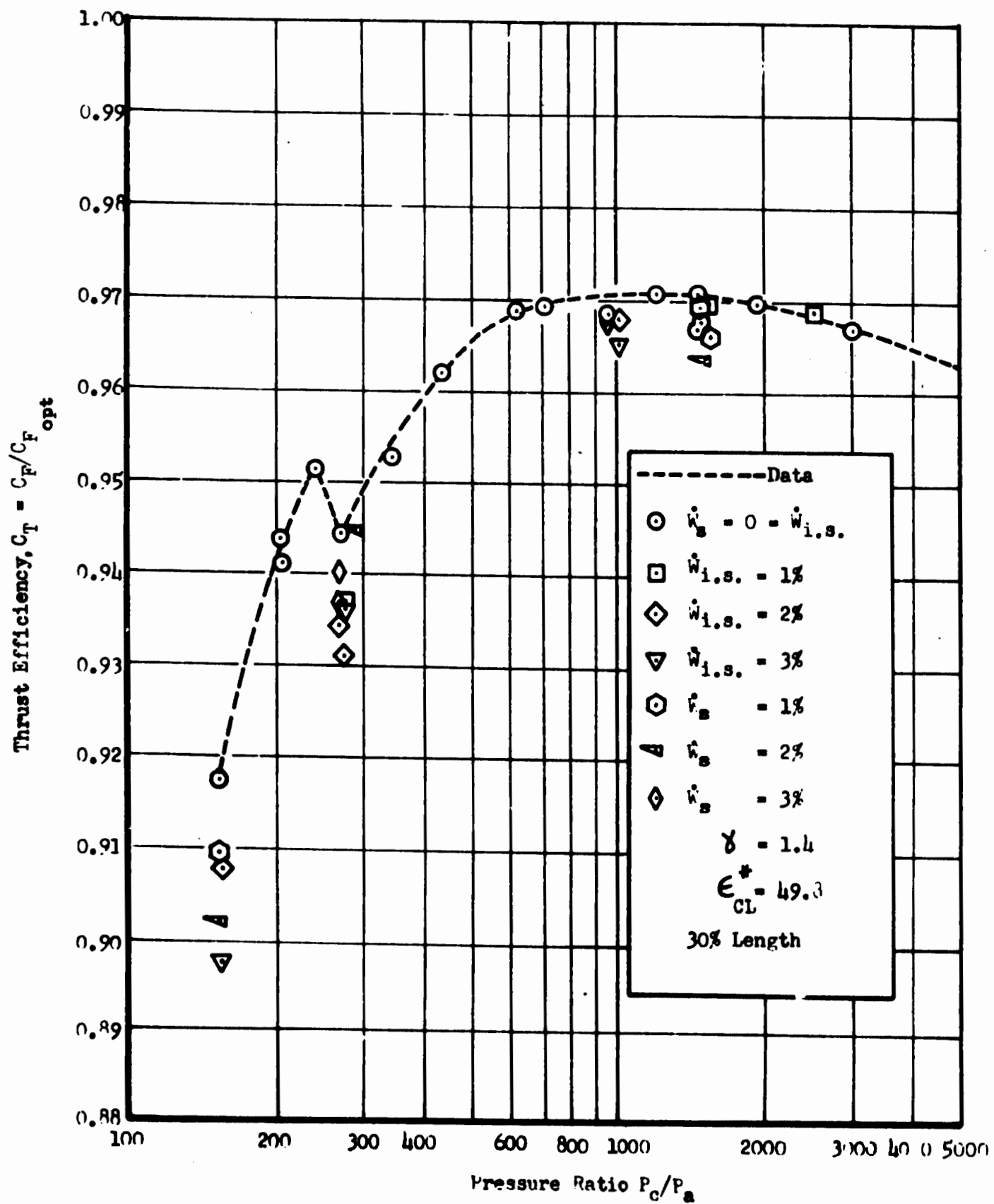
Fig. 88 Thrust Efficiency vs Pressure Ratio, 8 Modules Touching Multichamber, 30 Percent Length
