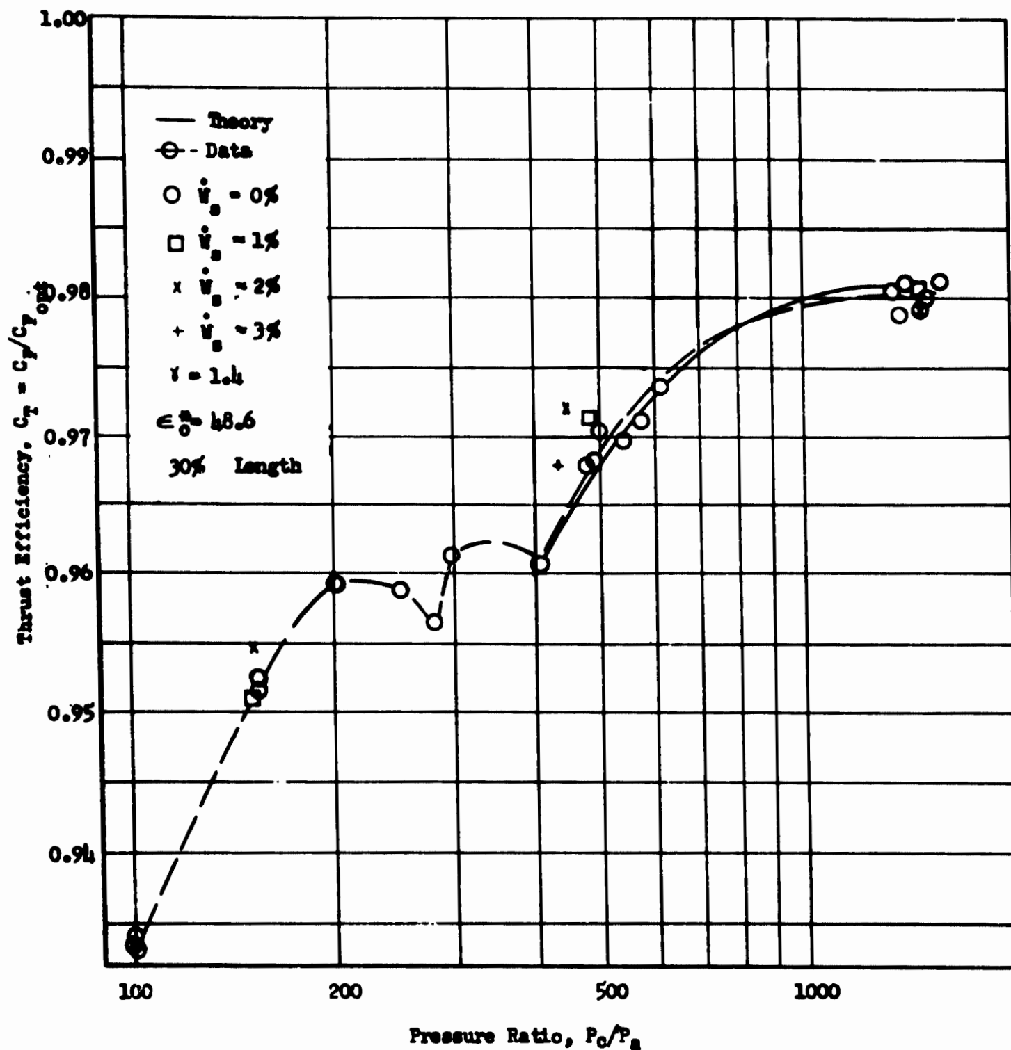
Fig. 75 Thrust Efficiency vs Pressure Ratio, Shrouded Spike Nozzle
