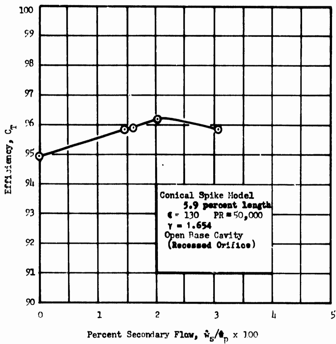
Fig. 35. Efficiency Versus Secondary Flowrate, Conical Aerodynamic Spike
