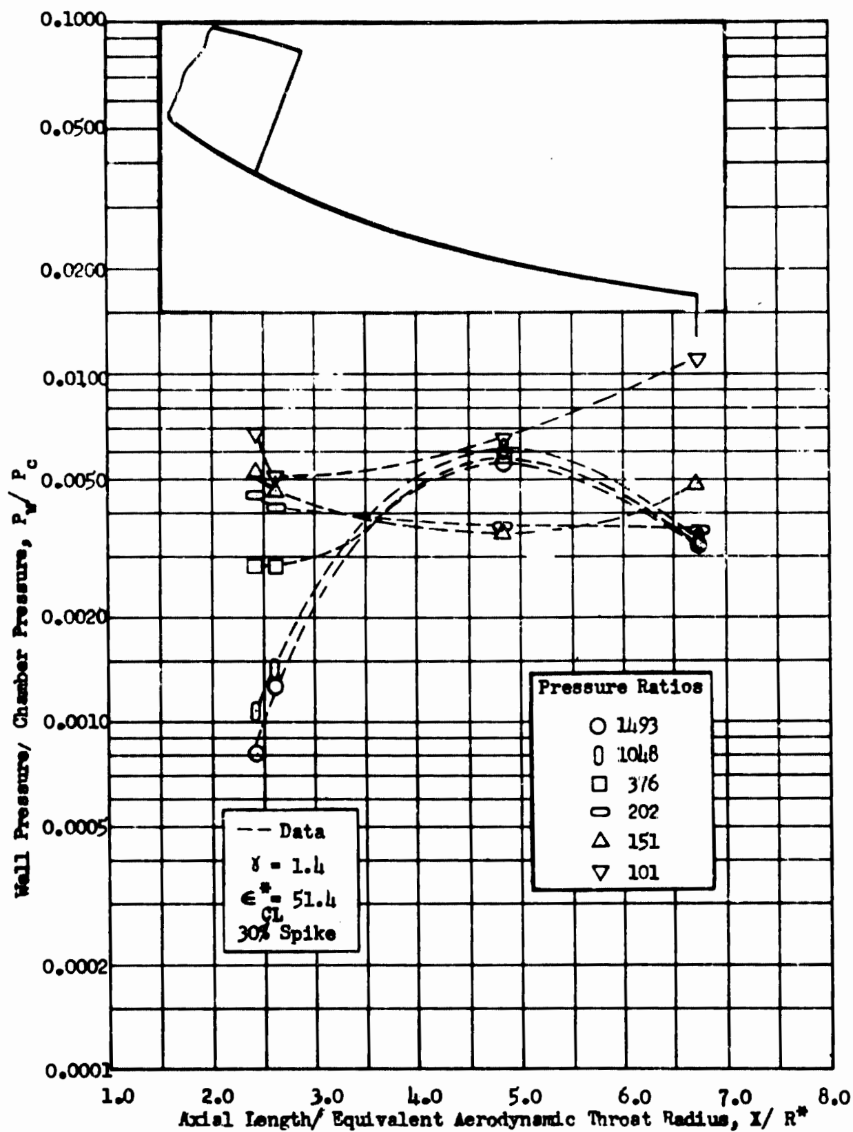
Fig. 109 Wall Pressure Between Modules vs Axial Length, 16 Module Multichamber, 30 Percent Length
