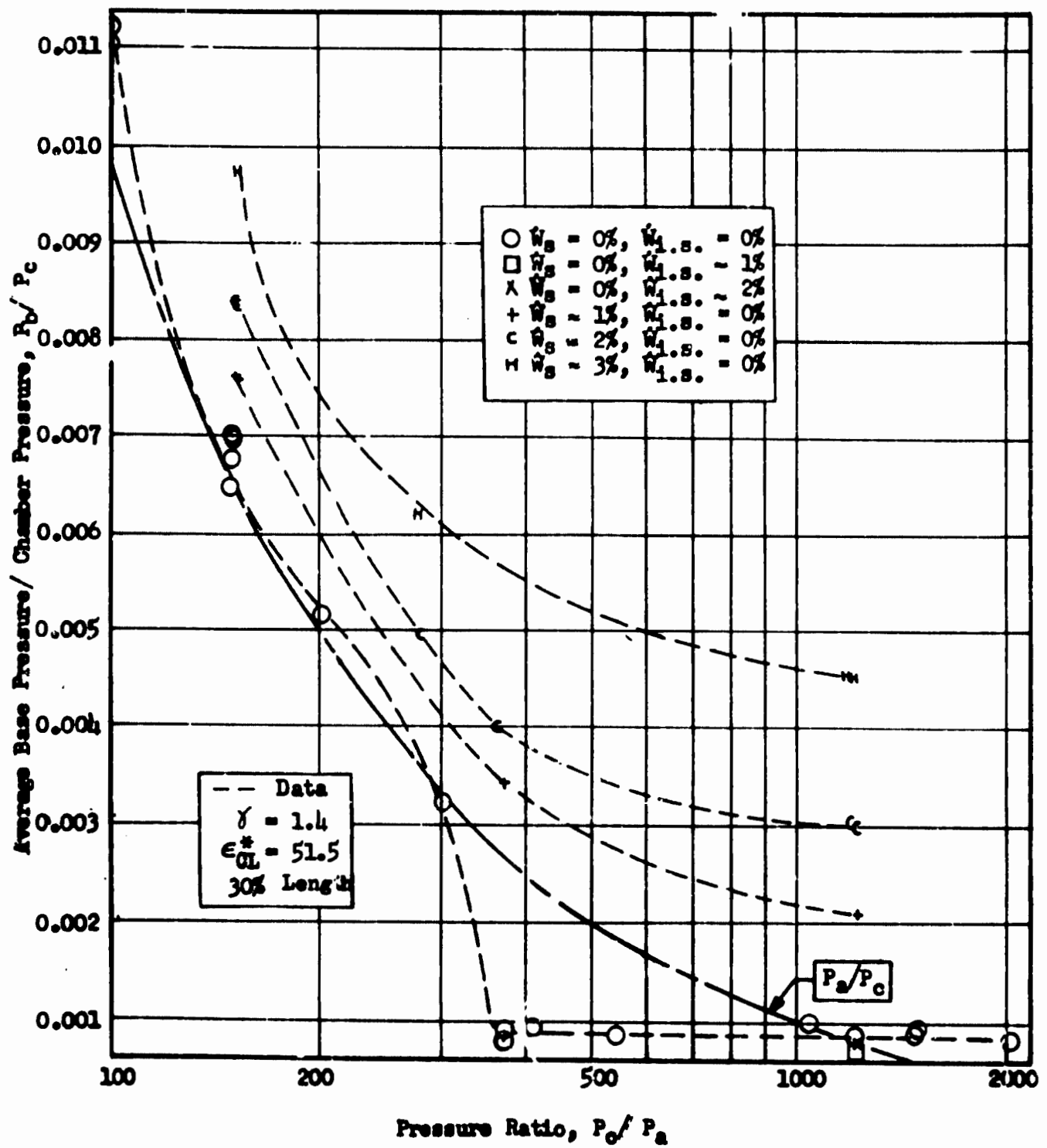
Fig.104 Base Pressure vs Pressure Ratio, 16 Module Multichamber, 30 percent Length
