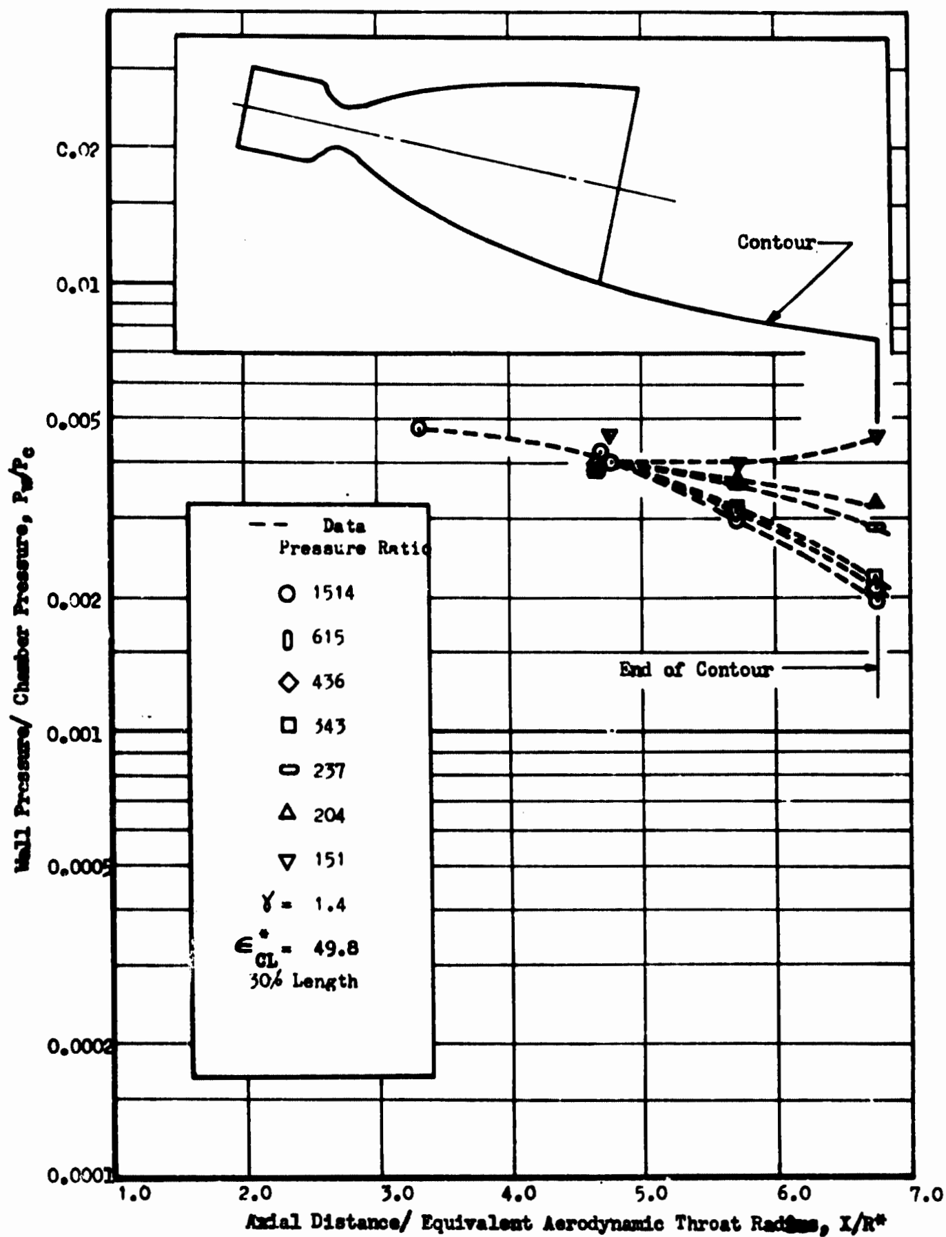
Fig. 94 Module Centerline Wall Pressures vs Axial Length, 6 Module Touching Multichamber, 50 Percent Length
