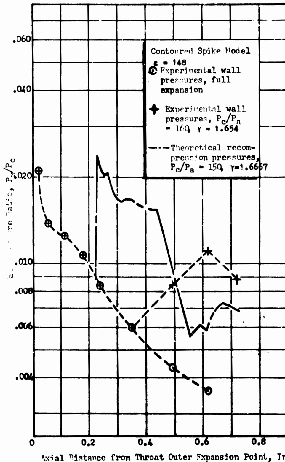
Fig. 28. Theoretical and Experimental Wall Pressures with Recompression, Contoured Spike Model
