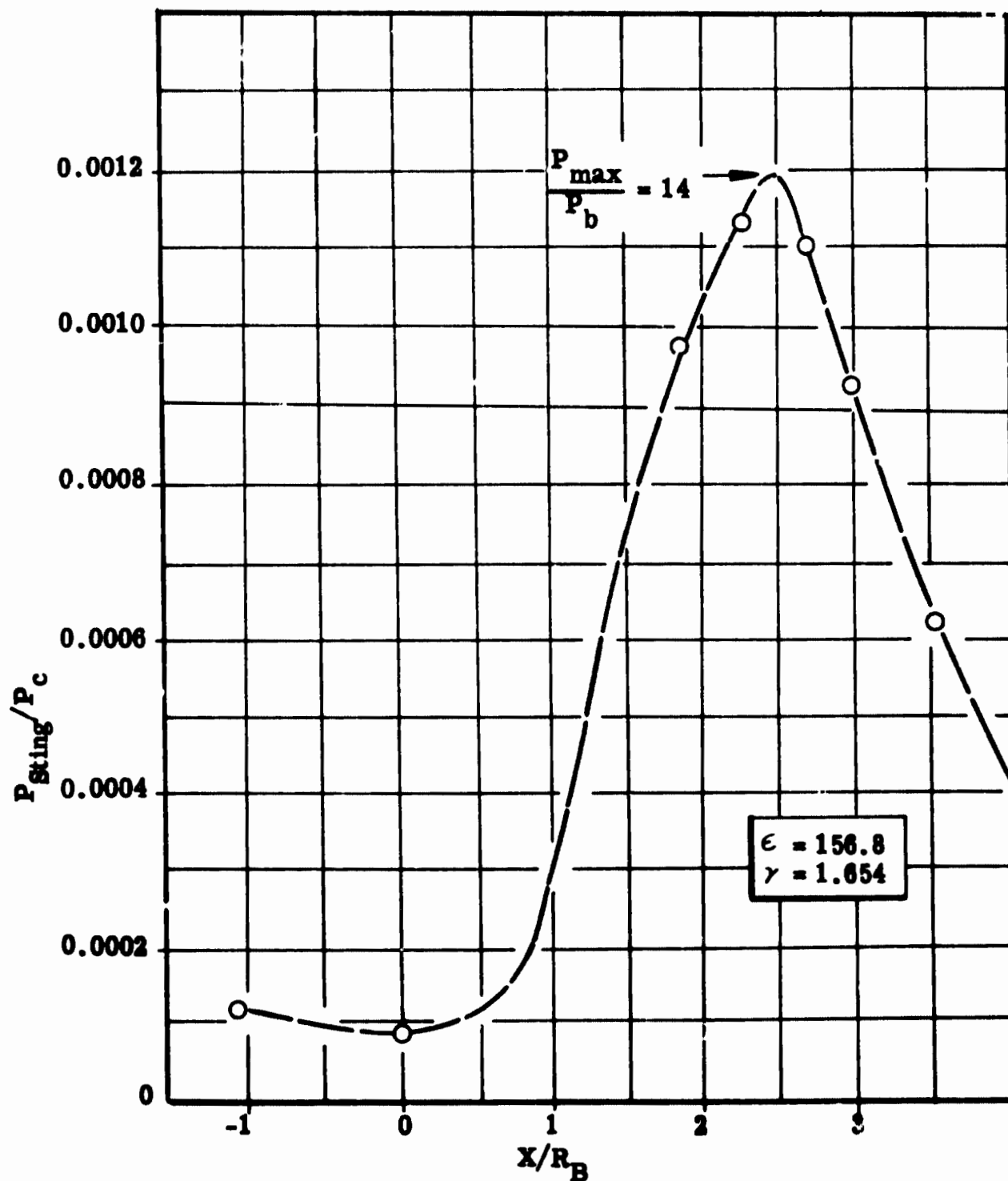
Figure 41. Centerline Wake Pressure Profile Contoured Spike Configuration, No Bleed
