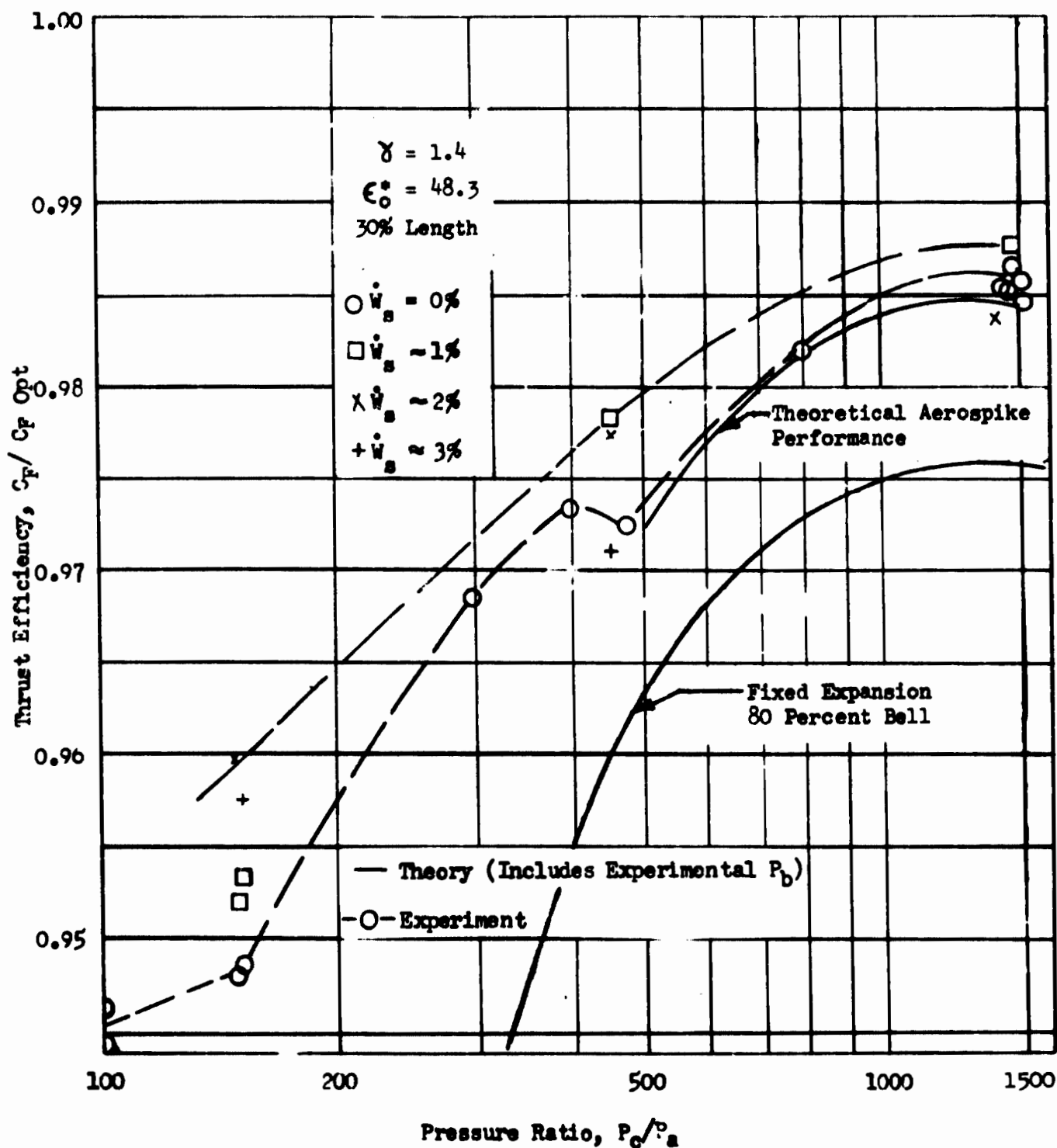
Fig. 70 Thrust Efficiency vs Pressure Ratio, Point Expansion Spike Nozzle
