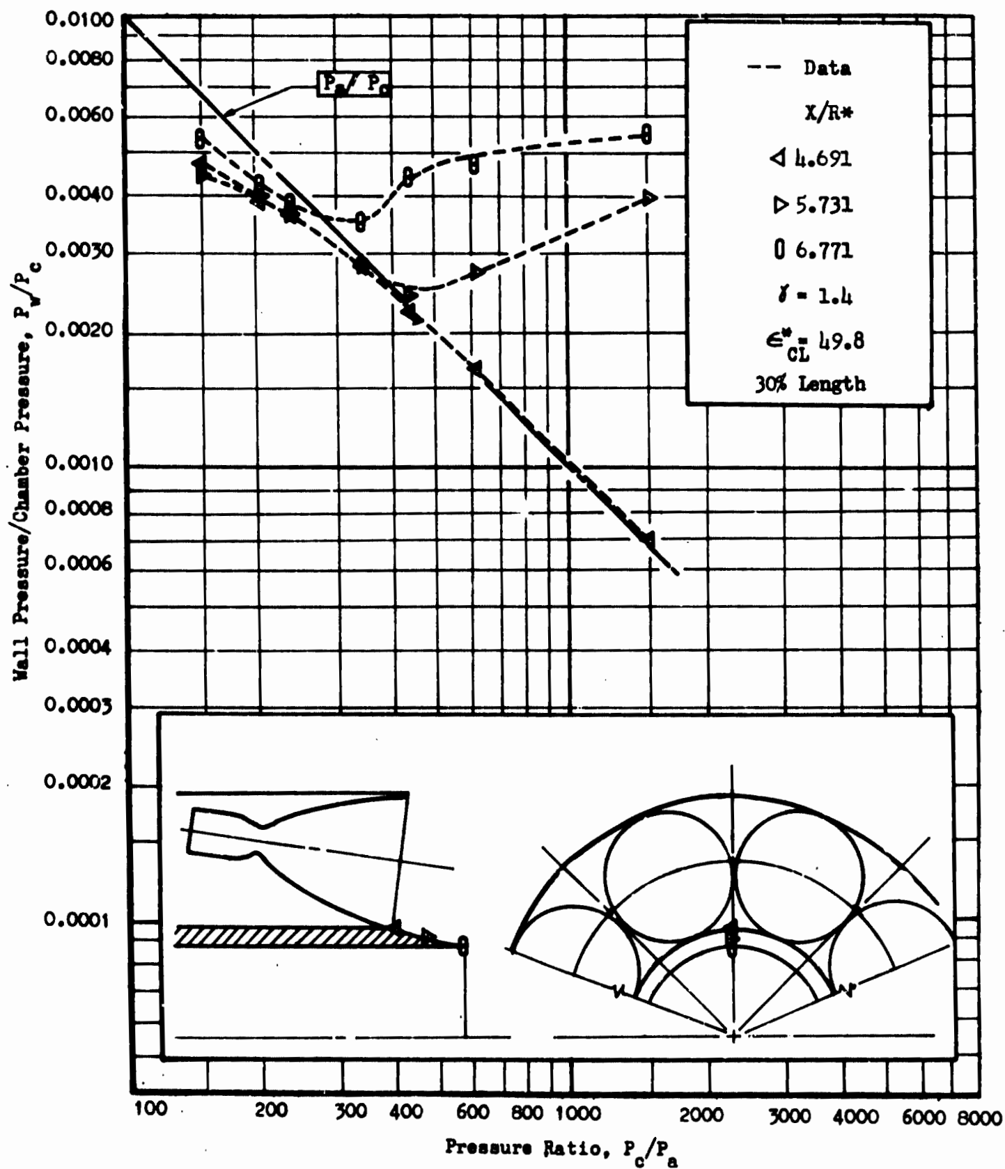
Fig. 93 Wall Pressure Between Modules vs Pressure Ratio, 8 Modules, Touching Multichamber, 30 Percent Length
