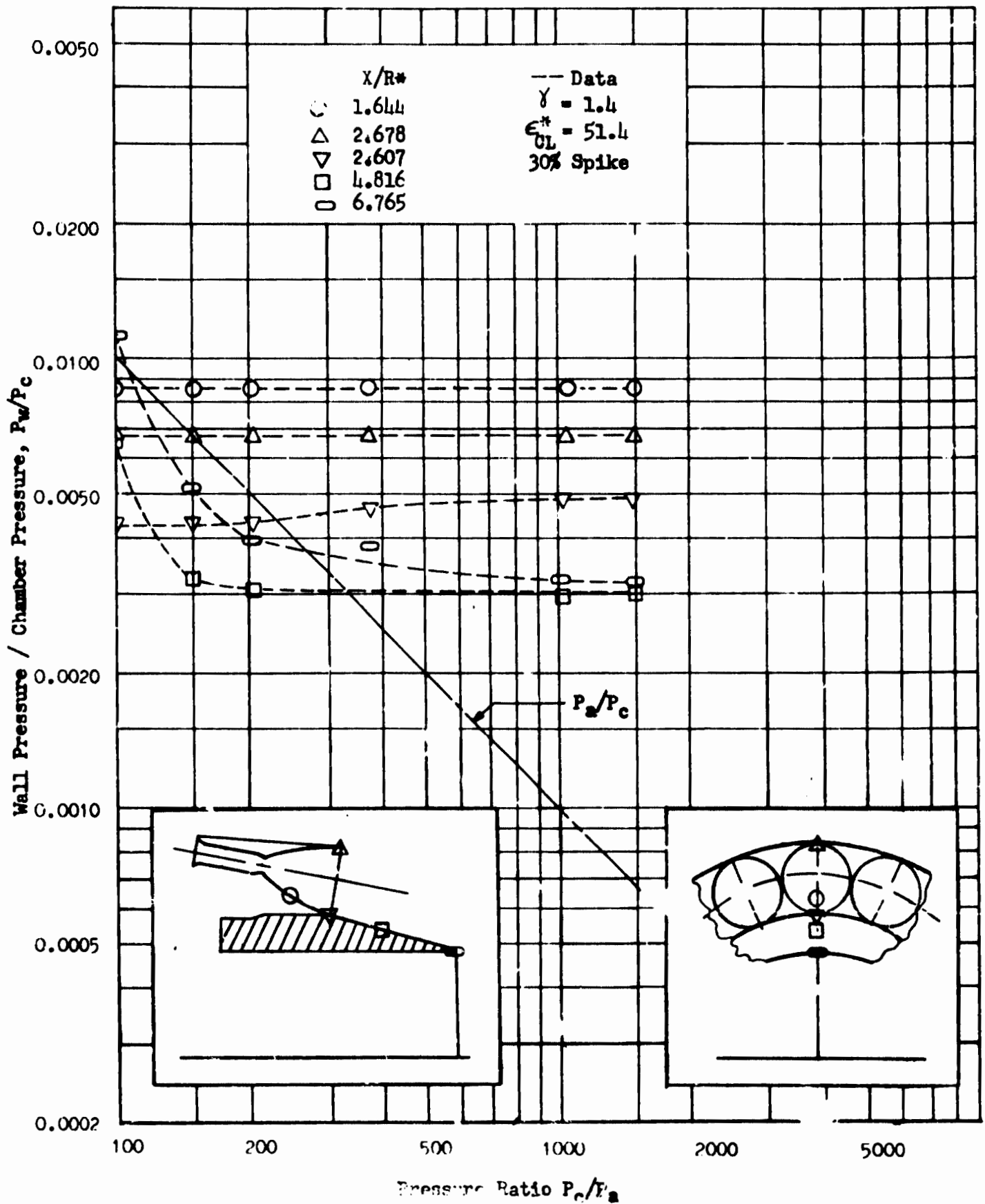
Fig. 106 Module Centerline Wall Pressure vs Pressure Ratio, 16 Module Multichamber 30 percent Length
