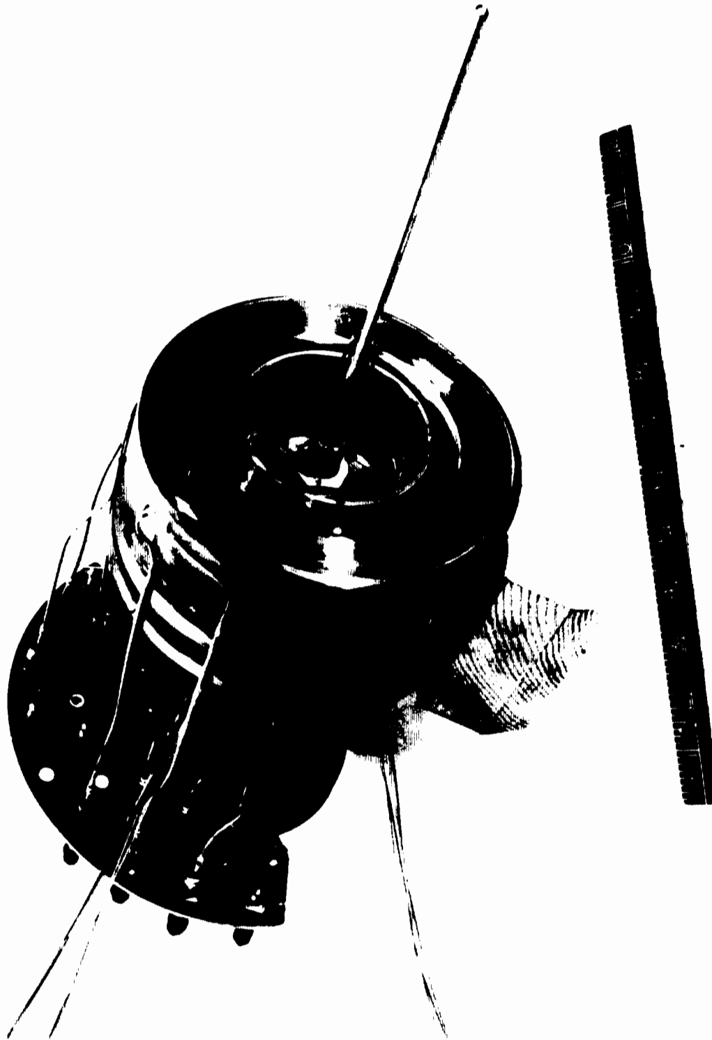
Fig. 39. Instrumented Wake Probe Mounted on the Contoured High-Area-Ratio Aerodynamic Spike Nozzle
