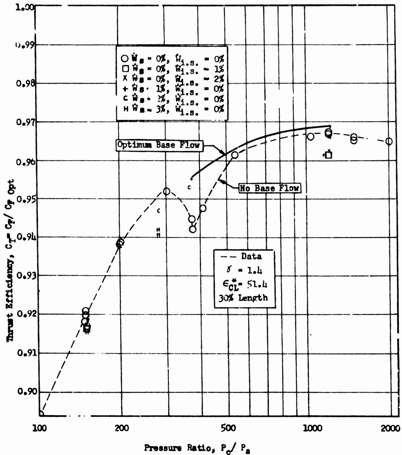
Fig. 103 Thrust Efficiency vs Pressure Ratio, 16 Module Multichamber, 30 percent Length
