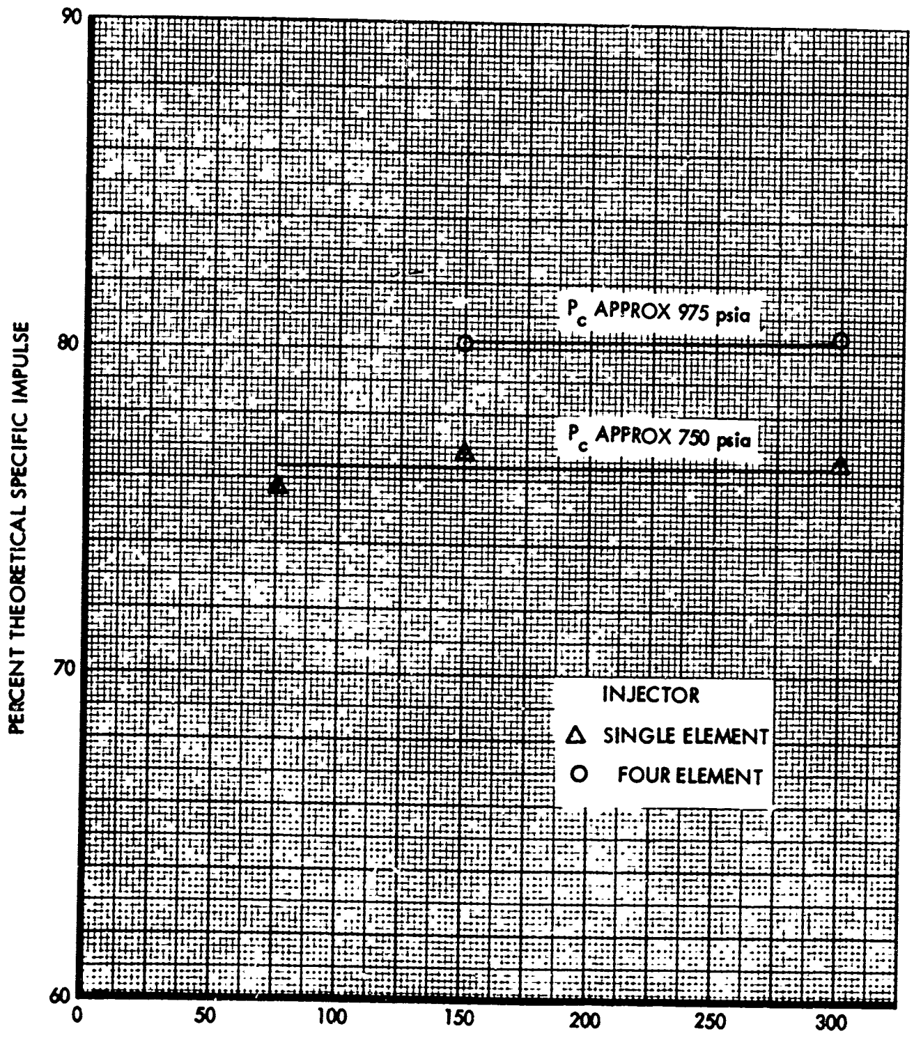
FIGURE 9 CHARACTERISTIC LENGTH, L^* (in)
