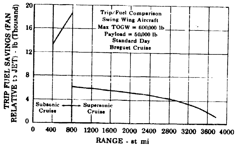
Figure 9. Trip/Fuel Comparison
