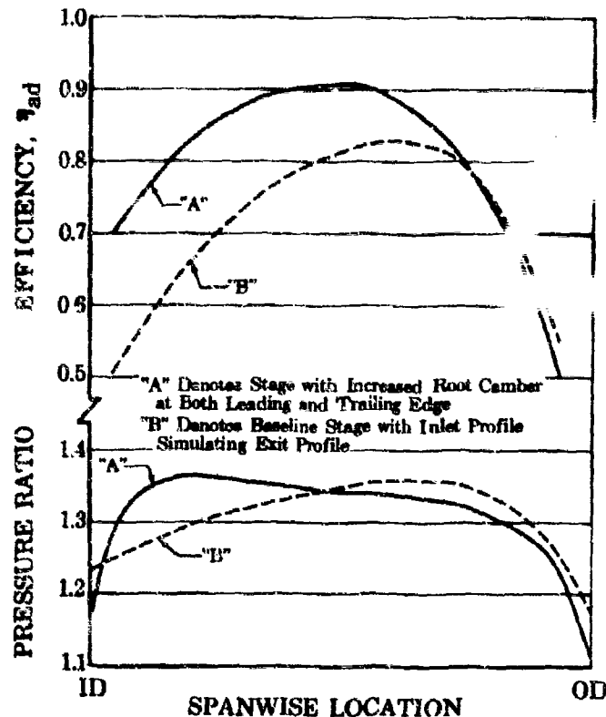
Figure 24. Single Stage Tests of Simulated JTF17 HPC Stage
