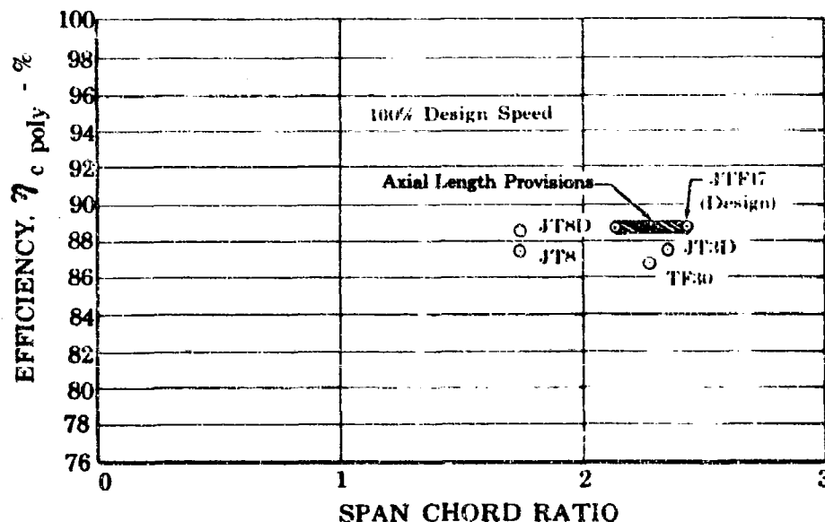
Figure 19. Polytypic Efficiency vs Span Chord Ratio for High Pressure Compressors
