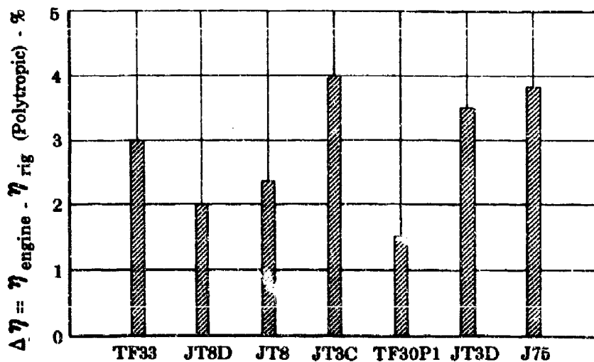
Figure 26. Difference Between Engine and Rig Efficiency
