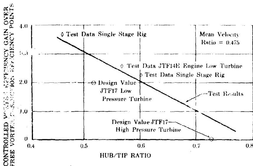
Figure 14. Efficiency Gains of Controlled Vortex Test Turbines Over Free Vortex Predictions FD 17531 ATIIC
