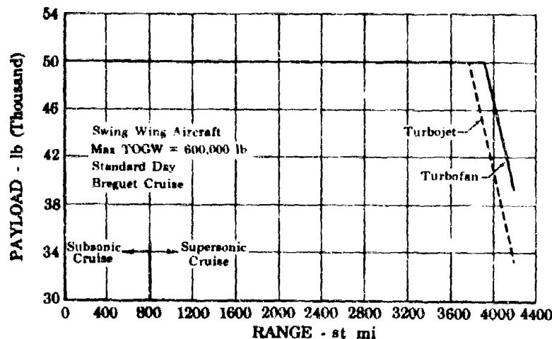
Figure 10. Range/Payload Comparison
