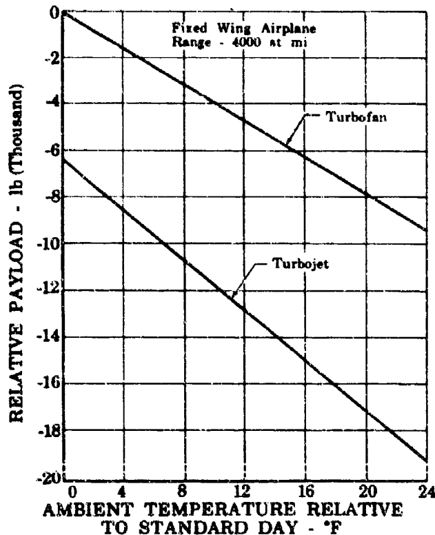
Figure 17. Cruise Ambient Temperature Effect on Payload - Fixed-Wing Aircraft
