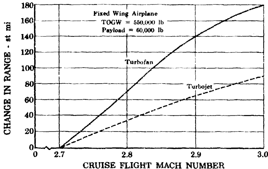
Figure 22. Cruise Mach No. Effect on Design Range
