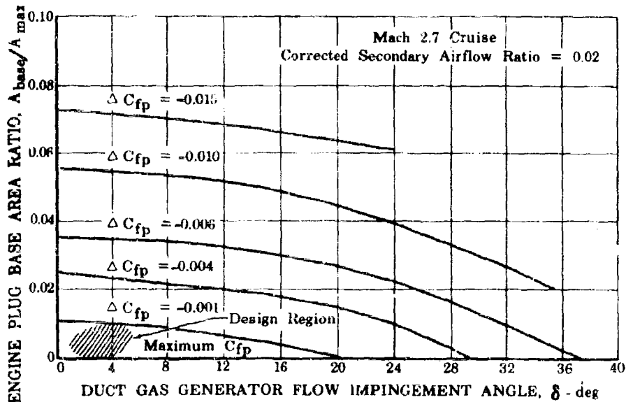
Figure 27. Typical Variation of Exhaust System Performance With Engine Plug Base Area
