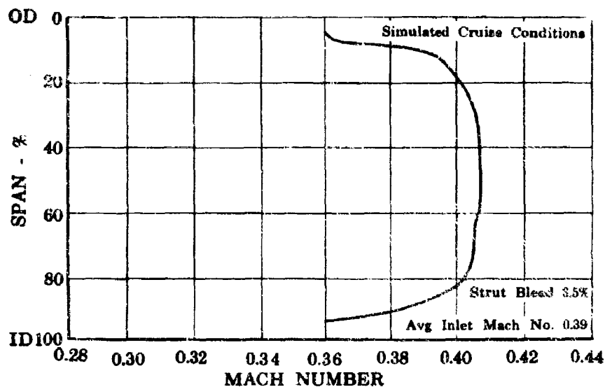
Figure 17. 120-deg Sector Rig Inlet Airflow Profile
