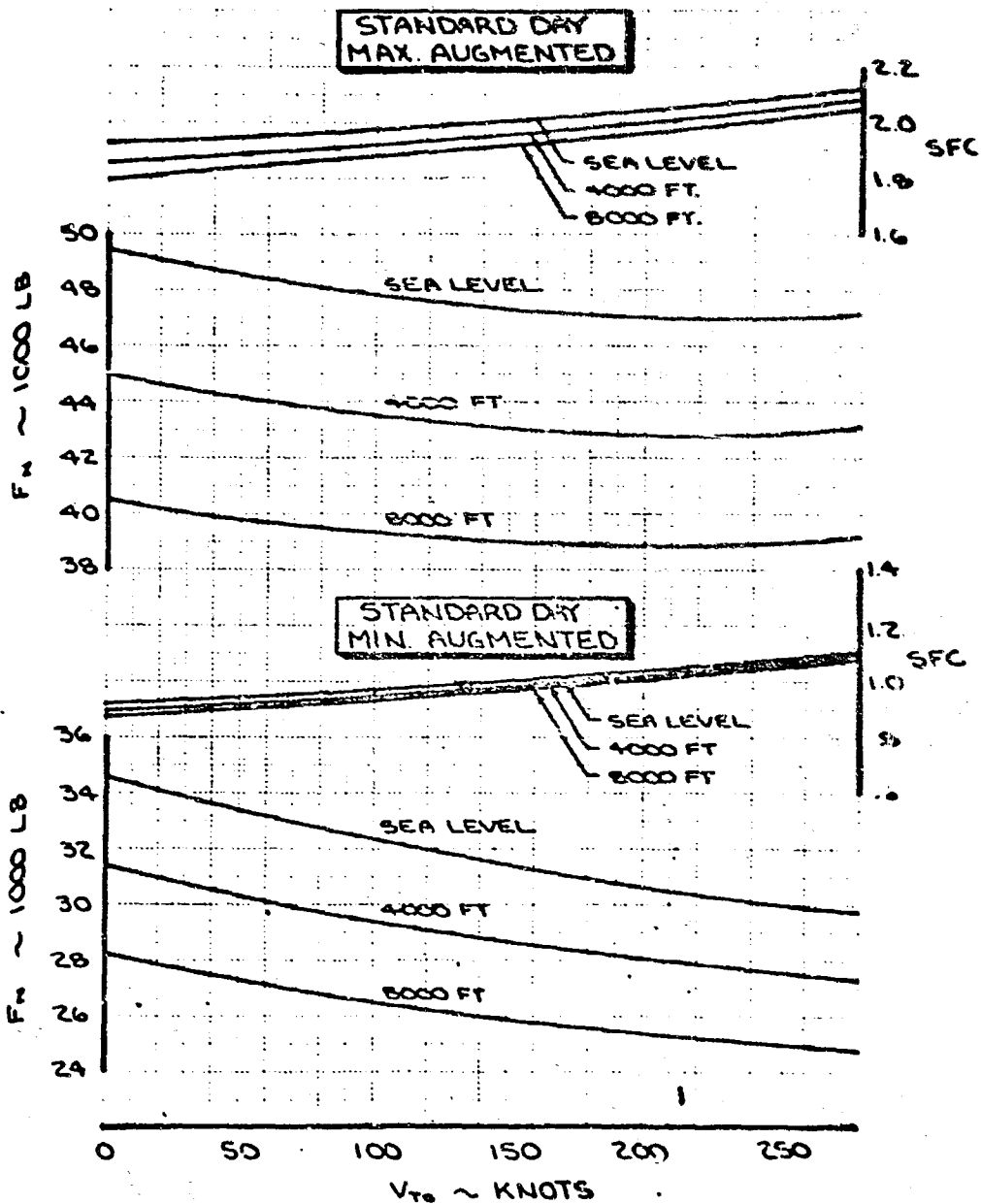
Fig. 4 Takeoff Thrust and SFC - Standard Day
