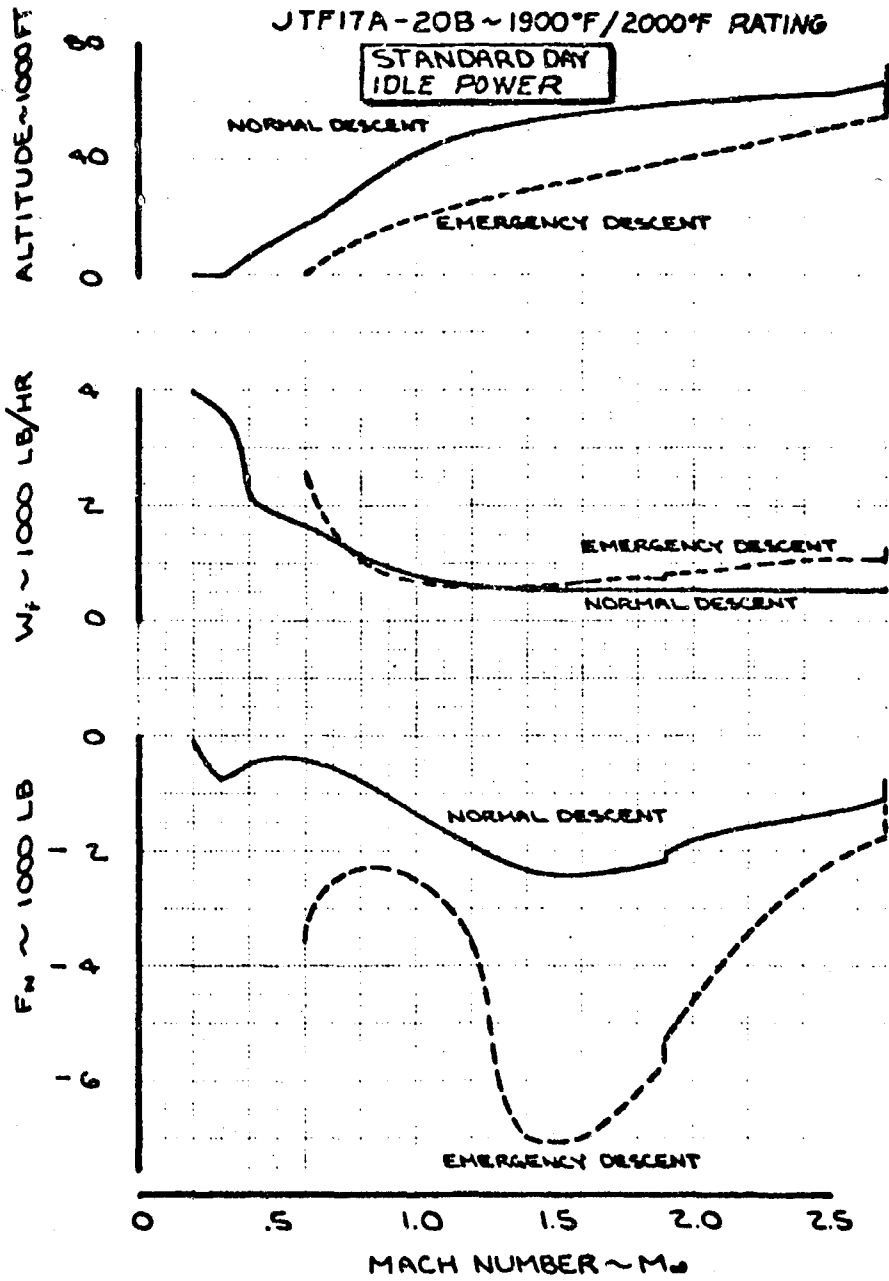
Fig. 16 Normal and Emergency Descent - Thrust and Fuel Flow - Standard Day
