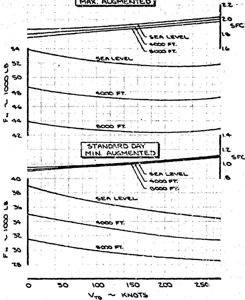
Fig. A-1 Takeoff Net Thrust and SFC - Standard Day
