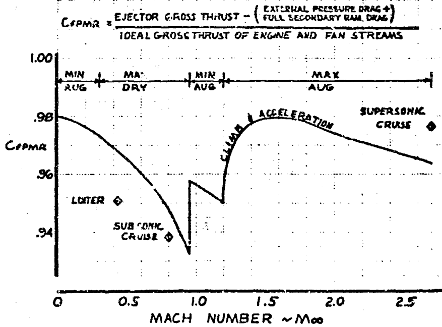
Fig. 2 Thrust Coefficient
