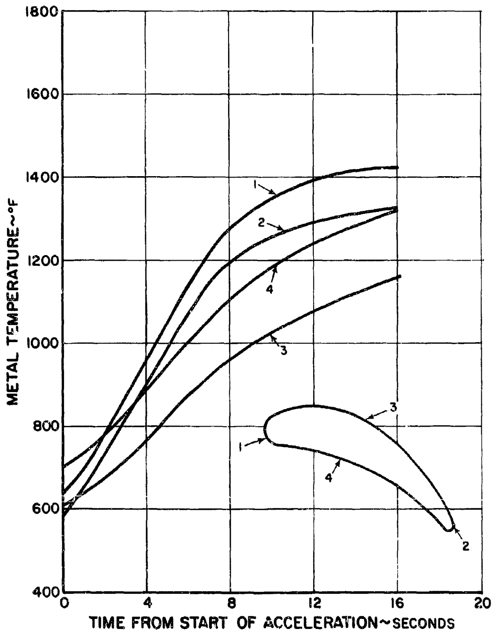
CONVECTIVELY COOLED FIRST TURBINE BLADE - TRANSIENT RESPONSE
