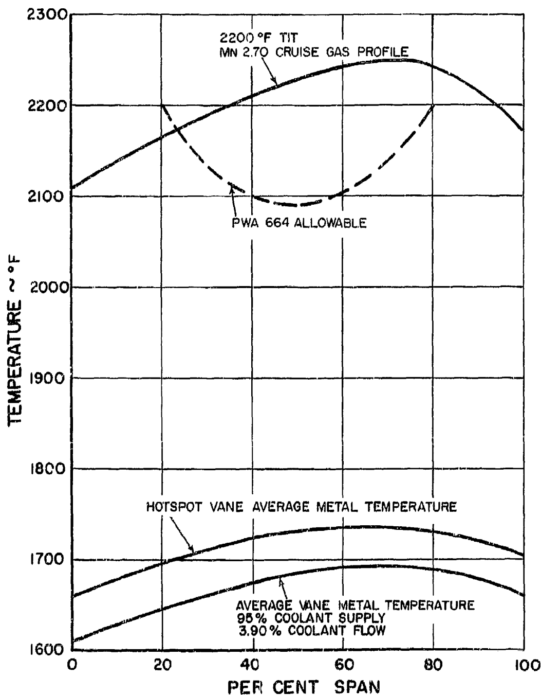
AVERAGE VANE TEMPERATURE
