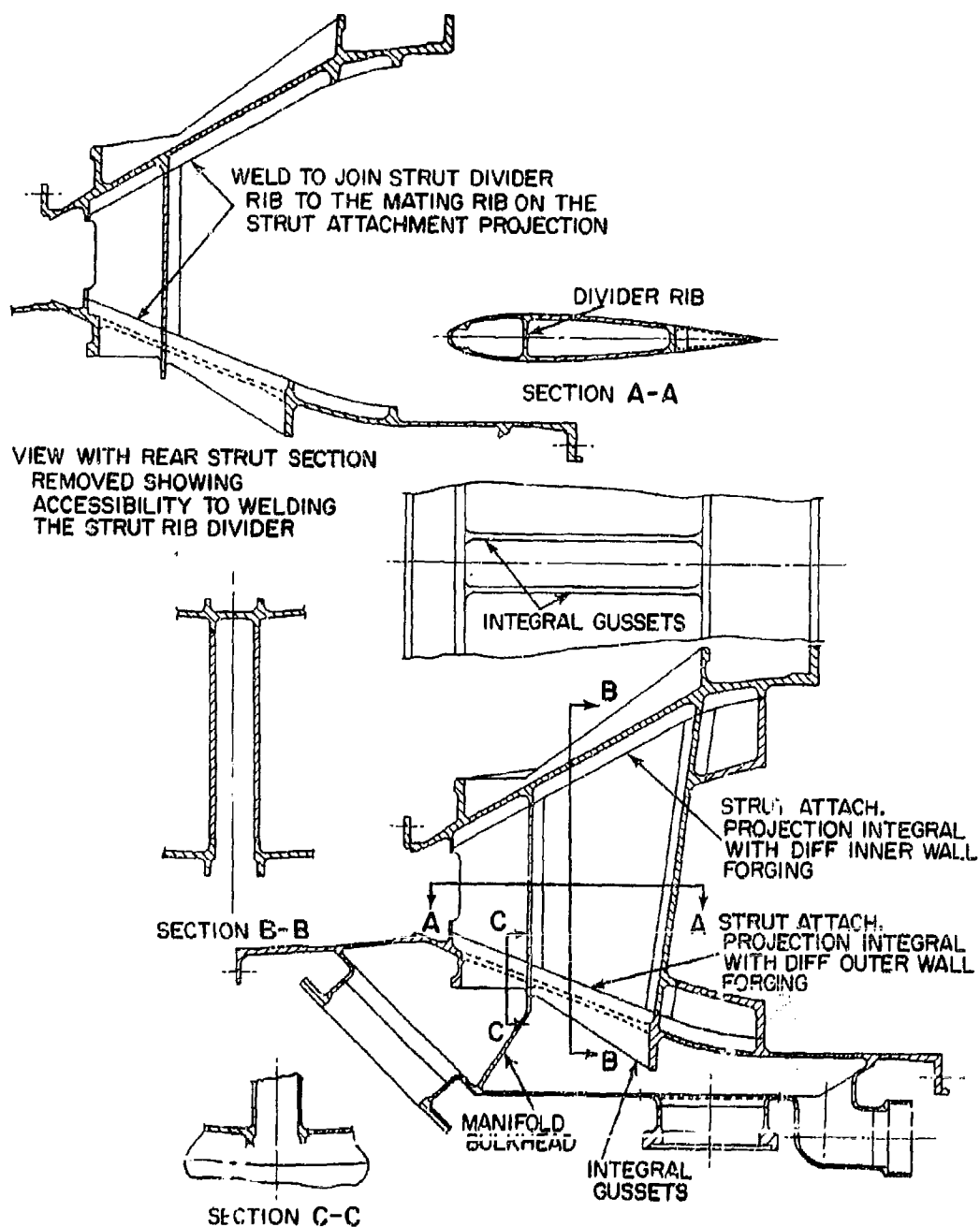
STP219 DIFFUSER CASE FABRICATION TECHNIQUES CONSIDERED IN EARLY DESIGN STUDIES
