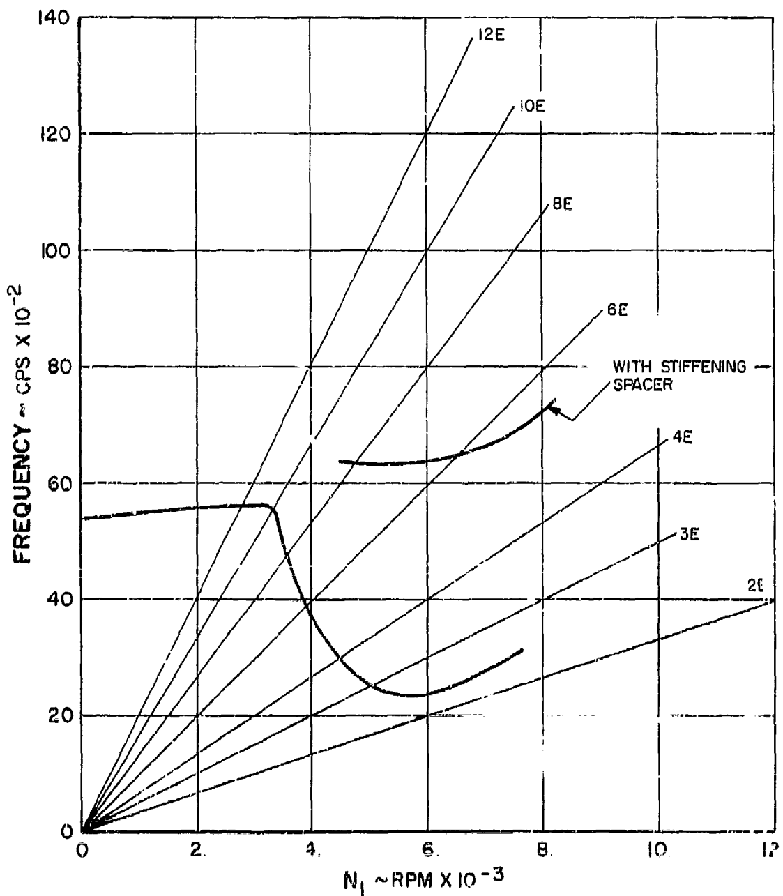
STP219 THIRD STAGE DISK BLADE COUPLED FREQUENCIES
