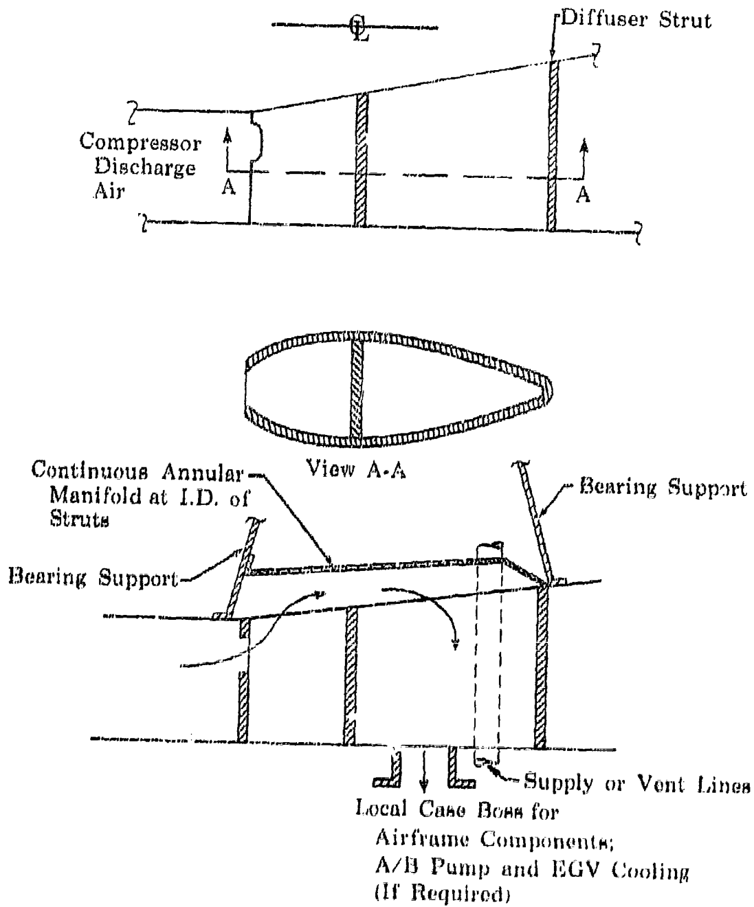
AIRFRAME BLEED FLOW REQUIREMENTS
