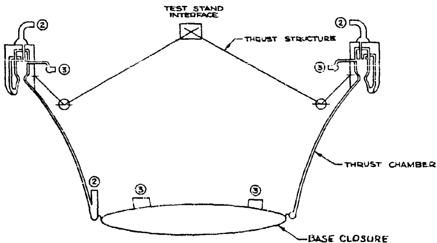
①-THRUST SUBSYSTEM
