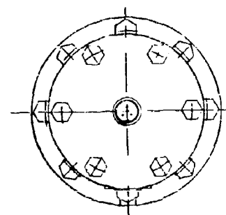
VIEW B-B (SCALE 1/1)
