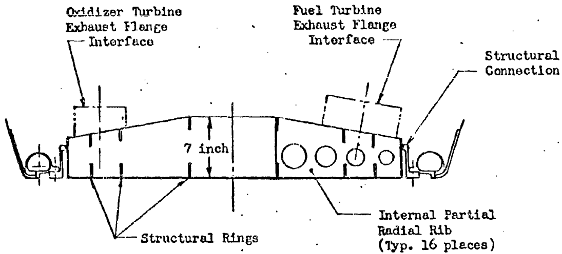
Figure 32. Flat Plate Base Closure
