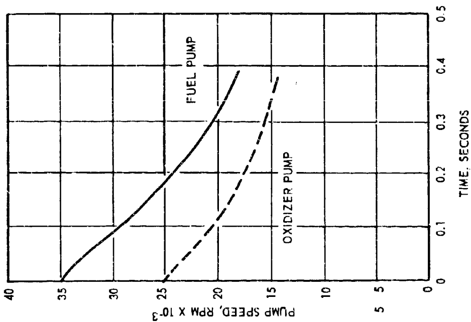
Figure 14. Pump Speed Cutoff Decay
