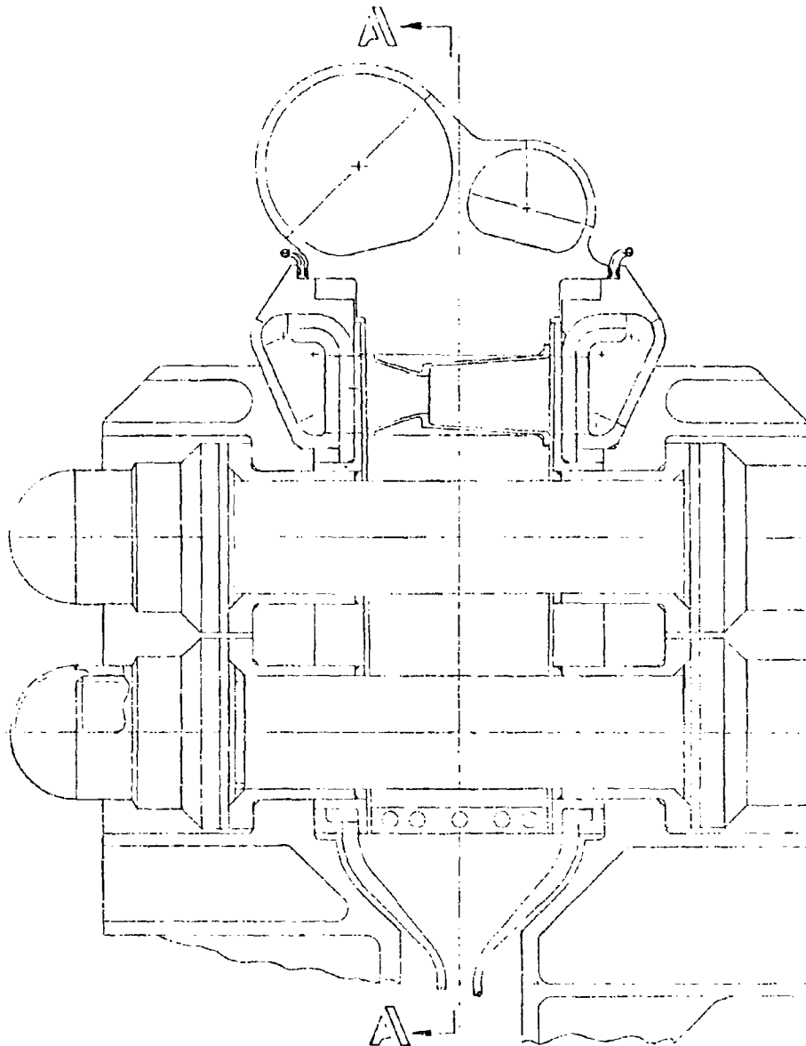
Figure 31. Integral Baffle Injector
