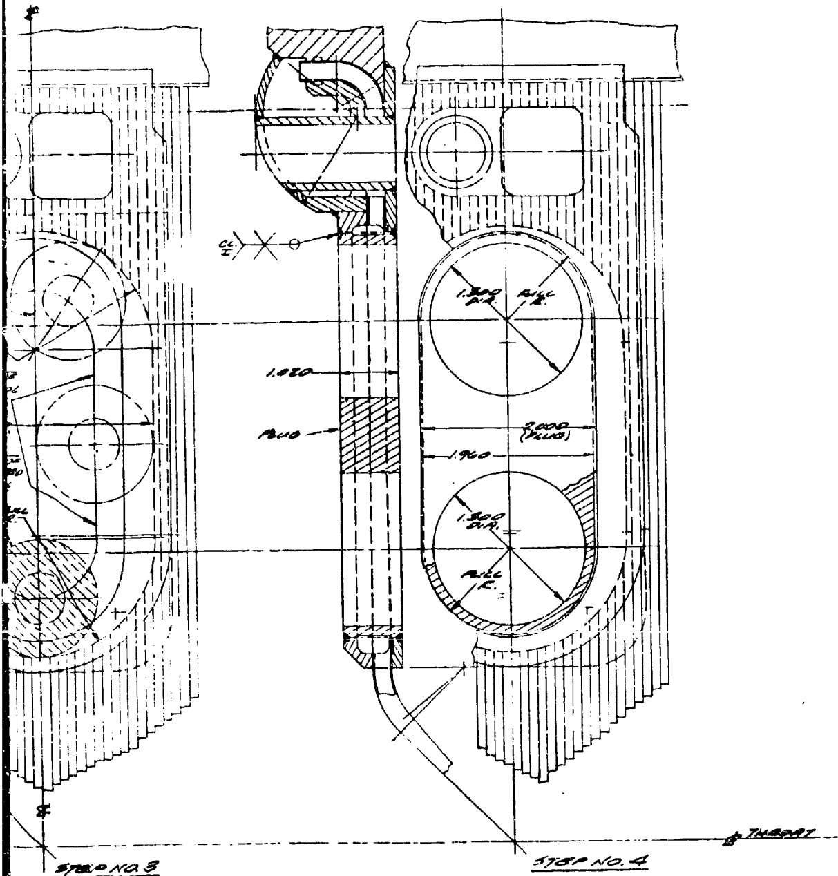
Figure 28. Step Method of Installing and Machining Baffle Seat
